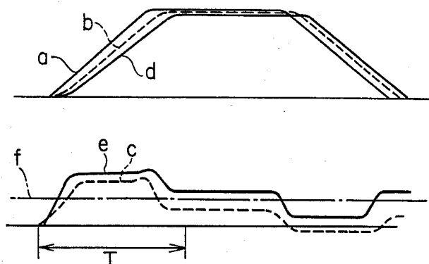
FIG. 4 (PRIOR ART)
