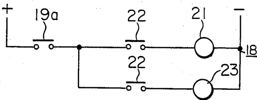
FIG. 5 (PRIOR ART)
