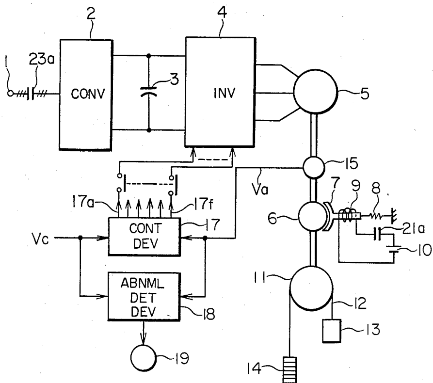
FIG. 4 (PRIOR ART)
