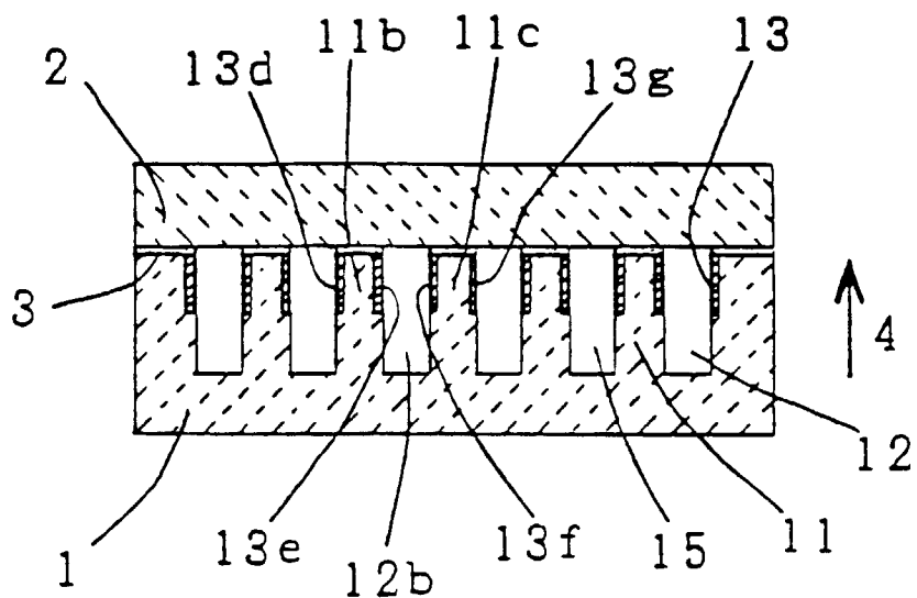
Fig.15 PRIOR ART
