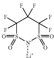
[Chemical Formulas 6]
