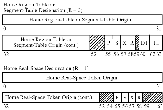
Format of Control Register 13
