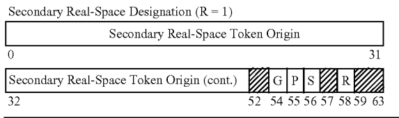
Format of Control Register 7
