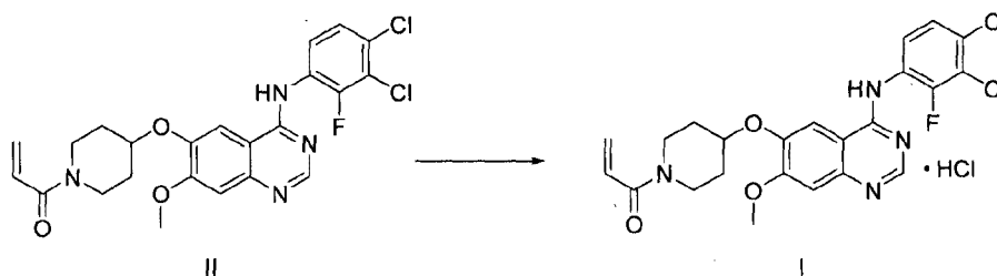
<Reaction Scheme 6>
