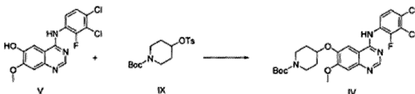
<Reaction Scheme 3>
