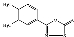
5-(3,4-Dimethyl-phenyl)-[1,3,4]oxathiazol-2-one
