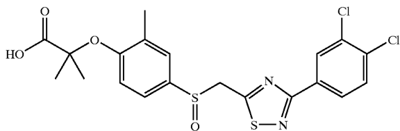
2-{4-[3-(3,4-Dichloro-phenyl)-[1,2,4]thiadiazol-5-ylmethanesulfinyl]-2-methyl-phenoxy}-2-methyl-propionic acid
