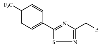
3-Bromomethyl-5-(4-trifluoromethyl-phenyl)-[1,2,4]thiadiazole
