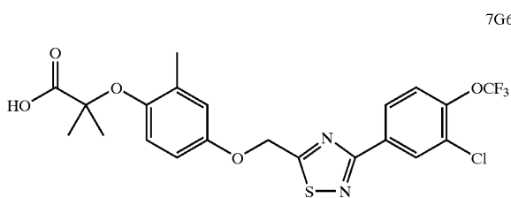
2-Methyl-2-{2-methyl-4-[3-(4-trifluoromethoxy-phenyl)-[1,2,4]thiadiazol-5-ylmethoxy]-phenoxy}-propionic acid
