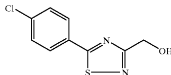
[5-(4-Chloro-phenyl)-[1,2,4]thiadiazol-3-yl]-methanol
