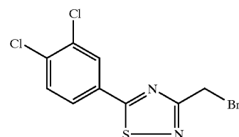
3-Bromomethyl-5-(3,4-dichloro-phenyl)-[1,2,4]thiadiazole
