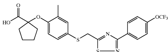
1-{2-Methyl-4-[3-(4-trifluoromethoxy-phenyl)-[1,2,4]thiadiazol-5-ylmethylsulfanyl]-phenoxy}-cyclopentanecarboxylic acid
