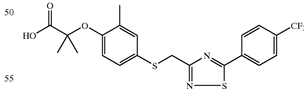
2-Methyl-2-[2-methyl-4-[5-(4-trifluoromethyl-phenyl)-[1,2,4]thiadiazol-3-ylmethylsulfanyl]-phenoxy]-propionic acid
