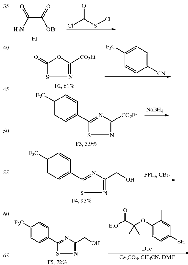
Scheme F
