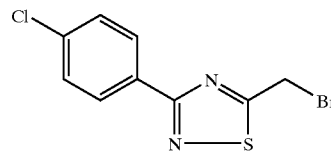
5-Bromomethyl-3-(4-chloro-phenyl)-[1,2,4]thiadiazole
