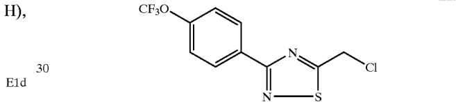
5-Chloromethyl-3-(4-trifluoromethoxy-phenyl)-[1,2,4]thiadiazole
