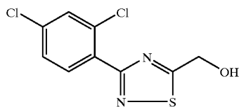
[3-(2,4-Dichloro-phenyl)- [1,2,4]thiadiazol-5-yl]-methanol
