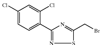
5-Bromomethyl-3- (2,4-dichloro-phenyl)-[1,2,4]thiadiazole
