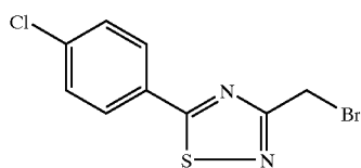
3-Bromomethyl-5-(4-chloro-phenyl)-[1,2,4]thiadiazole
