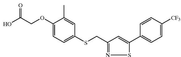
{2-Methyl-4-[5-(4-trifluoromethyl-phenyl)-isothiazol-3-ylmethylsulfanyl]-phenoxy}-acetic acid
