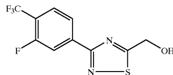
[3-(3-Fluoro-4-trifluoromethyl-phenyl)-[1,2,4]thiadiazol-5-yl]-methanol
