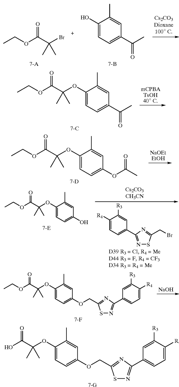
Scheme 7. Synthesis of Compound 7-G
