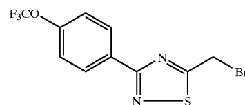
5-Bromomethyl-3-(4-(trifluoromethoxy)-phenyl)-[1,2,4]thiadiazole
