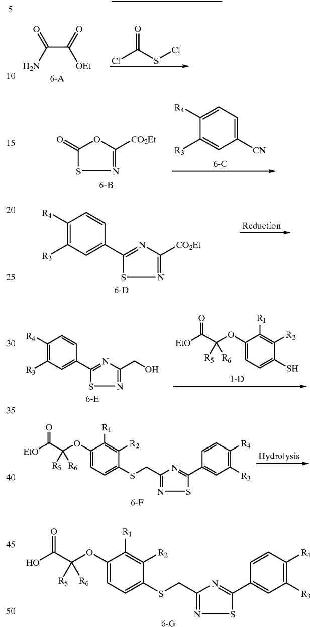
Scheme 6. Synthesis of Compound 6-G
