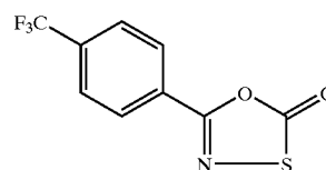
5-(4-Trifluoromethyl-phenyl)-[1,3,4]oxathiazol-2-one
