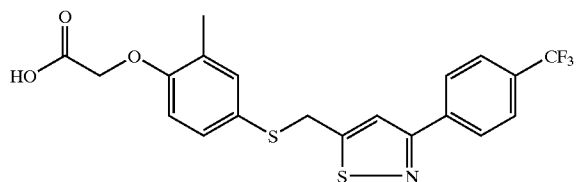
{2-Methyl-4-[3-(4-trifluoromethyl-phenyl)-isothiazol-5-ylmethylsulfanyl]-phenoxy}-acetic acid
