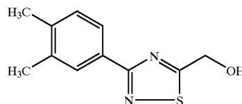
[3-(3,4-Dimethyl-phenyl)- [1,2,4]thiadiazol-5-yl]-methanol
