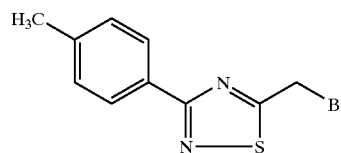
5-Bromomethyl-3-p-tolyl-[1,2,4]thiadiazole
