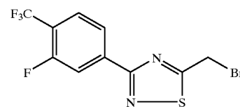
5-Bromomethyl-3-(3-fluoro-4-trifluoromethyl-phenyl)-[1,2,4]thiadiazole
