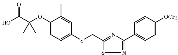
2-Methyl-2-{2-methyl-4-[3-(4-trifluoromethoxyphenyl)-[1,2,4]thiadiazol-5-ylmethylsulfanyl]-phenoxy}-propionic acid
