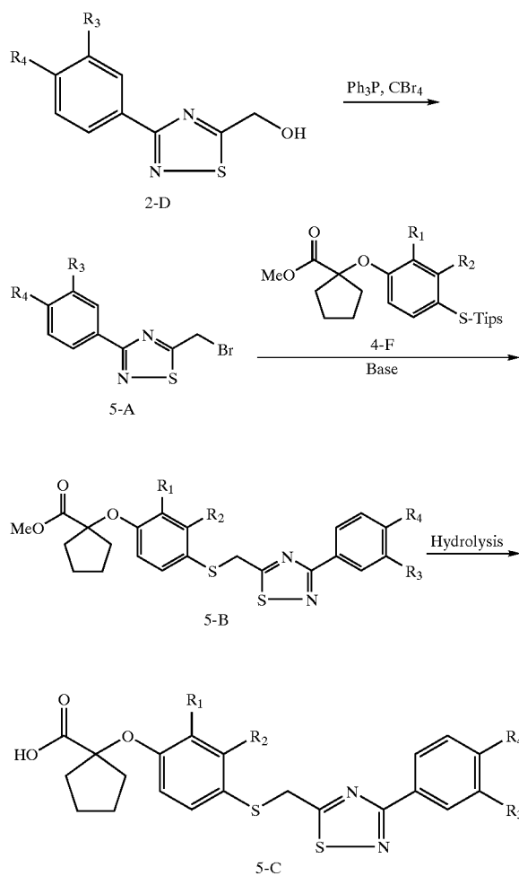
Scheme 5. Synthesis of Compound 5-C
