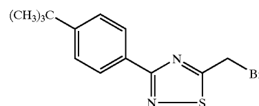
5-Bromomethyl-3-(4-tert-butyl-phenyl)-[1,2,4]thiadiazole
