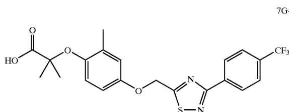
2-Methyl-2-{2-methyl-4-[3-(4-trifluoromethyl-phenyl)-[1,2,4]thiadiazol-5-ylmethoxy]-phenoxy}-propionic acid
