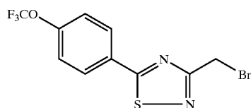
3-Bromomethyl-5-(4-trifluoromethoxy-phenyl)-[1,2,4]thiadiazole
