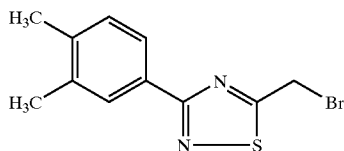
5-Bromomethyl-3-(3,4-dimethyl-phenyl)-[1,2,4]thiadiazole
