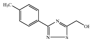
(3-p-Tolyl-[1,2,4]thiadiazol-5-yl)-methanol
