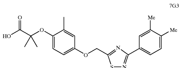
2-{4-[3-(3,4-Dimethyl-phenyl)-[1,2,4]thiadiazol-5-ylmethoxy]-2-methyl-phenoxy}-2-methyl-propionic acid
