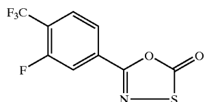
5-(3-Fluoro-4-trifluoromethyl-phenyl)-[1,3,4]oxathiazol-2-one
