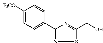
[3-(4-Trifluoromethoxy-phenyl)-[1,2,4]thiadiazol-5-yl]-methanol
