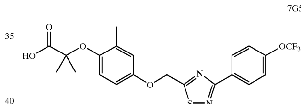
2-Methyl-2-{2-methyl-4-[3-(4-trifluoromethoxy-phenyl)-[1,2,4]thiadiazol-5-ylmethoxy]-phenoxy}-propionic acid
