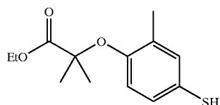
2-(4-Mercapto-2-methyl-phenoxy)-2-methyl-propionic acid ethyl ester
