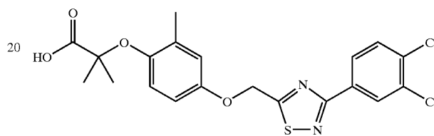
2-{4-[3-(3,4-Dichloro-phenyl)-[1,2,4]thiadiazol-5-ylmethoxy]-2-methyl-phenoxy}-2-methyl-propionic acid
