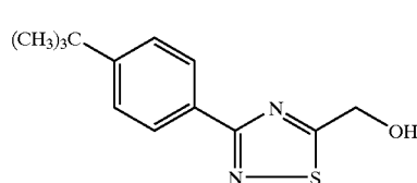
[3-(4-tert-Butyl-phenyl)-[1,2,4]thiadiazol-5-yl]-methanol
