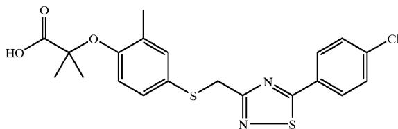
2-{4-[5-(4-Chloro-phenyl)-[1,2,4]thiadiazol-3-ylmethylsulfanyl]-2-methyl-phenoxy}-2-methyl-propionic acid
