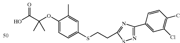
2-(4-{2-[3-(3,4-Dichloro-phenyl)-[1,2,4]thiadiazol-5-yl]-ethylsulfanyl}-2-methyl-phenoxy)-2-methyl-propionic acid
