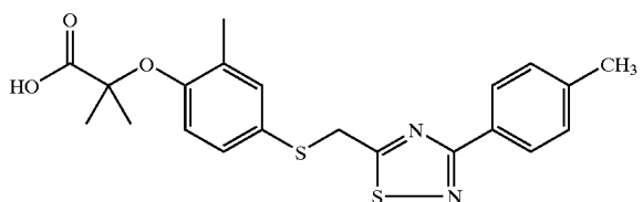
2-Methyl-2-[2-methyl-4-(3-p-tolyl-[1,2,4]thiadiazol-5-ylmethylsulfanyl)-phenoxy]-propionic acid
