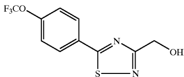
[5-(4-Trifluoromethoxy-phenyl)-[1,2,4]thiadiazol-3-yl]-methanol
