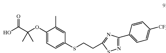
2-Methyl-2-(2-methyl-4-{2-[3-(4-trifluoromethyl-phenyl)-[1,2,4]thiadiazol-5-yl]-ethylsulfanyl}-phenoxy)-propionic acid
