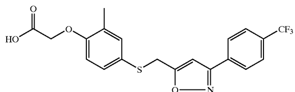
{2-Methyl-4-[3-(4-trifluoromethyl-phenyl)-isoxazol-5-ylmethylsulfanyl]-phenoxy}-acetic acid
