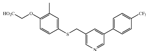
{2-Methyl-4-[5-(4-trifluoromethyl-phenyl)-pyridin-3-ylmethylsulfanyl]-phenoxy}-acetic acid
