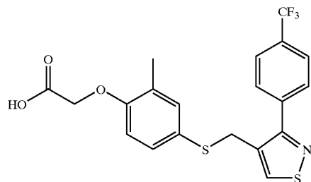
{2-Methyl-4-[3-(4-trifluoromethyl-phenyl)-isothiazol-4-ylmethylsulfanyl]-phenoxy}-acetic acid
