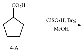
Scheme 4. Synthesis of Intermediate 4-F
