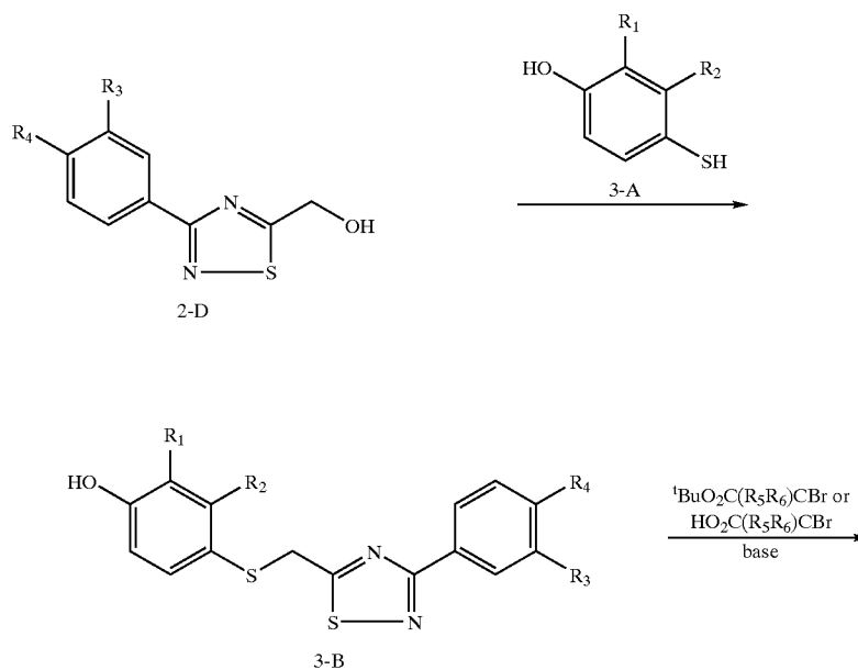
Scheme 3. Synthesis of Compound 2-F
