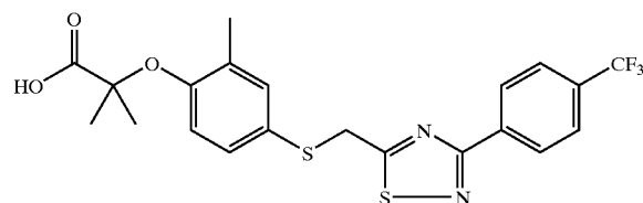
2-Methyl-2-{2-methyl-4-[3-(4-trifluoromethyl-phenyl)-[1,2,4]thiadiazol-5-ylmethylsulfanyl]-phenoxy}-propionic acid
