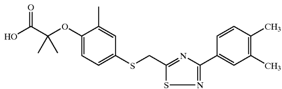
2-{4-[3-(3,4-Dimethyl-phenyl)-[1,2,4]thiadiazol-5-ylmethylsulfanyl]-2-methyl-phenoxy}-2-methyl-propionic acid
