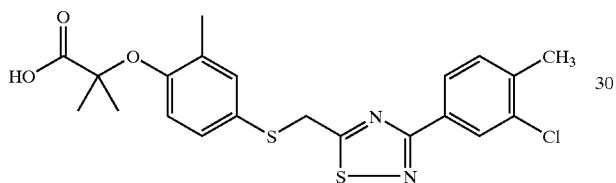
2-{4-[3-(3-Chloro-4-methyl-phenyl)-[1,2,4]thiadiazol-5-ylmethylsulfanyl]-2-methyl-phenoxy}-2-methyl-propionic acid
