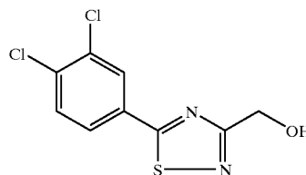
[5-(3,4-Dichloro-phenyl)-[1,2,4]thiadiazol-3-yl]-methanol
