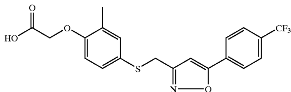
{2-Methyl-4-[5-(4-trifluoromethyl-phenyl)-isoxazol-3-ylmethylsulfanyl]-phenoxy}-acetic acid
