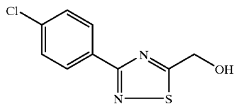
[3-(4-Chloro-phenyl)-[1,2,4]thiadiazol-5-yl]-methanol
