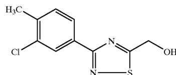
[3-(3-Chloro-4-methyl-phenyl)-[1,2,4]thiadiazol-5-yl]-methanol
