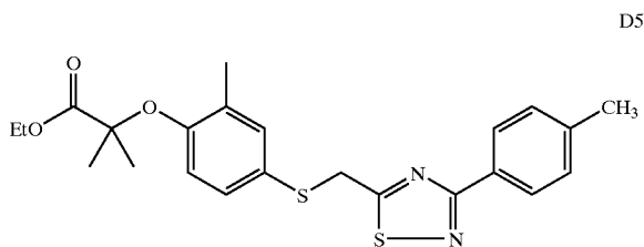
2-Methyl-2-[2-methyl-4-(3-p-tolyl-[1,2,4]thiadiazol-5-ylmethylsulfanyl)-phenoxy]-propionic acid ethyl ester
