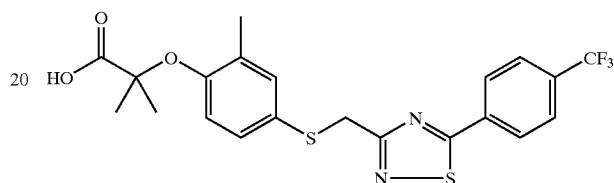
2-Methyl-2-{2-methyl-4-[5-(4-trifluoromethyl-phenyl)-[1,2,4]thiadiazol-3-ylmethylsulfanyl]-phenoxy}-propionic acid
