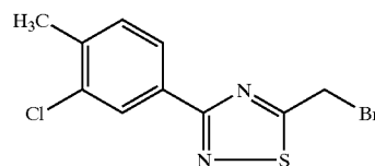
5-Bromomethyl-3-(3-chloro-4-methyl-phenyl)-[1,2,4]thiadiazole
