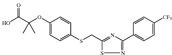
2-Methyl-2-{4-[3-(4-trifluoromethyl-phenyl)-[1,2,4]thiadiazol-5-ylmethylsulfanyl]-phenoxy}-propionic acid
