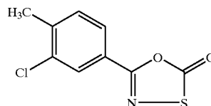
5-(3-Chloro-4-methyl-phenyl)-[1,3,4]oxathiazol-2-one
