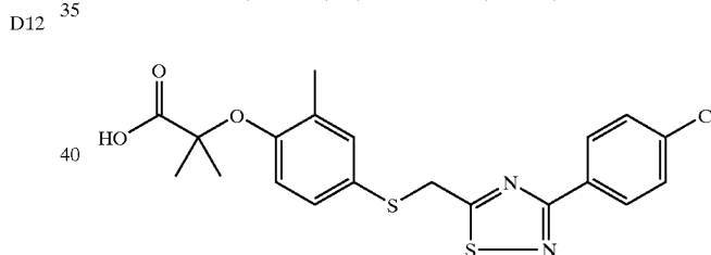
2-{4-[3-(4-Chloro-phenyl)-[1,2,4]thiadiazol-5-ylmethylsulfanyl]-2-methyl-phenoxy}-2-methyl-propionic acid
