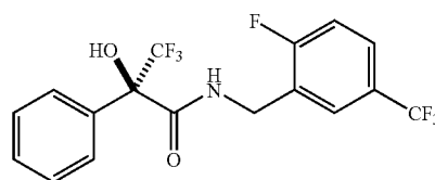
(2R)-3,3,3-trifluoro-N-(2-fluoro-5-trifluoromethylbenzyl)-2-hydroxy-2-phenylpropanamide.
