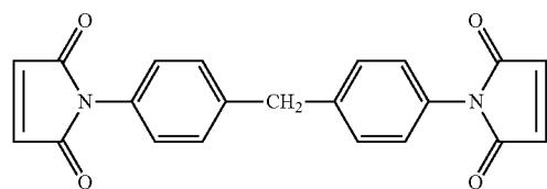
Compimide MDAB
