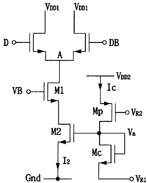
FIG. 3 (Background Art)
