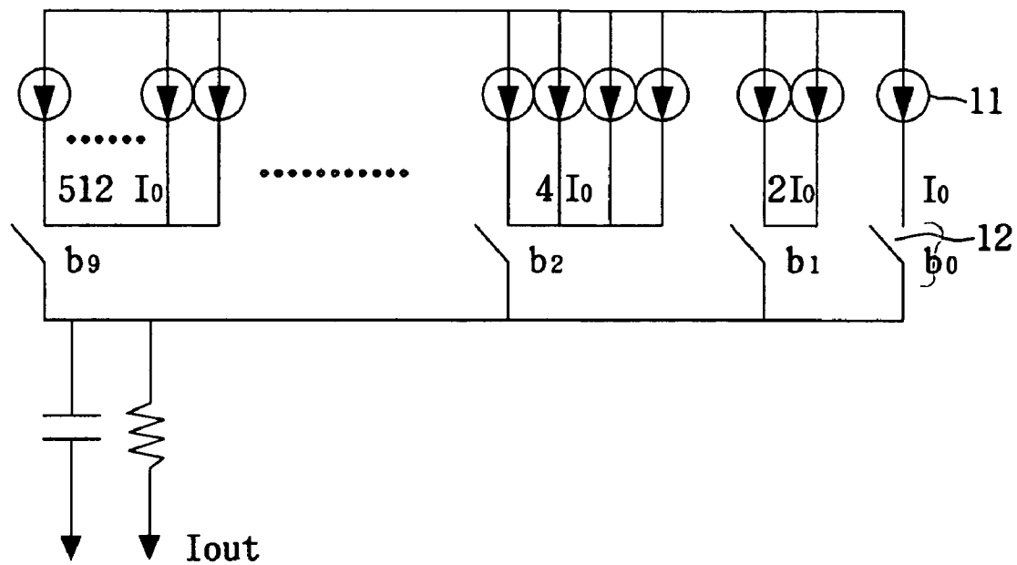
FIG. 1 (Background Art)
