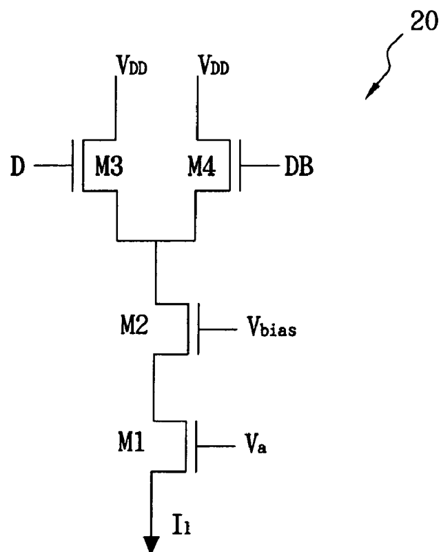
FIG. 2 (Background Art)
