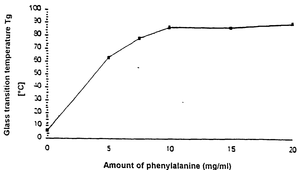
Figure 1 a: Glass transition temperature of individual Maltose-L-Phenylalanine mixtures
