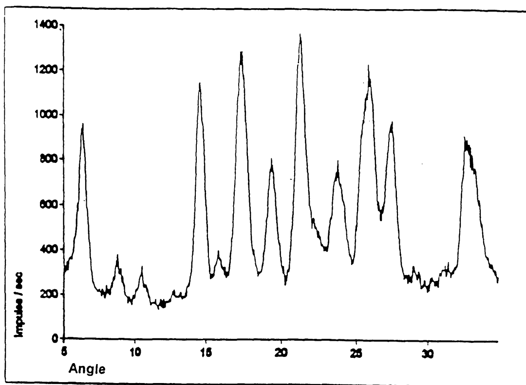
Figure 2 a: Phenylalanine 0.12 m vacuum-dried (crystalline, water content 1.2%)
