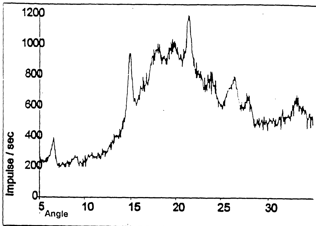
Figure 2 c: Maltose + 10 mg Phenylalanine/ml - vacuum-dried ( T_g = 88^\circ\text{C} , water content = 0.7 %)
