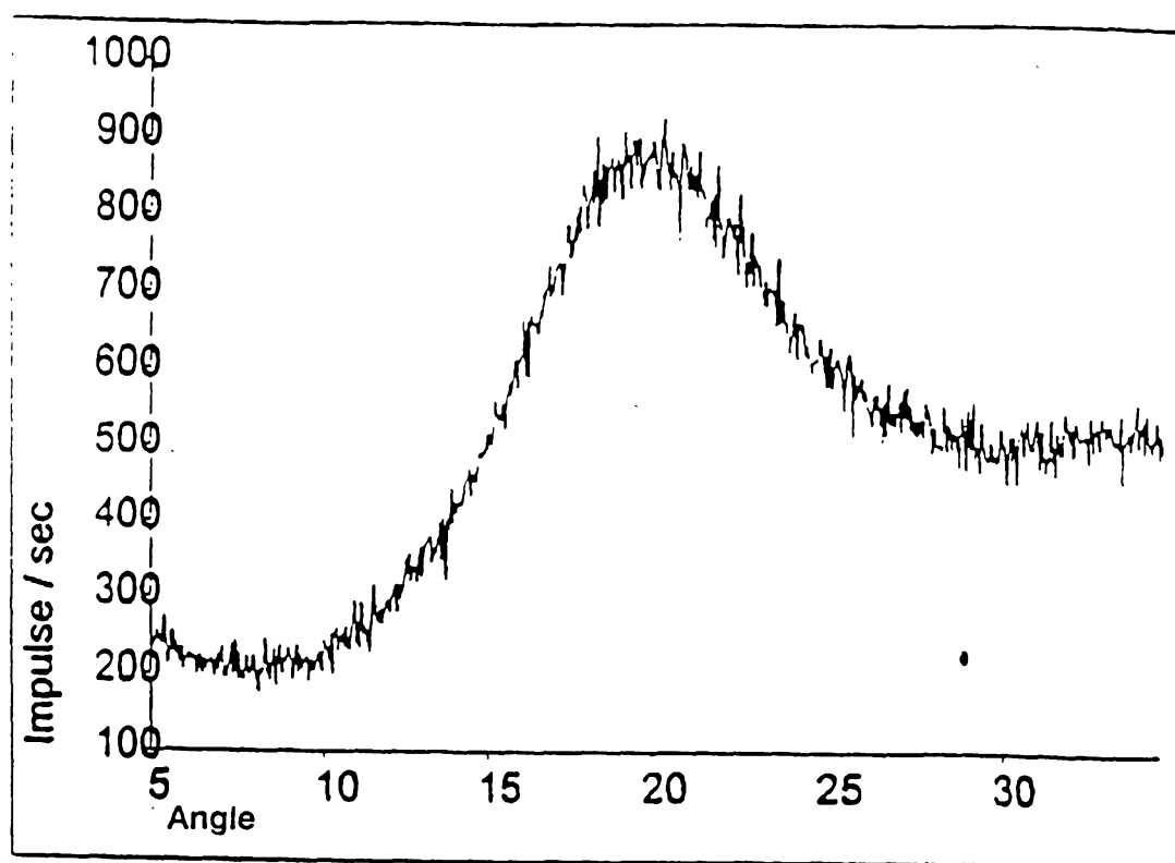
Figure 2 b: Maltose vacuum-dried ( T_g = 50.1^\circ\text{C} , water content = 4.0 %)
