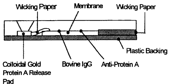
CROSS SECTION
