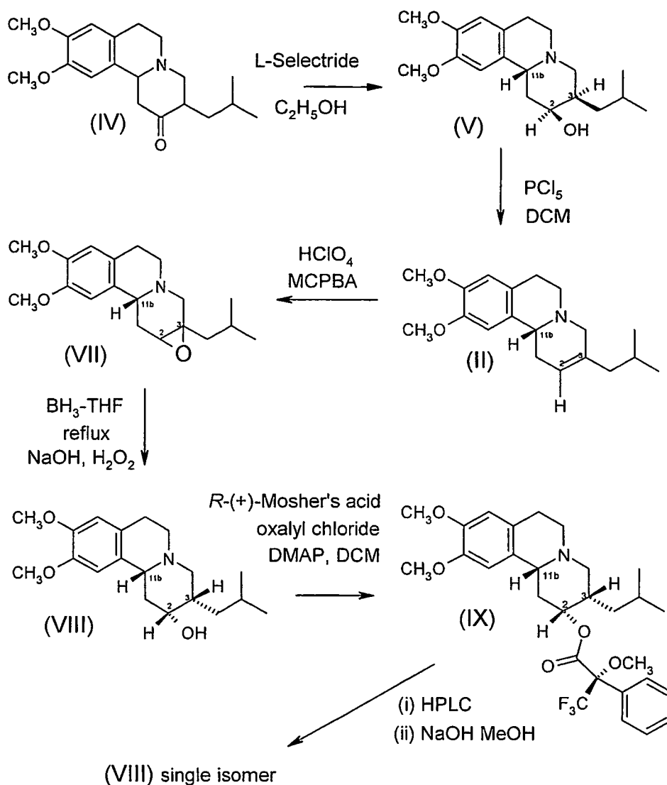
Scheme 2
