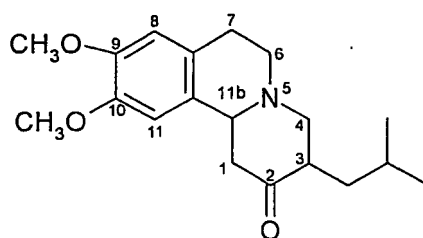
Figure 1- Structure of tetrabenazine
