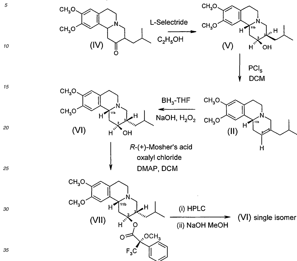
Scheme 1
