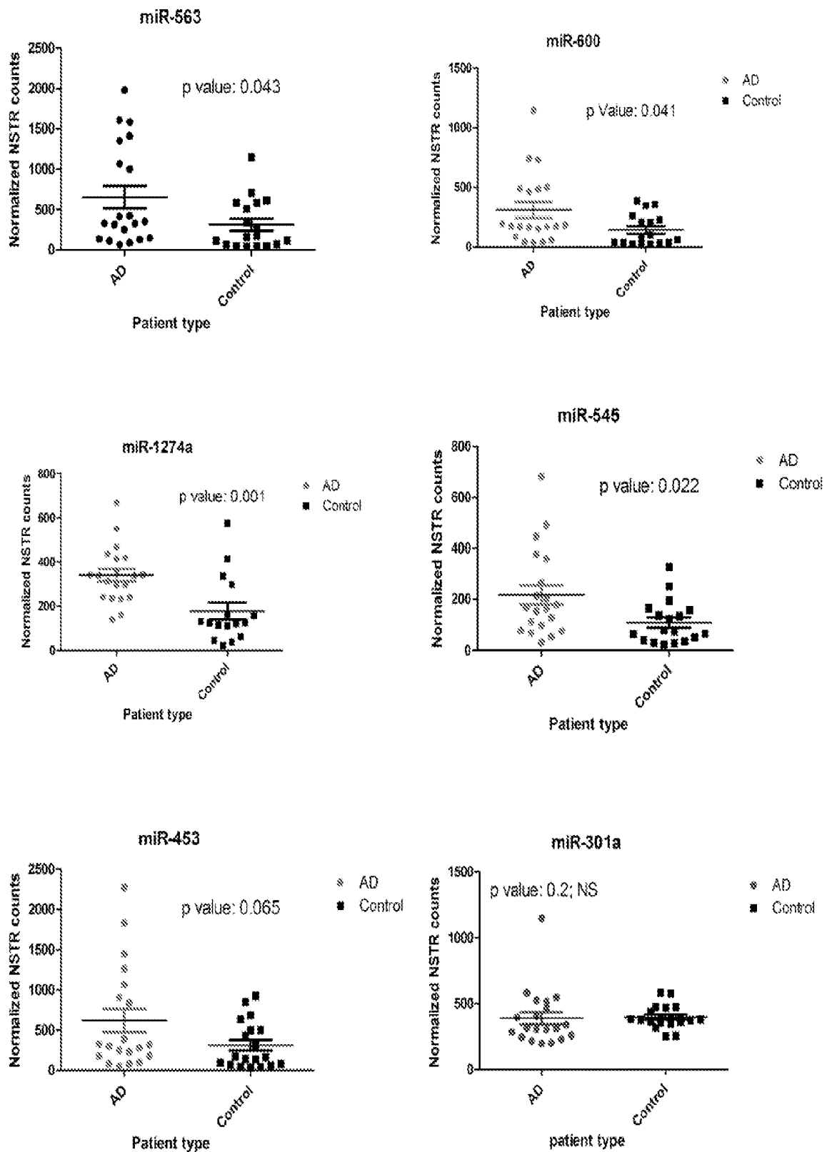
Figure 1B: Scatter plots of individual miRNA values post normalization for 20 (AD+MCI) and 20 Control patients (Cohort 1) using Nanostring.
