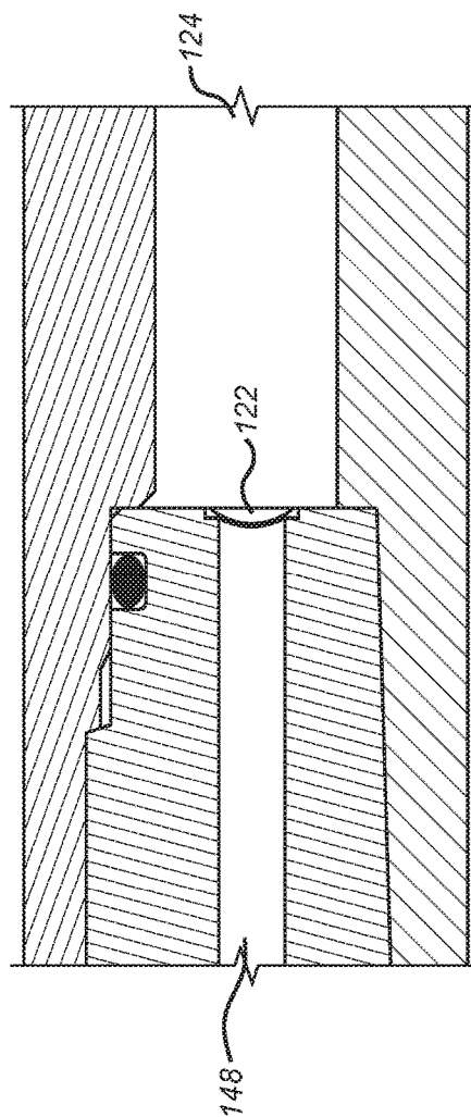
(PRIOR ART) FIG. 4
