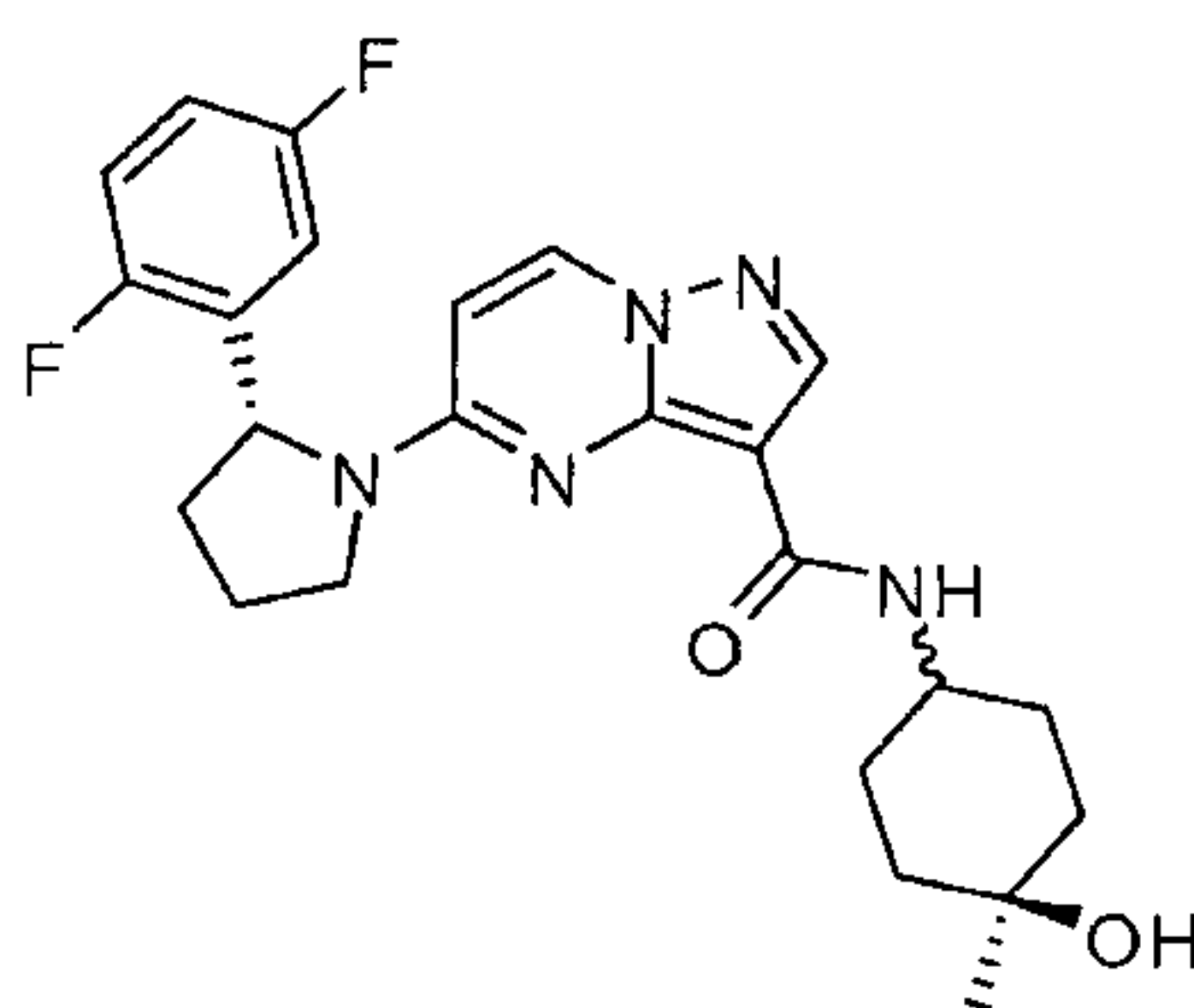
5-((R)-2-(2,5-difluorophenyl)pyrrolidin-1-yl)-N-(4-hydroxy-4-methylcyclohexyl)pyrazolo[1,5-a]pyrimidine-3-carboxamide (Diastereomer 2)
