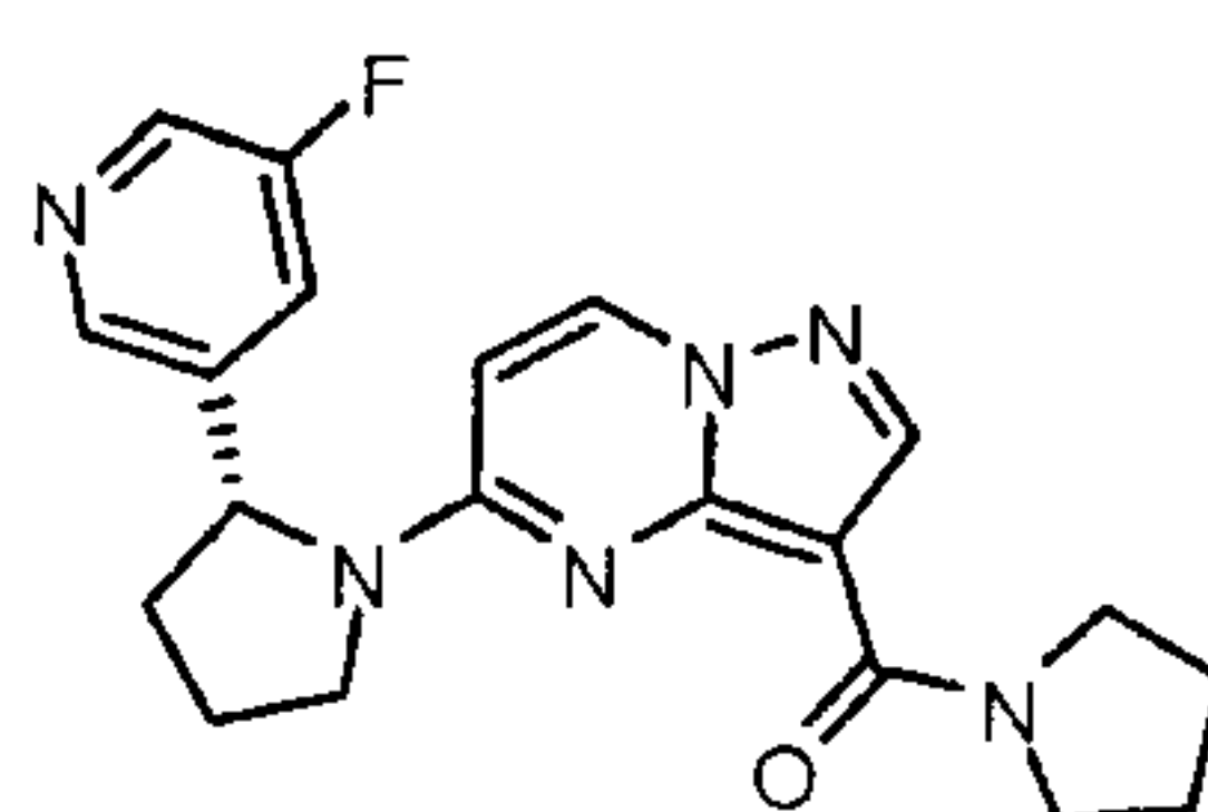
(R)-5-(2-(5-fluoropyridin-3-yl)pyrrolidin-1-yl)pyrazolo[1,5-a]pyrimidine-3-yl(pyrrolidin-1-yl)methanone
