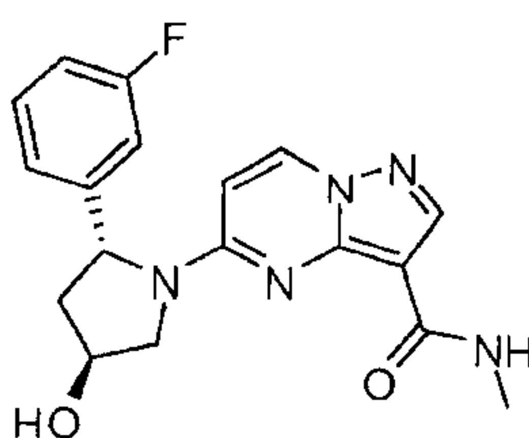
5-((2R,4S)-2-(3-fluorophenyl)-4-hydroxypyrrolidin-1-yl)-N-methylpyrazolo[1,5-a]pyrimidine-3-carboxamide
