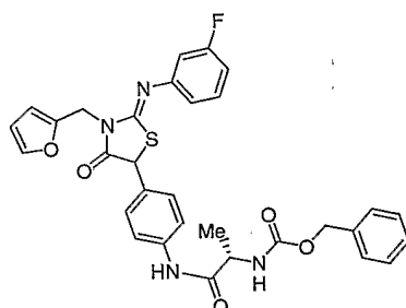
Compound 1
