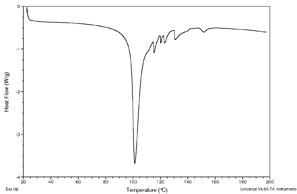
Figure H: DSC Thermogram of Form B of Example 3.13b
