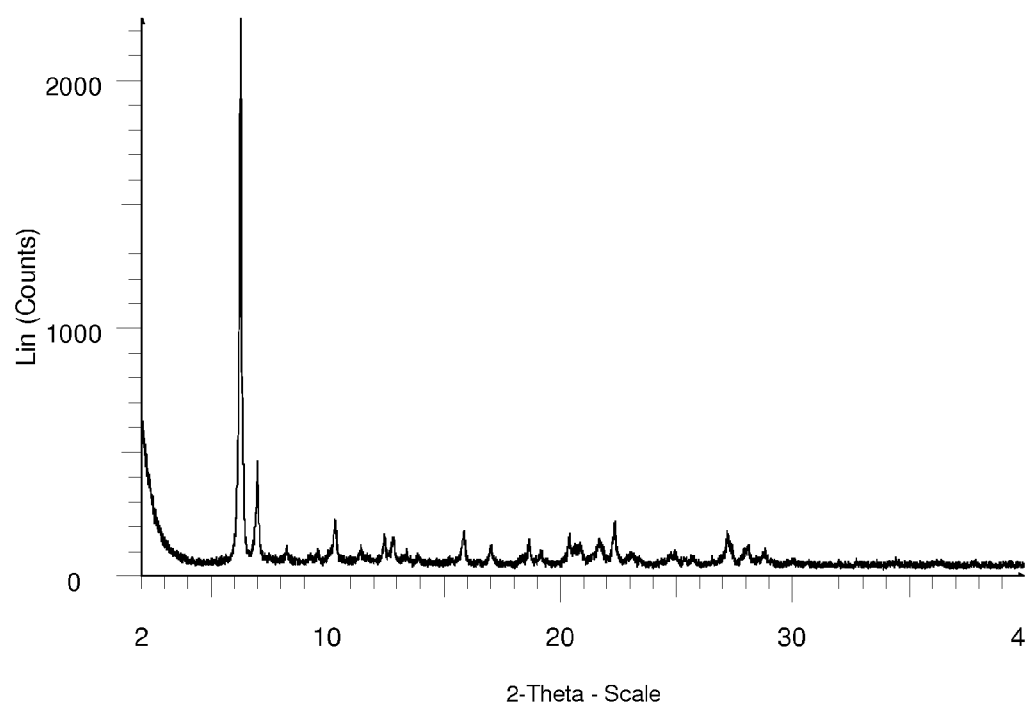
Figure G: X-Ray Powder Diffraction Pattern of Form B of Example 3.13b
