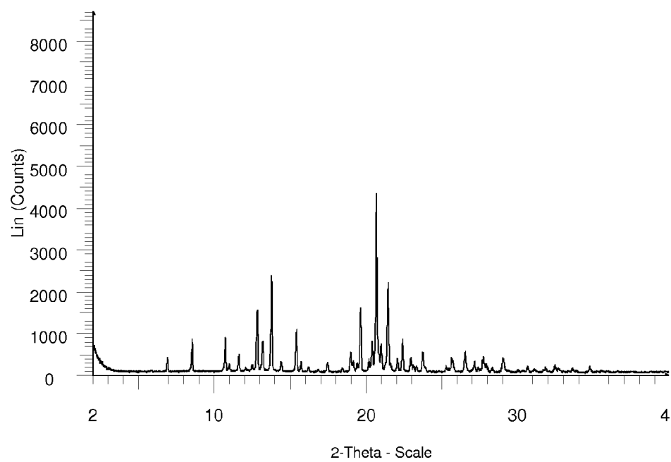
Figure C: X-Ray Powder Diffraction Pattern of Form B of Example 3.06b
