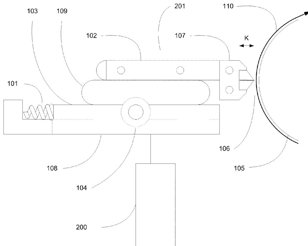
FIG. 2 SIDE VIEW
