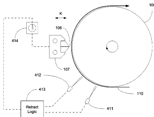
Feed-Forward Control
