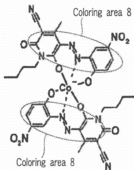
Structural formula of azo metal complex
