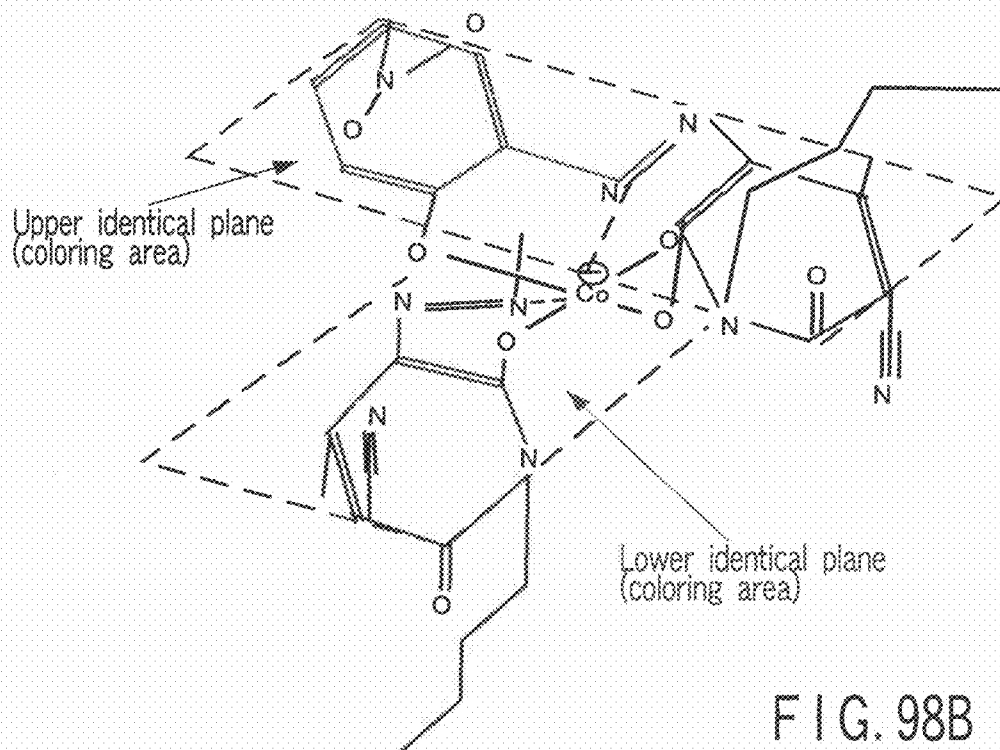
Three-dimensional structure of azo metal complex
