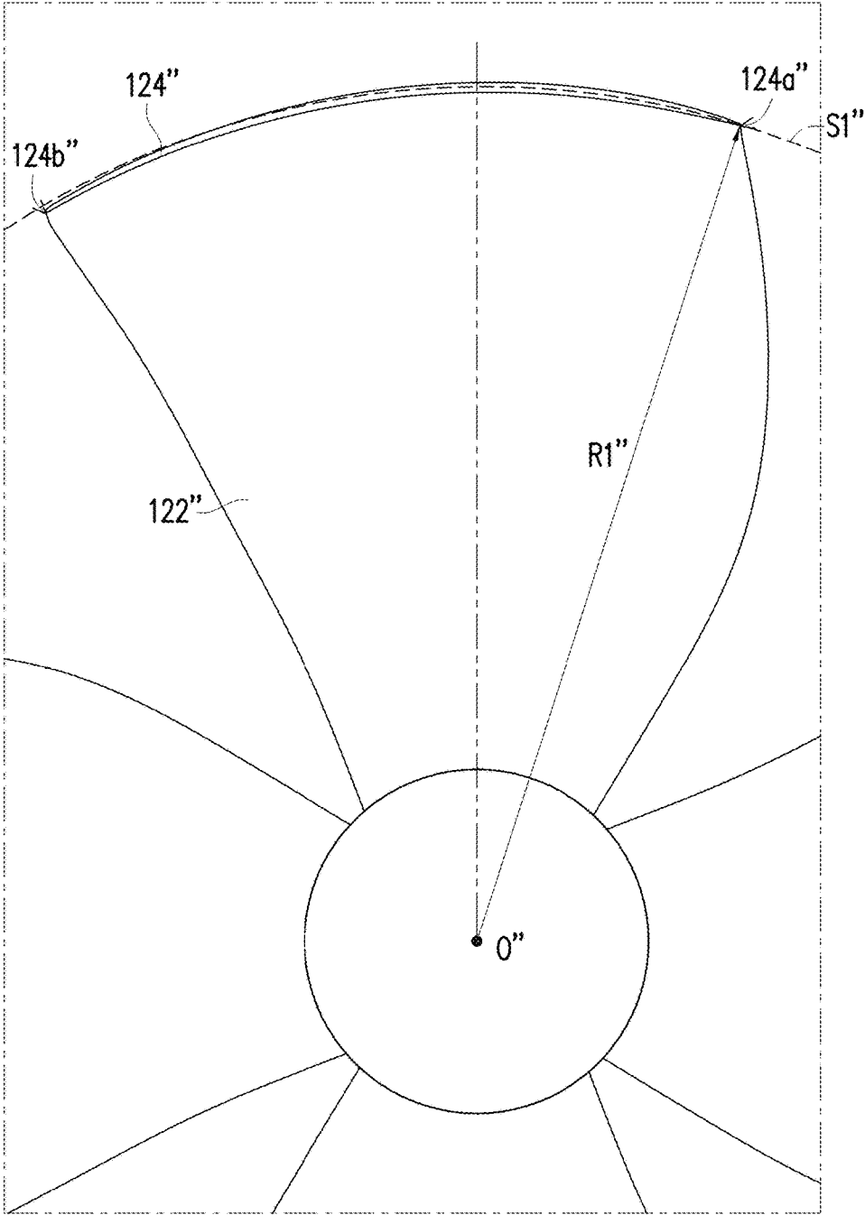
FIG. 6C (RELATED ART)
