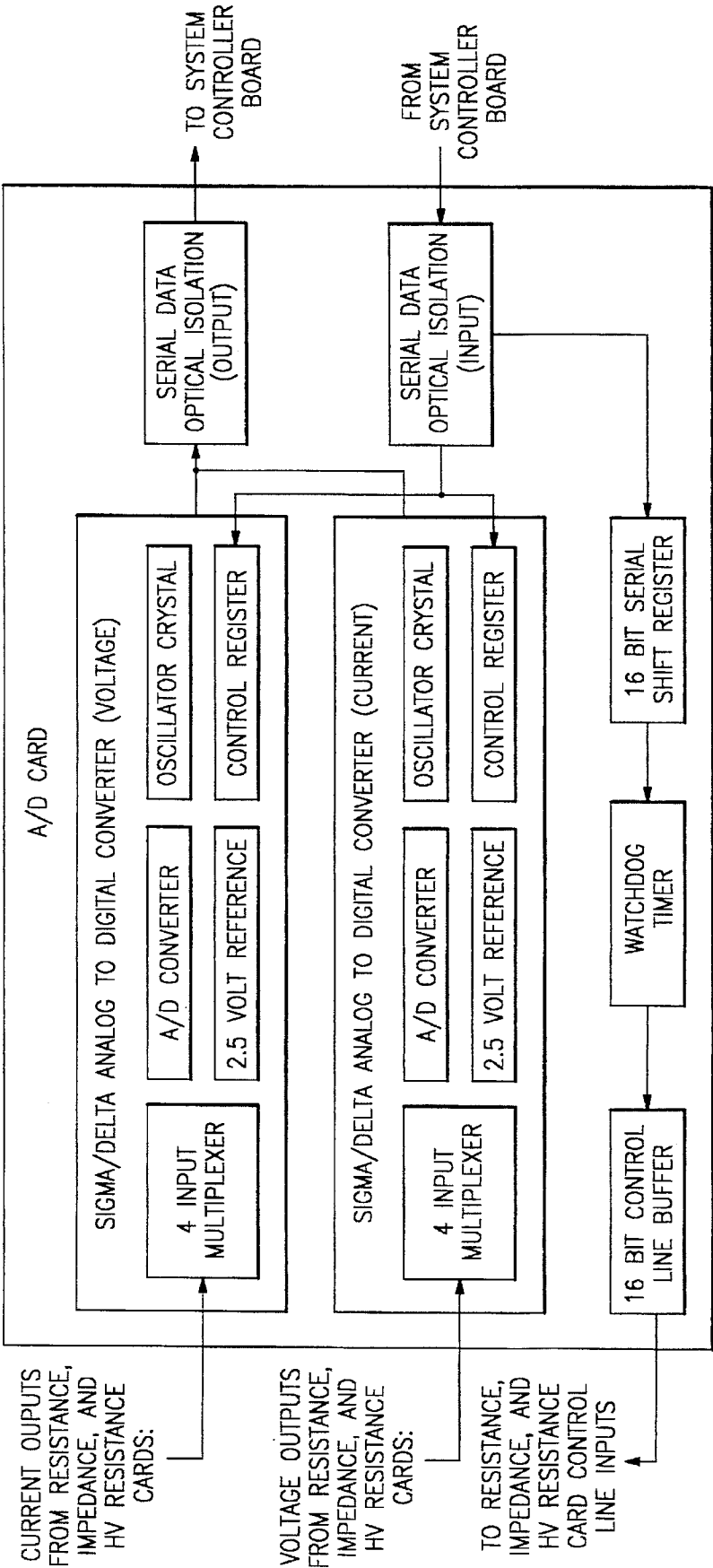
ANALOG TO DIGITAL CONVERSION CARD BLOCK DIAGRAM
