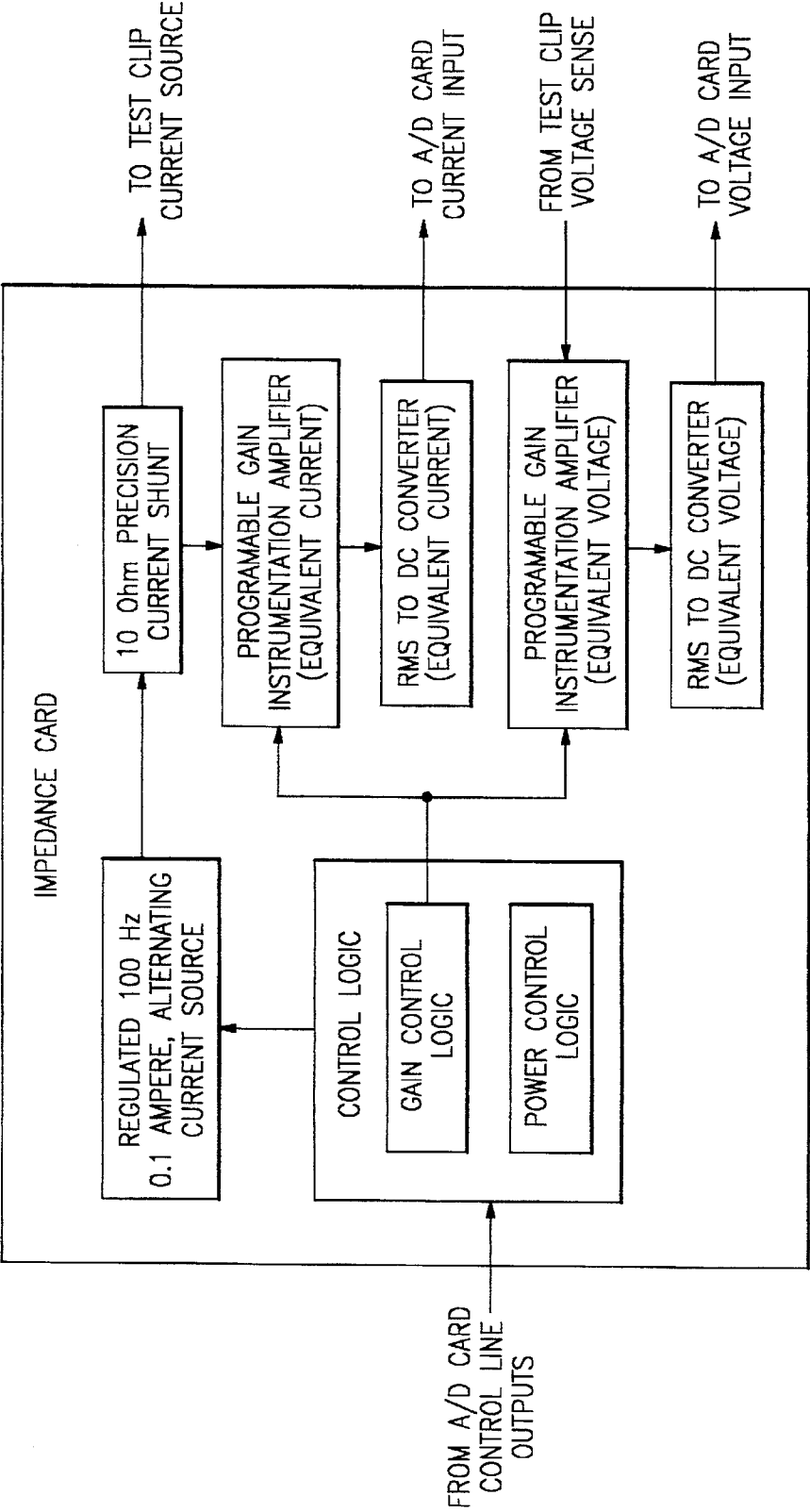
IMPEDANCE MEASUREMENT CARD BLOCK DIAGRAM
