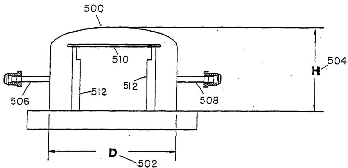
Wafer Chamber
