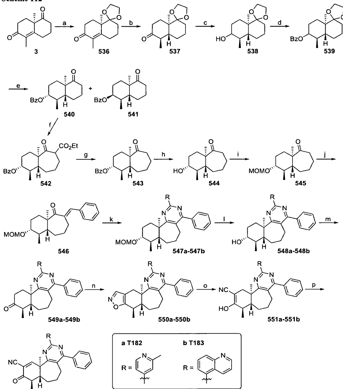
Scheme 112
