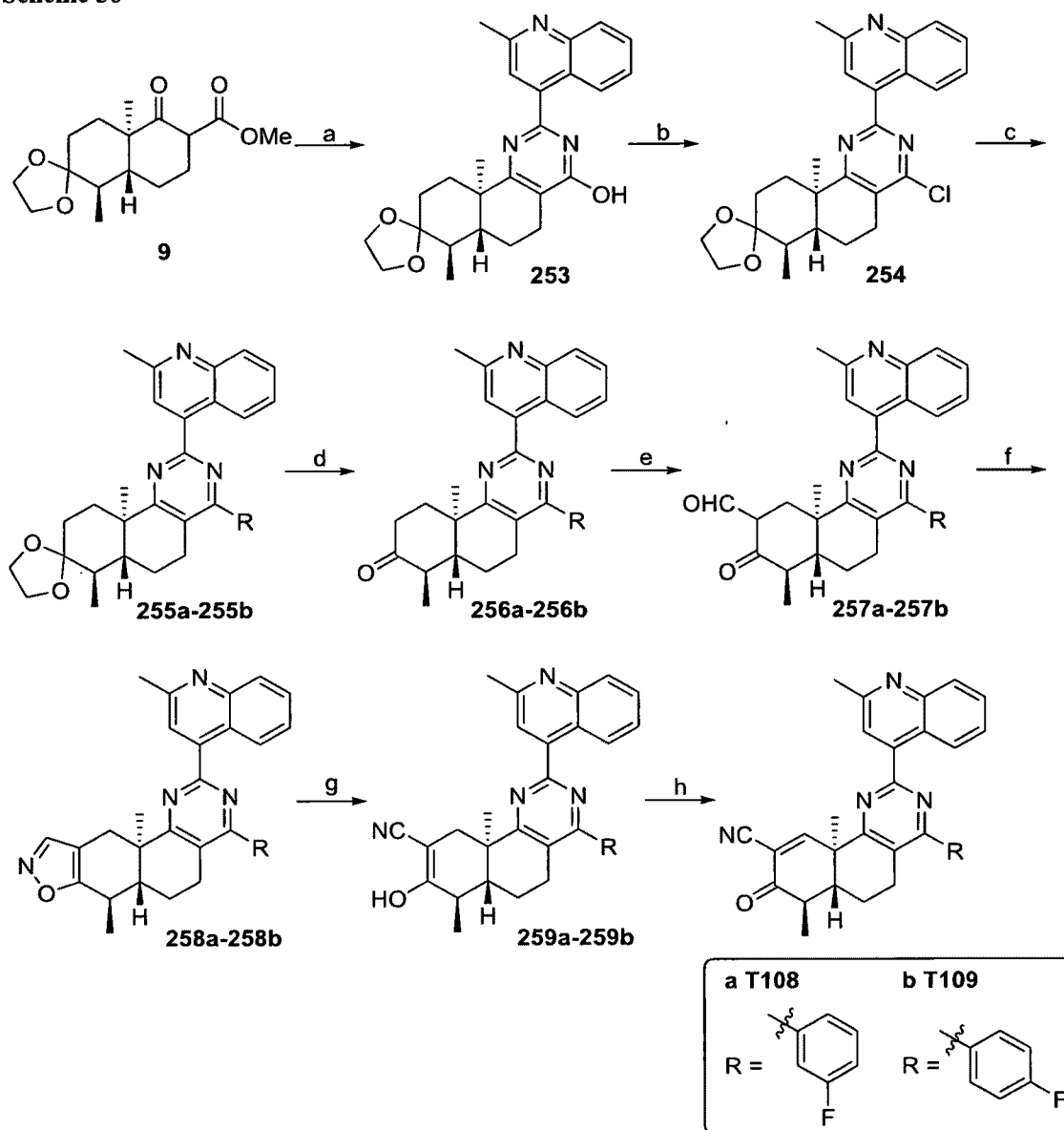
Scheme 56
