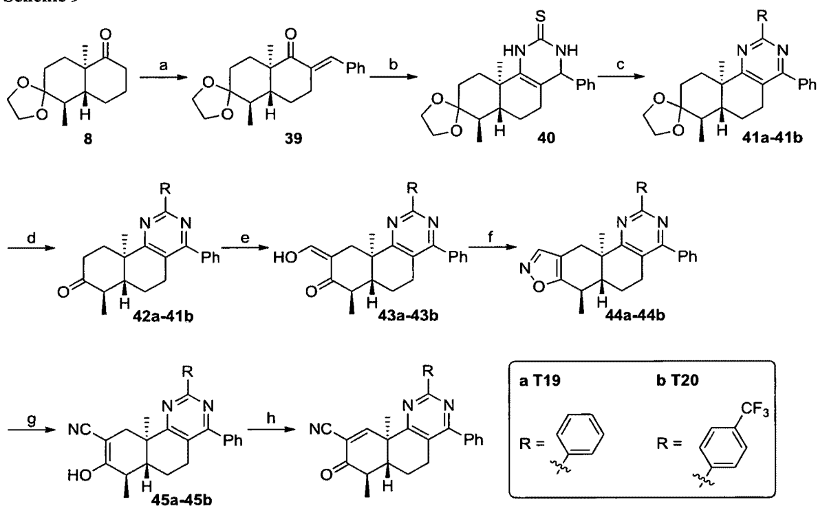
Scheme 9
