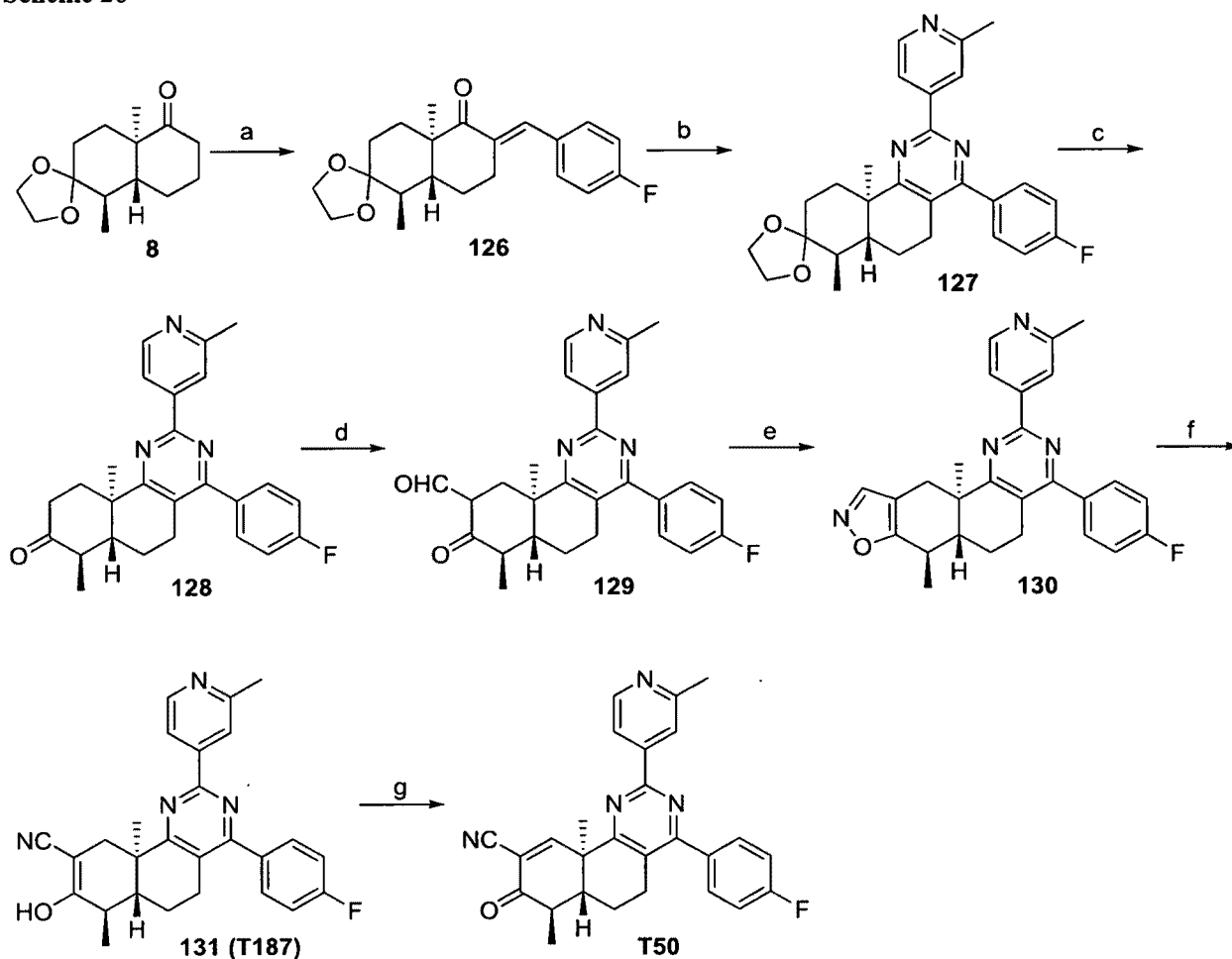
Scheme 26
