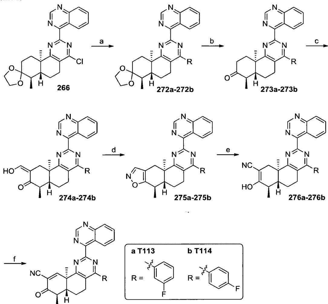
Scheme 59
