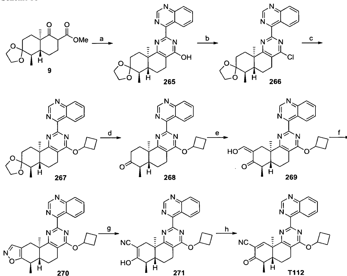
Scheme 58
