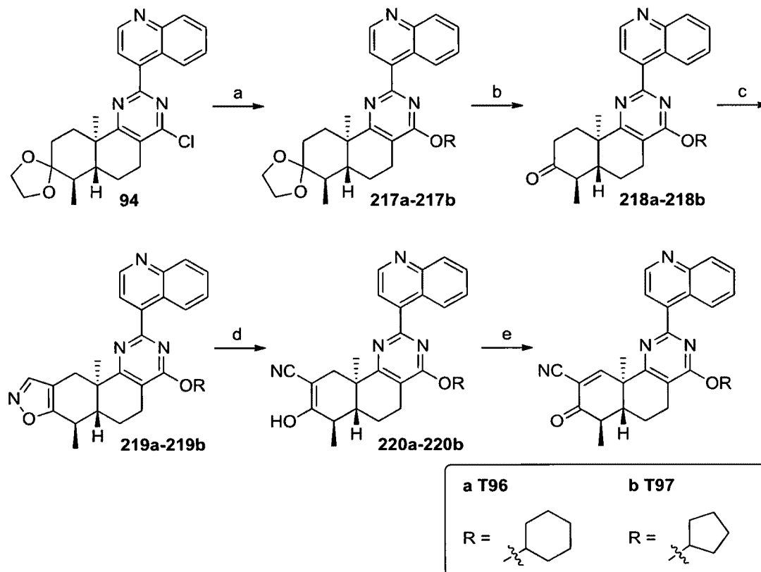
Scheme 48
