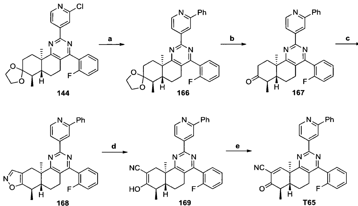
Scheme 34
