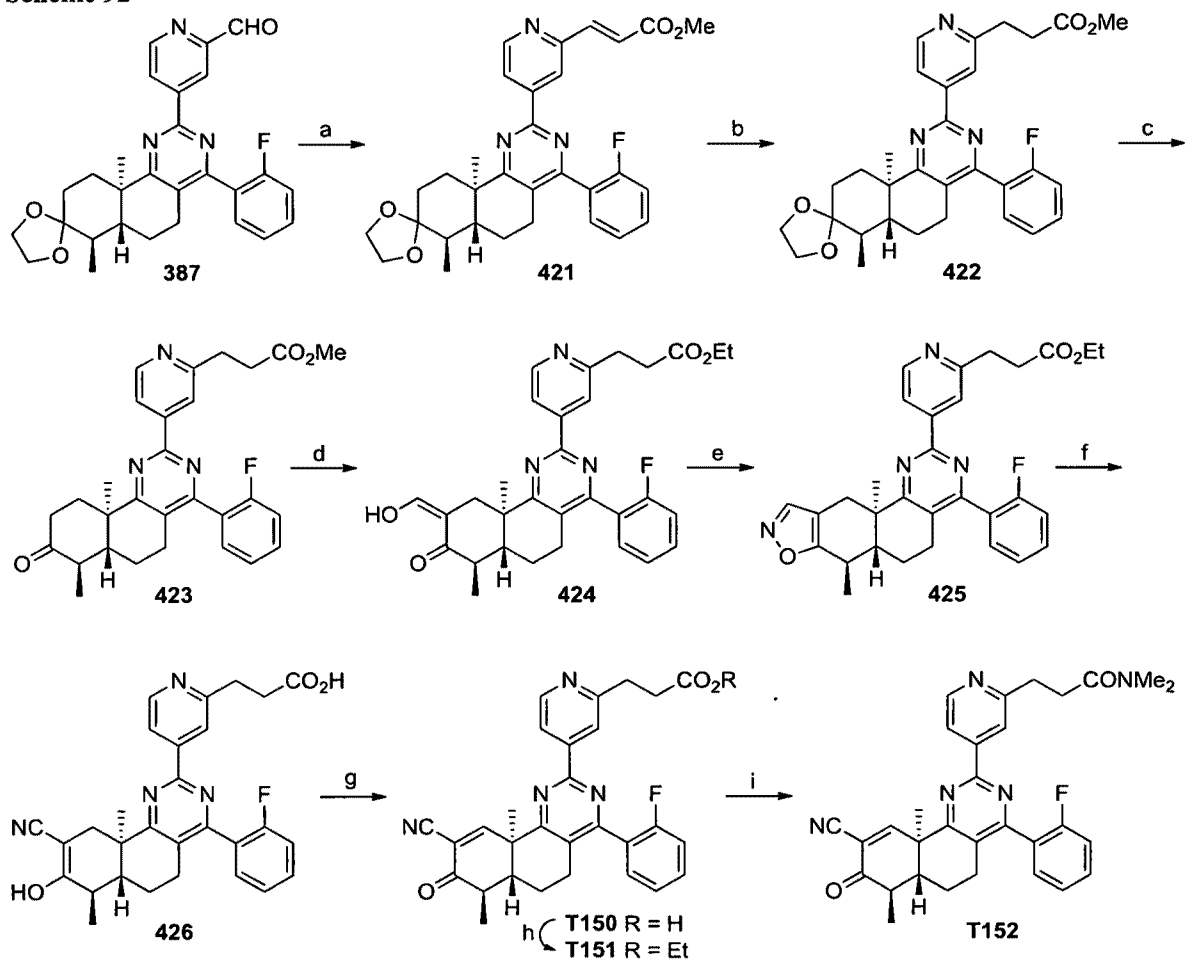
Scheme 92
