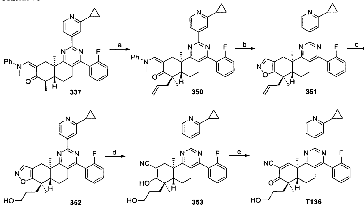
5 Scheme 78
