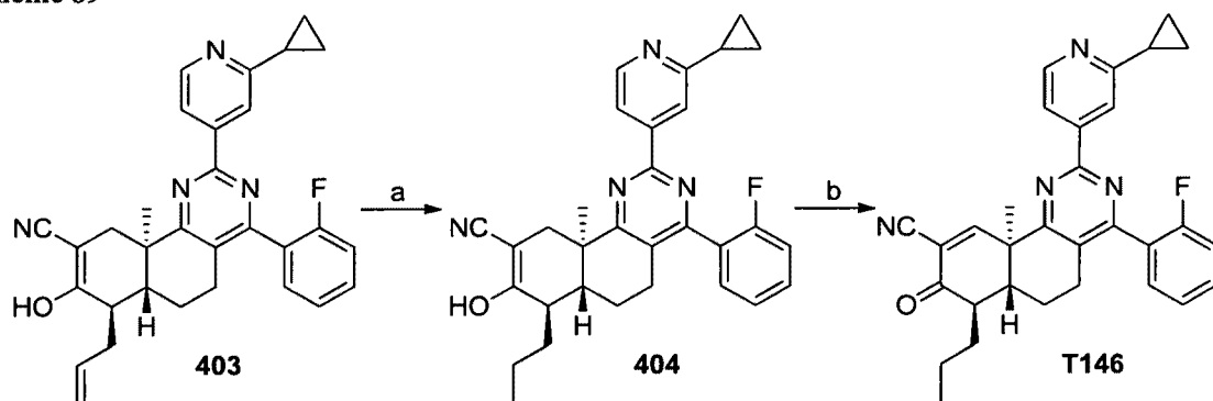
Scheme 89
