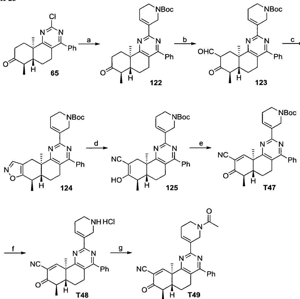
Scheme 25
