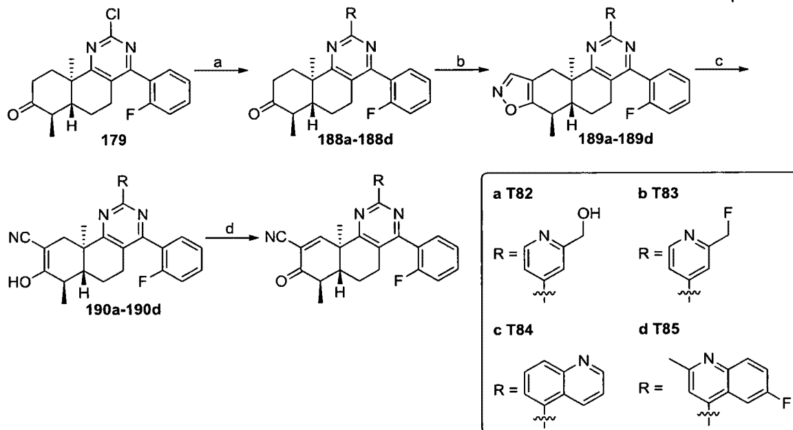
Scheme 40
