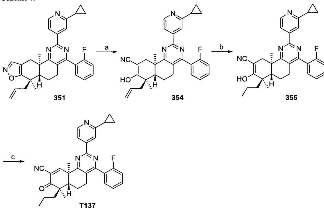
Scheme 79
