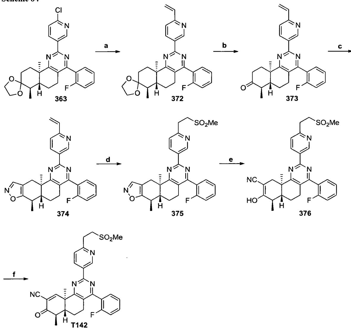
Scheme 84
