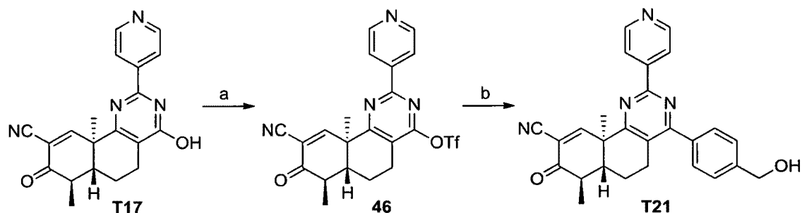
Scheme 10
