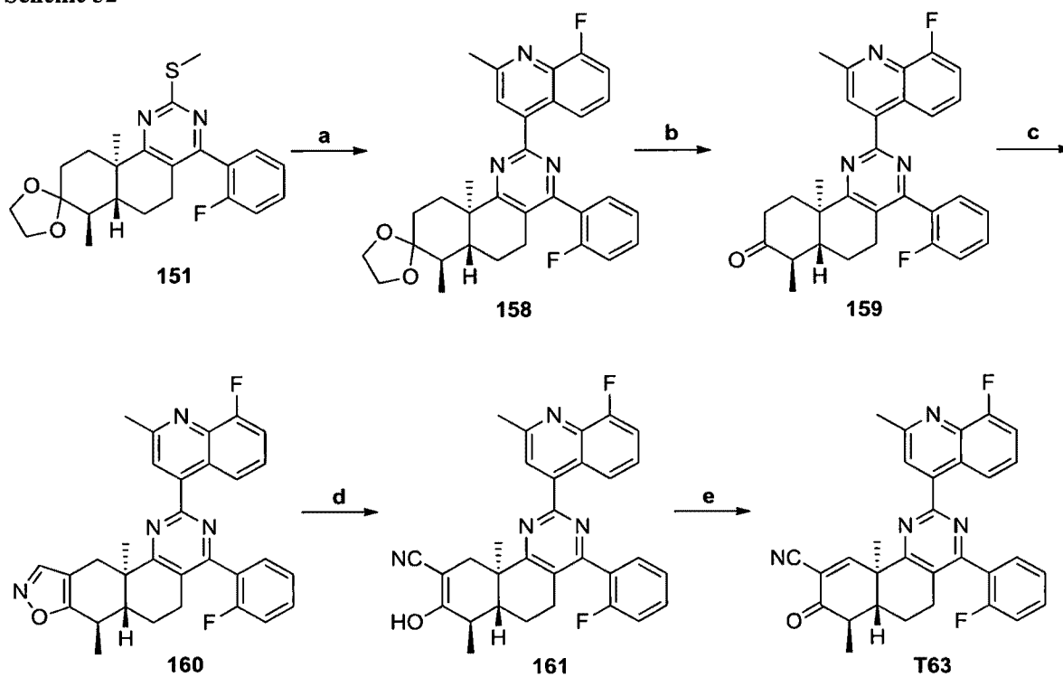
Scheme 32
