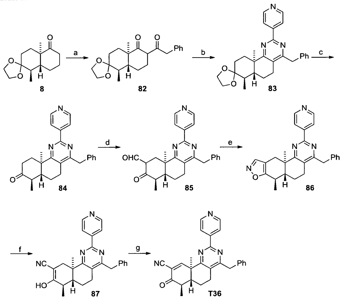
Scheme 17
