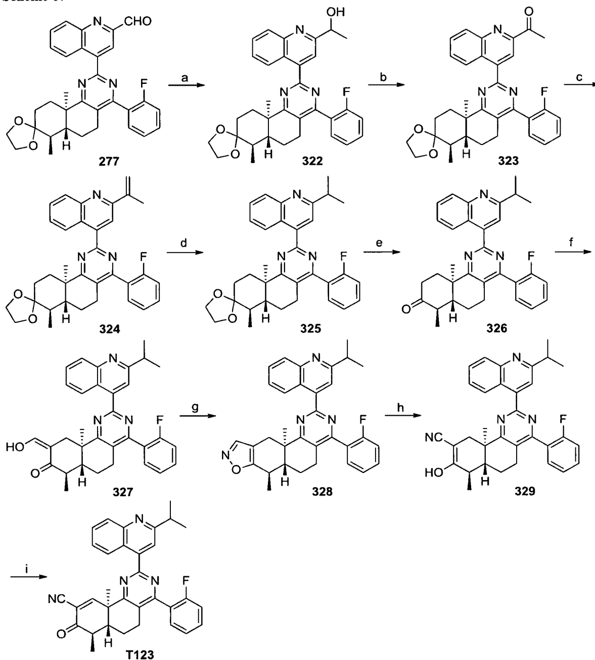
Scheme 67
