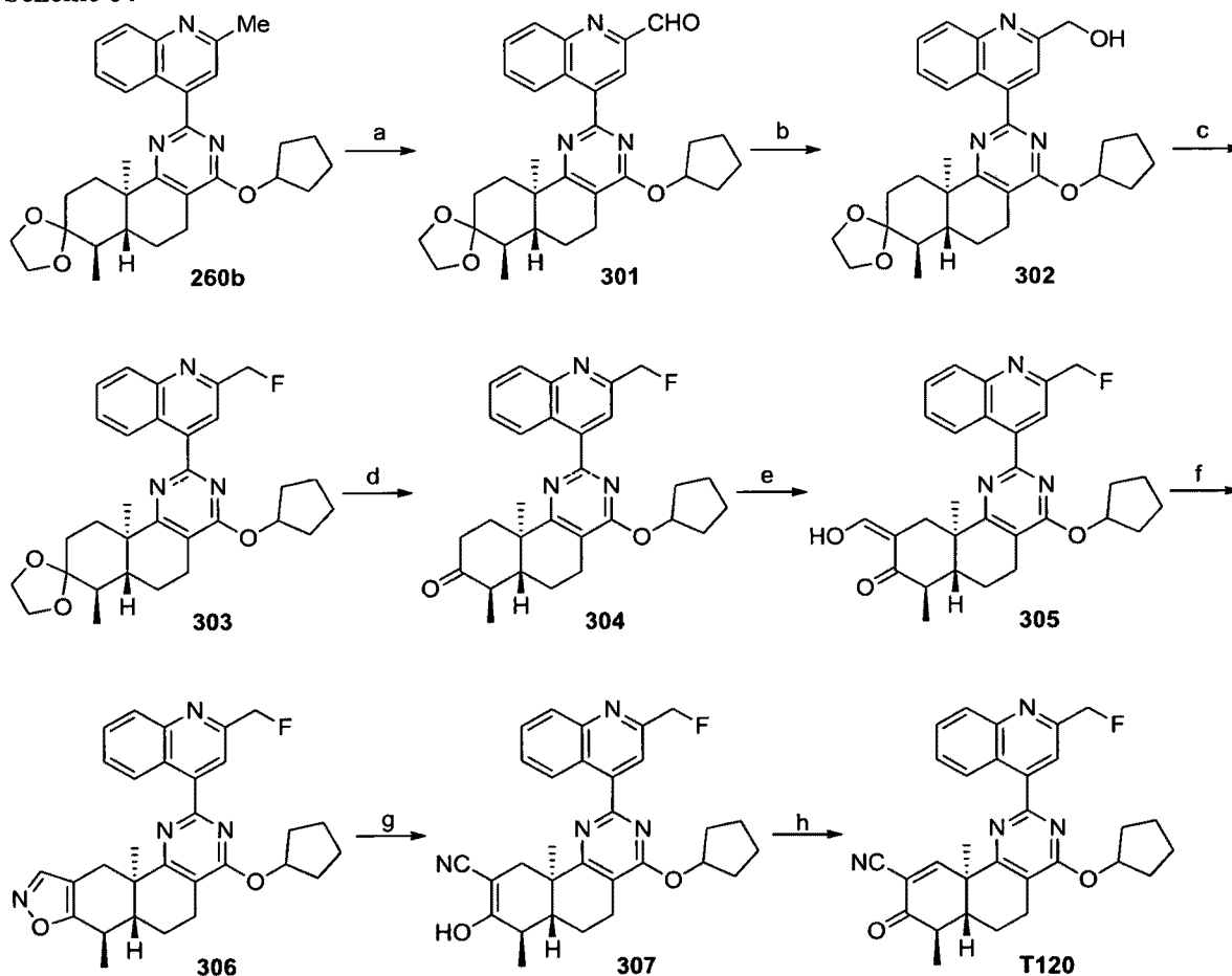
Scheme 64
