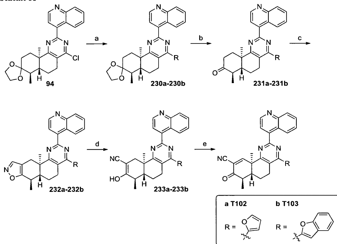
Scheme 51
