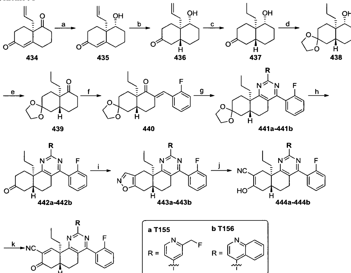
Scheme 95
