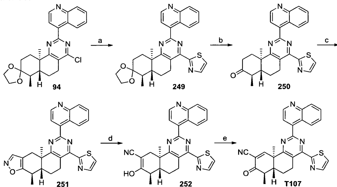
Scheme 55
