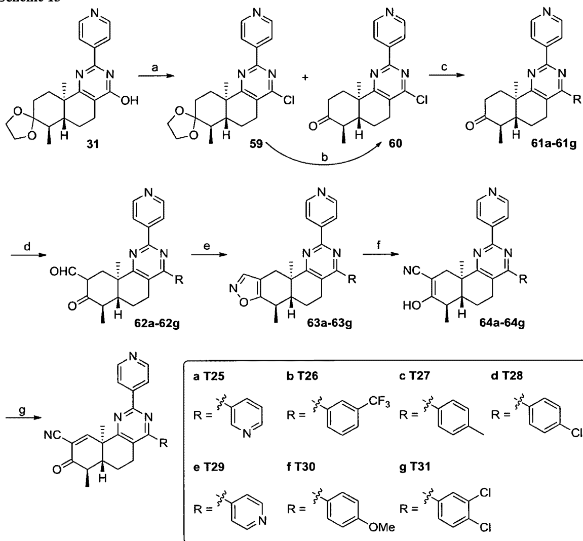
Scheme 13
