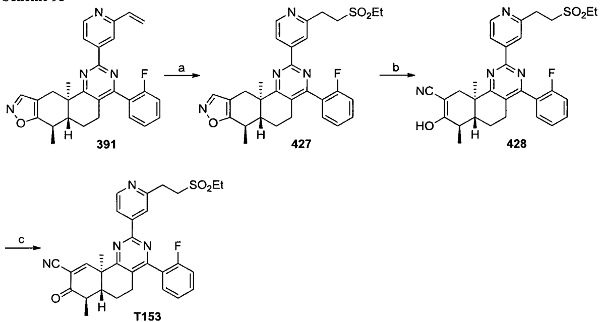
Scheme 93
