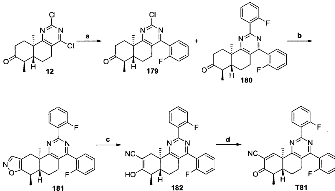
Scheme 37
