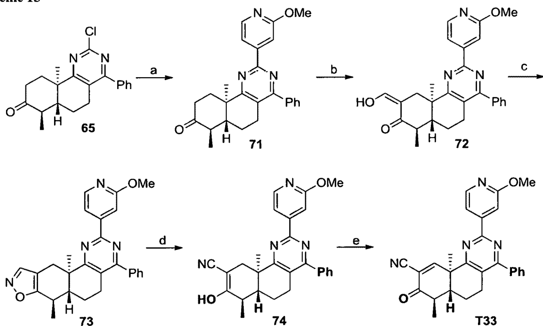
Scheme 15
