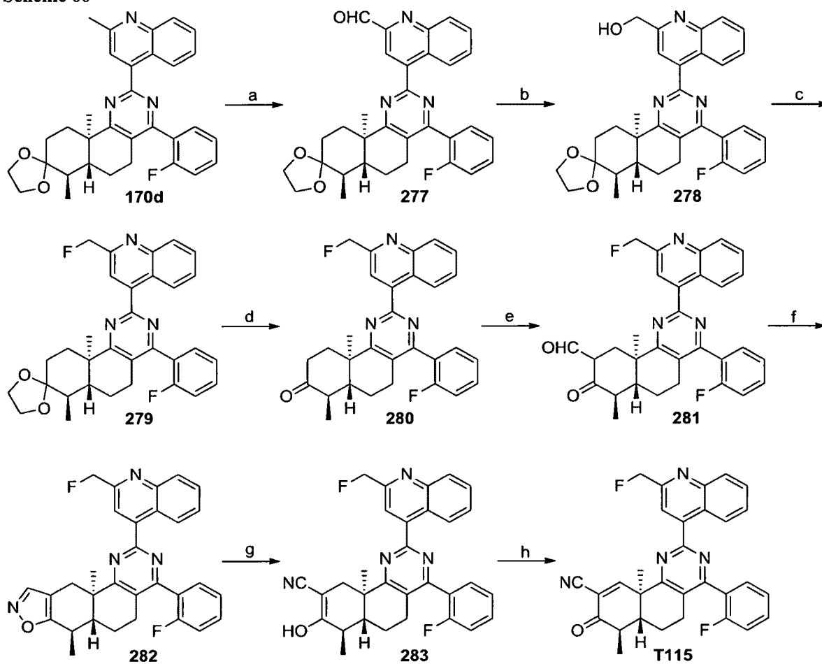
Scheme 60
