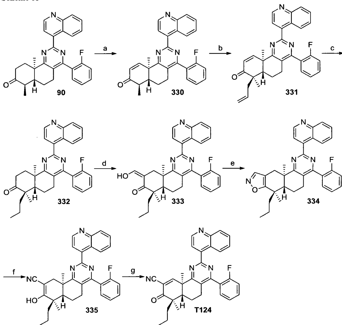
Scheme 68
