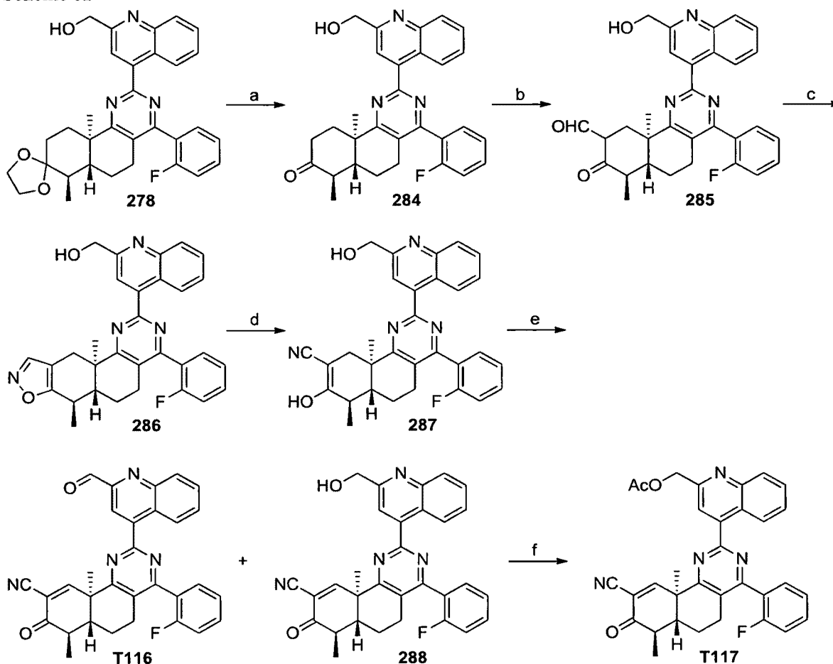
Scheme 61
