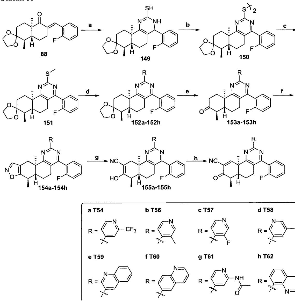
Scheme 30
