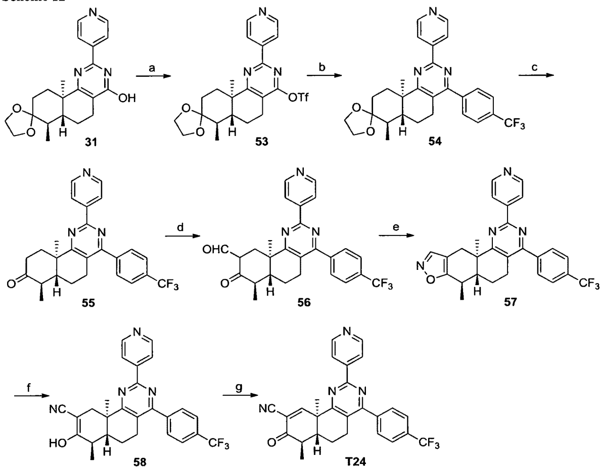
Scheme 12
