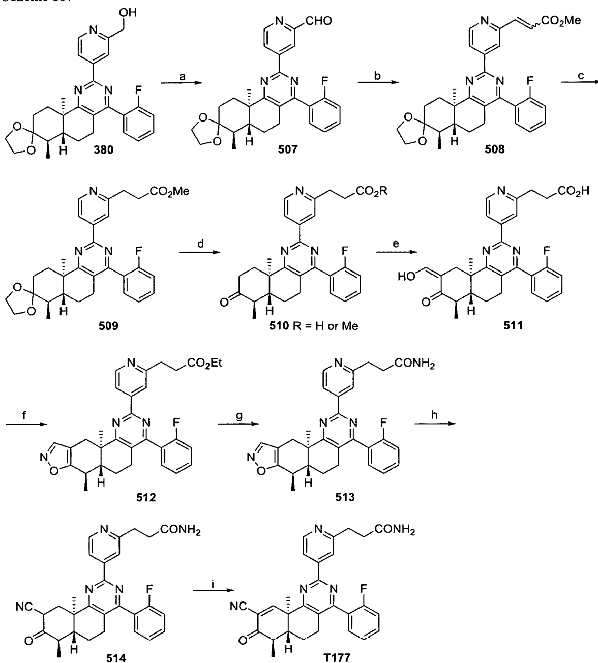
Scheme 107
