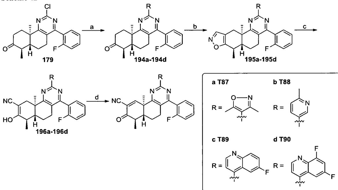
Scheme 42
