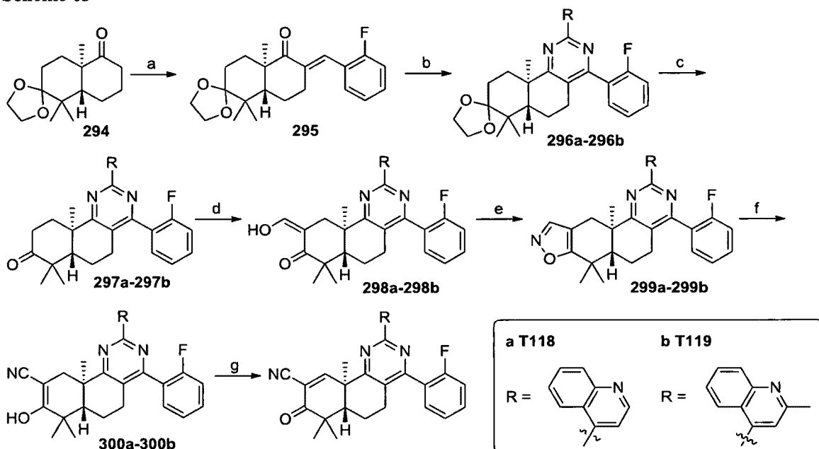
Scheme 63
