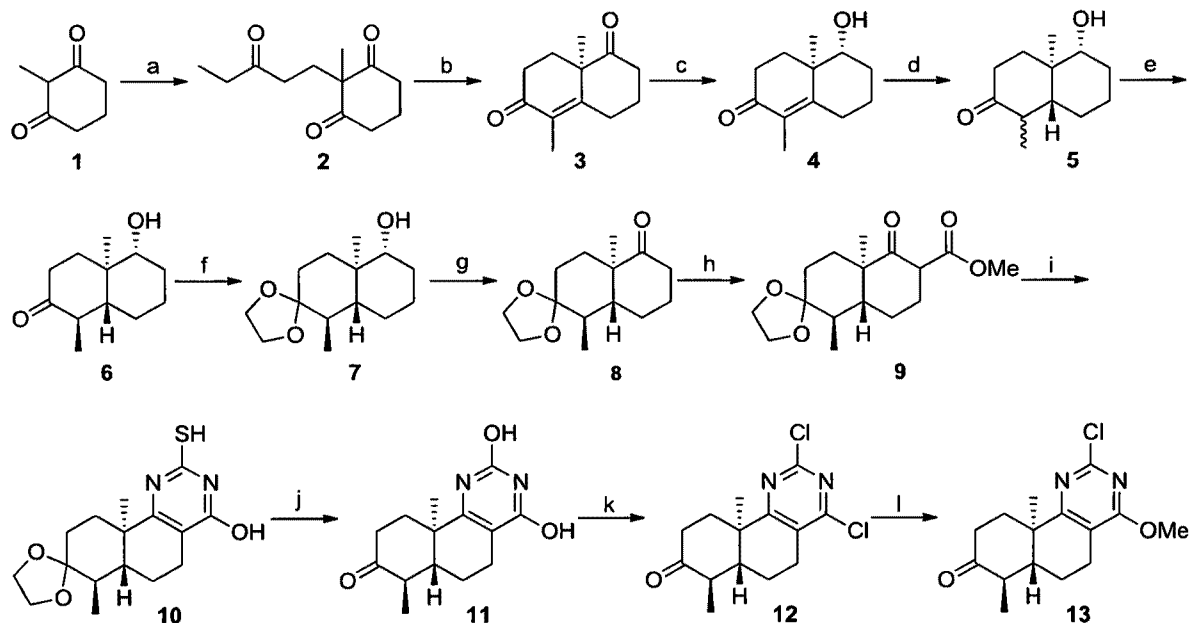
Scheme 1
