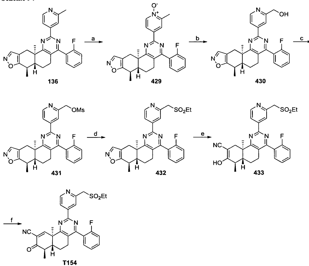
5 Scheme 94
