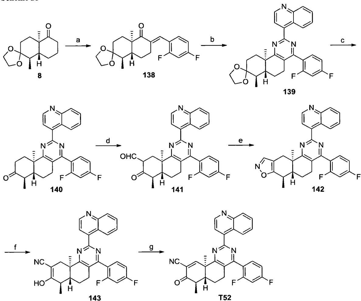
Scheme 28
