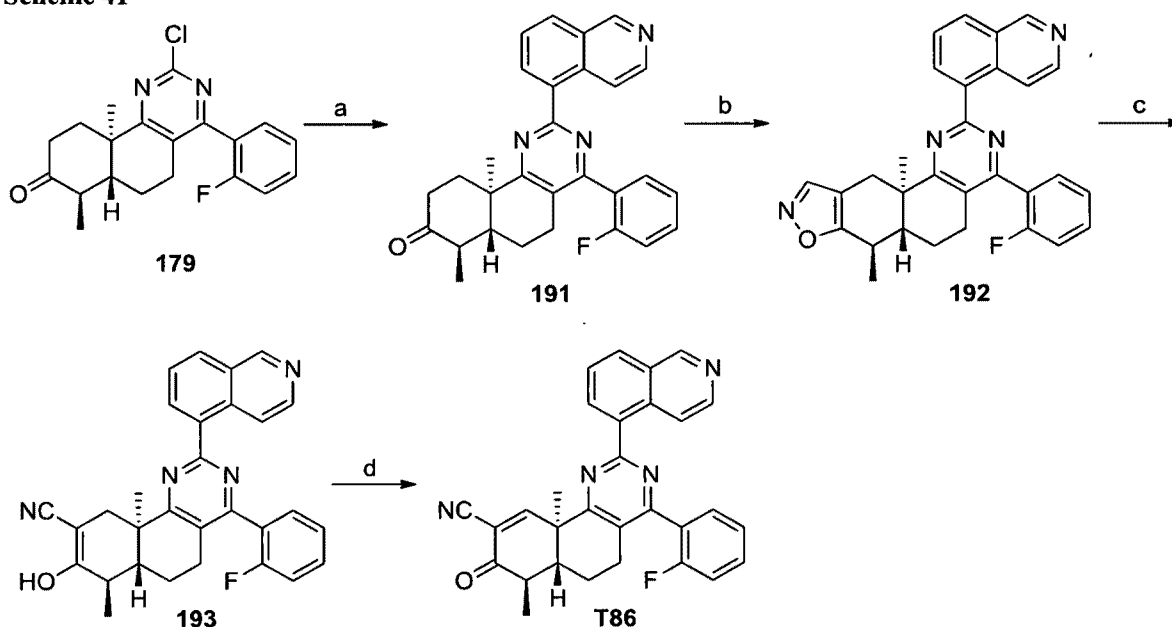
Scheme 41
