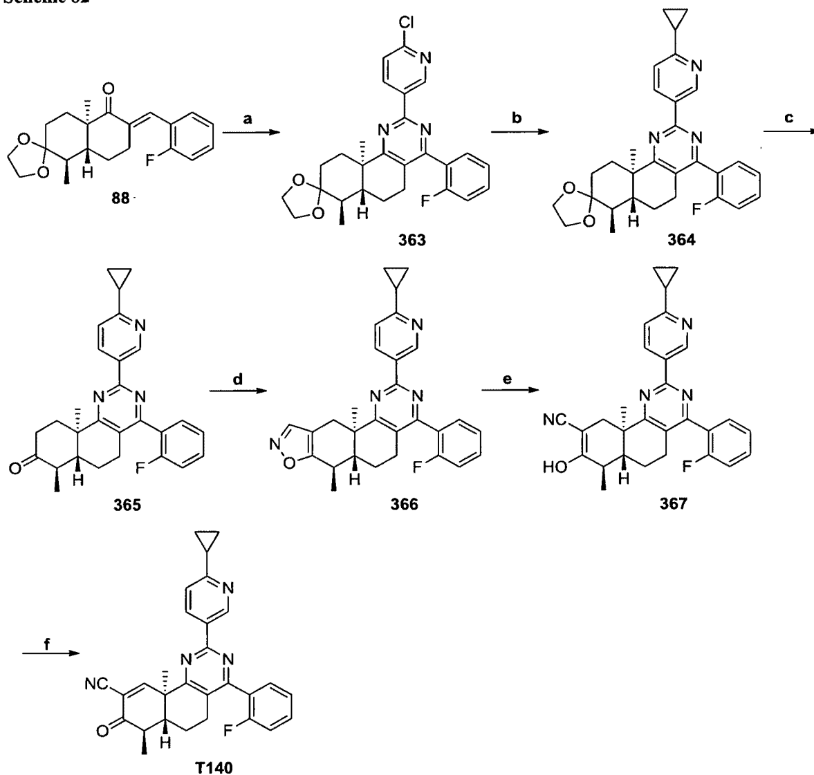
Scheme 82
