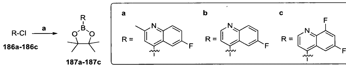
5 Scheme 39
