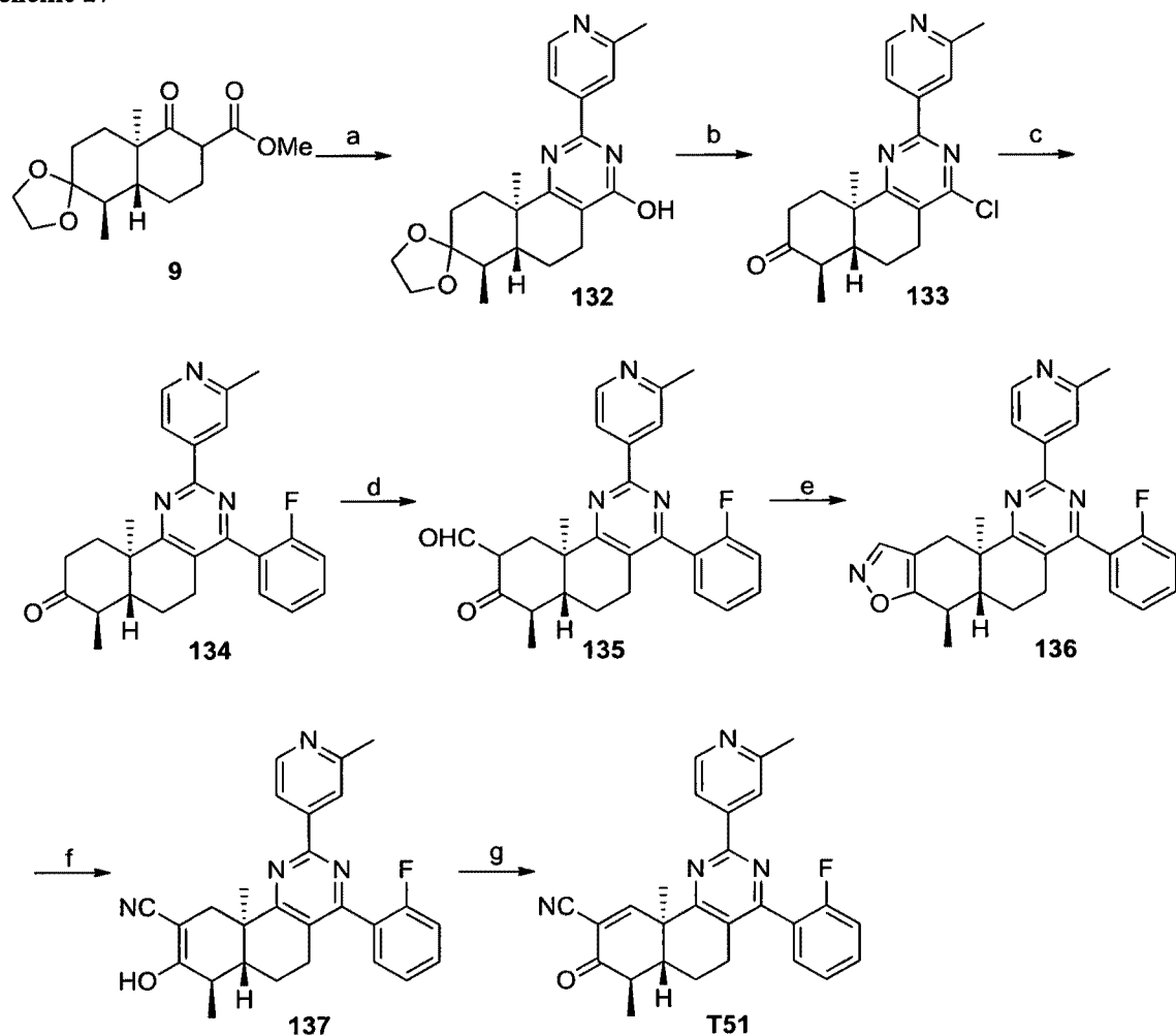
Scheme 27
