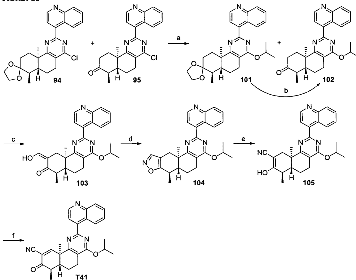
Scheme 21
