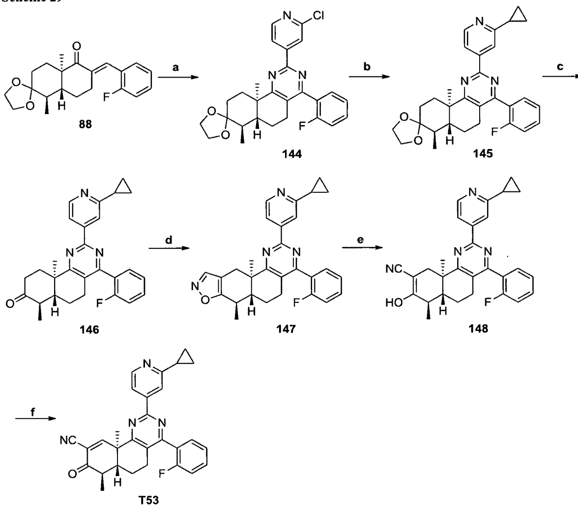
Scheme 29
