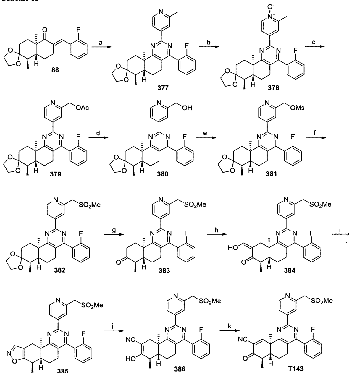
Scheme 85
