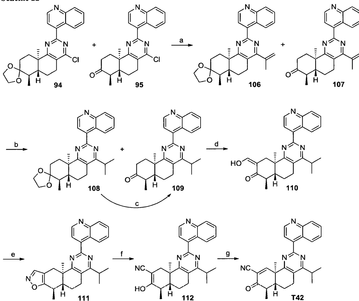
Scheme 22
