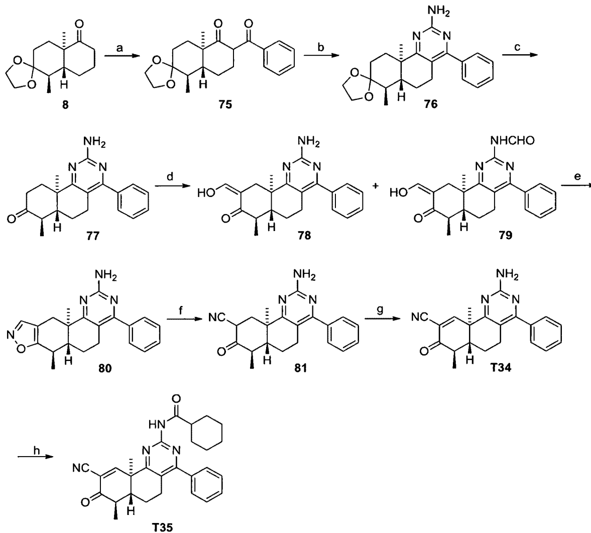
Scheme 16
