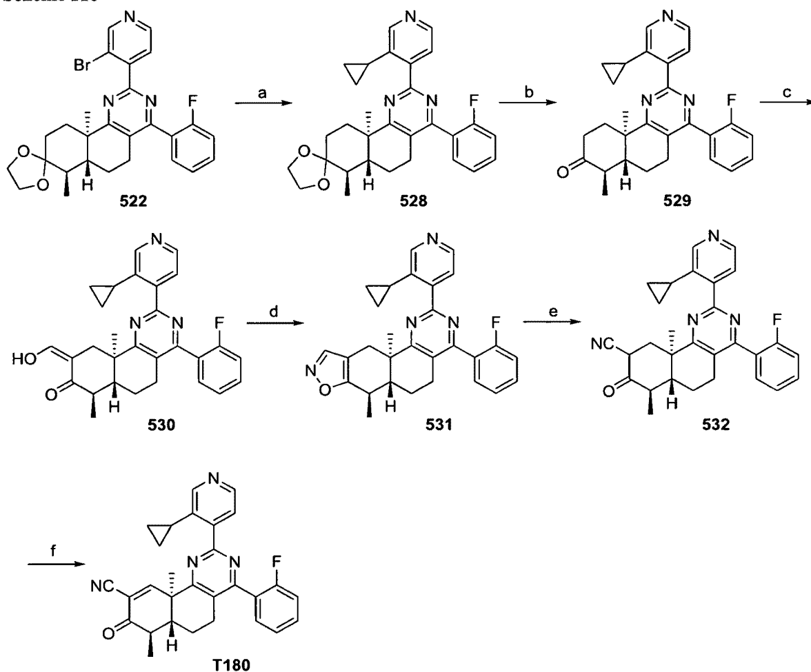
Scheme 110
