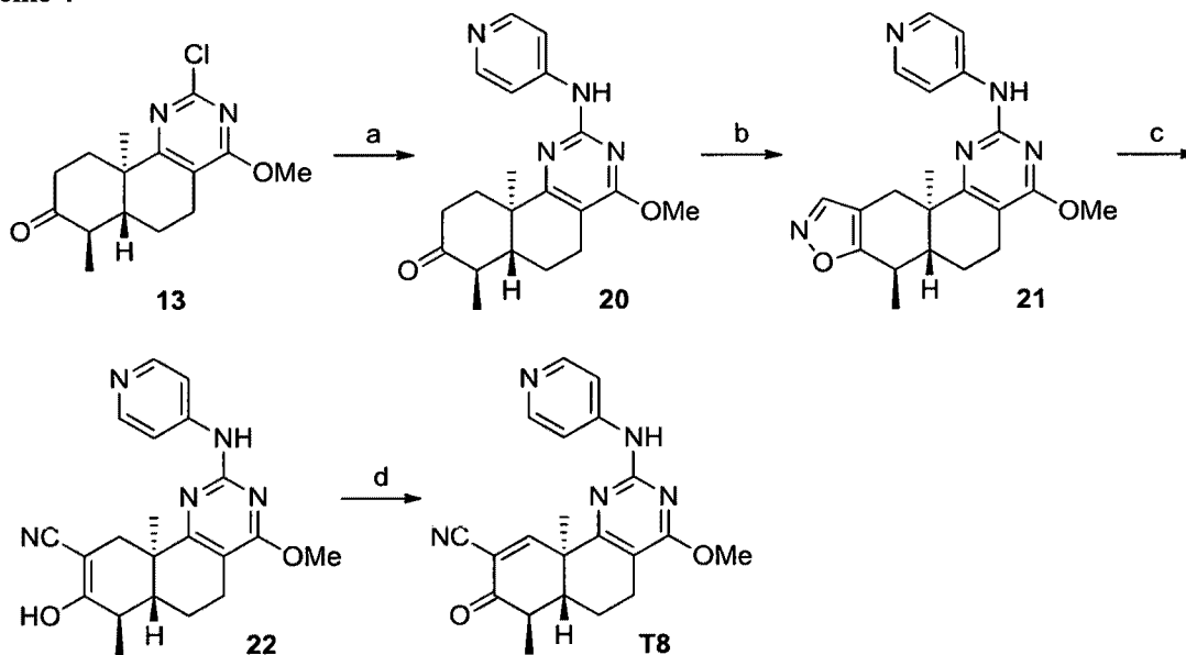
Scheme 4
