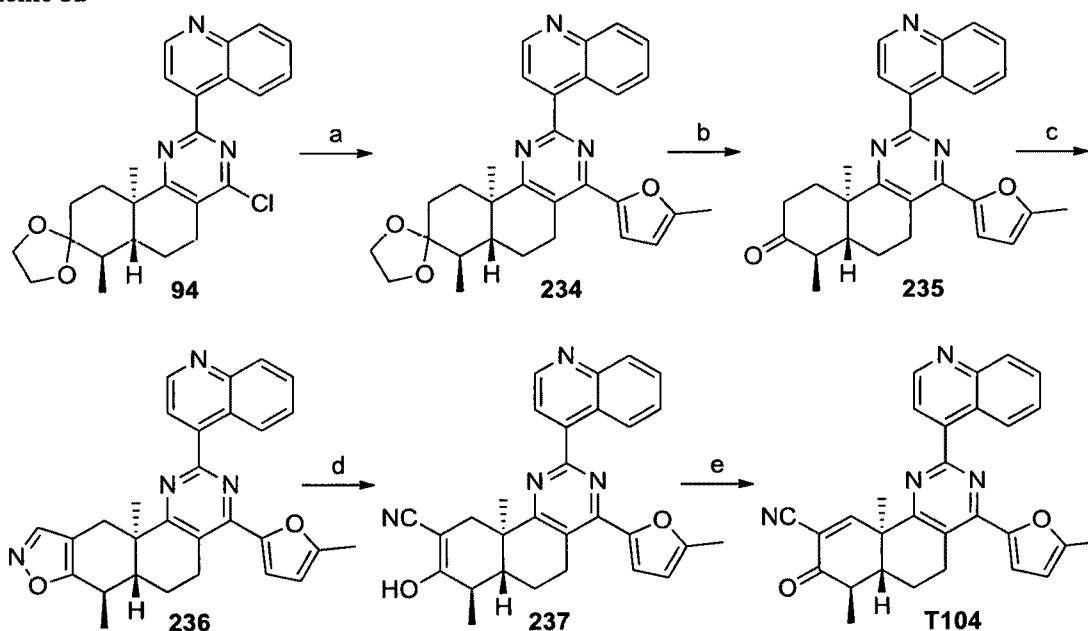
Scheme 52
