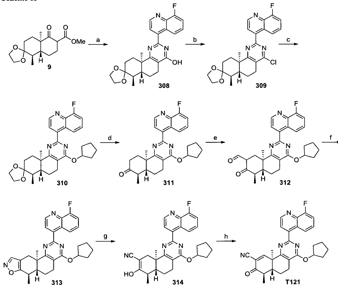
Scheme 65
