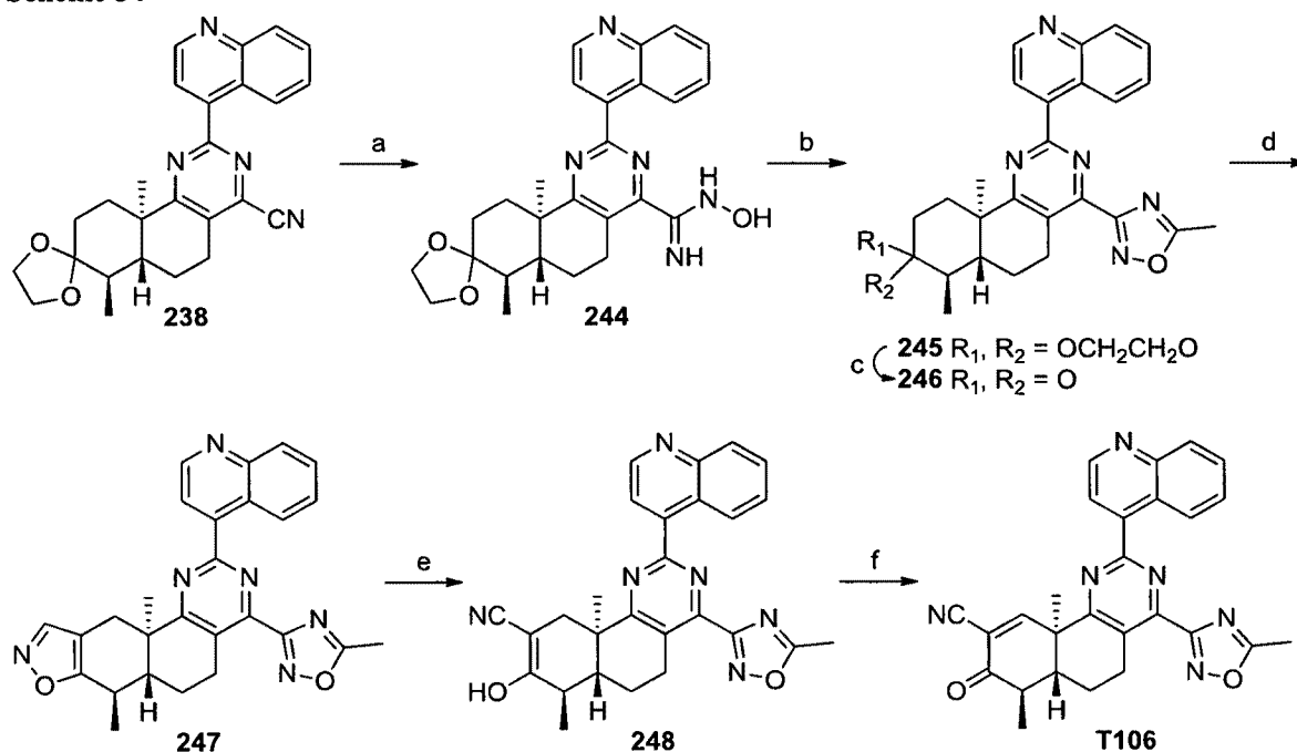
Scheme 54
