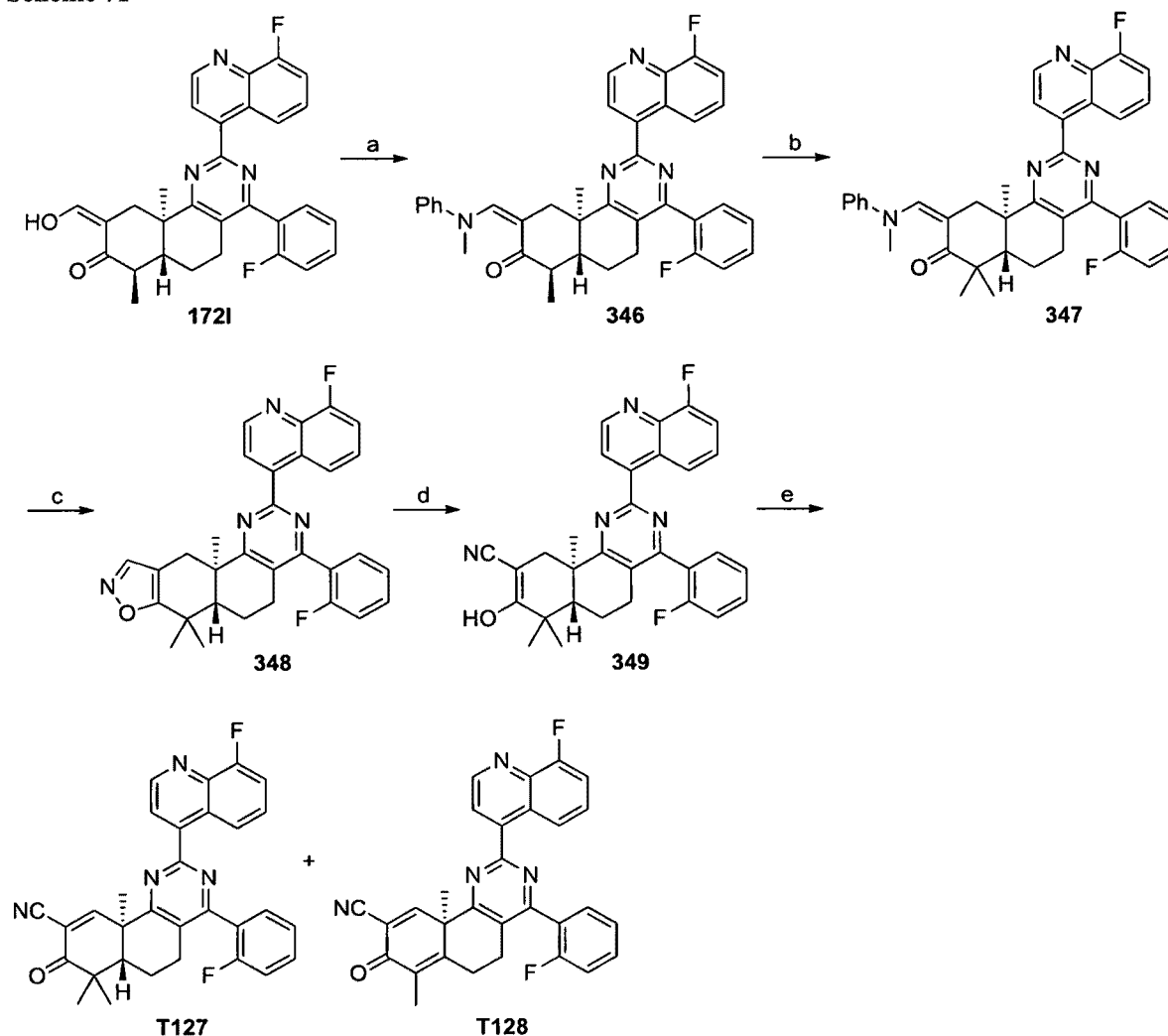
Scheme 71
