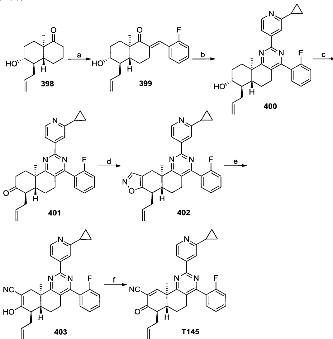
Scheme 88
