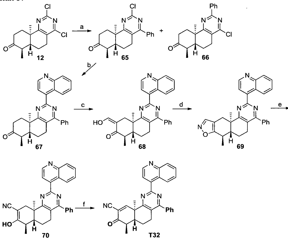
Scheme 14
