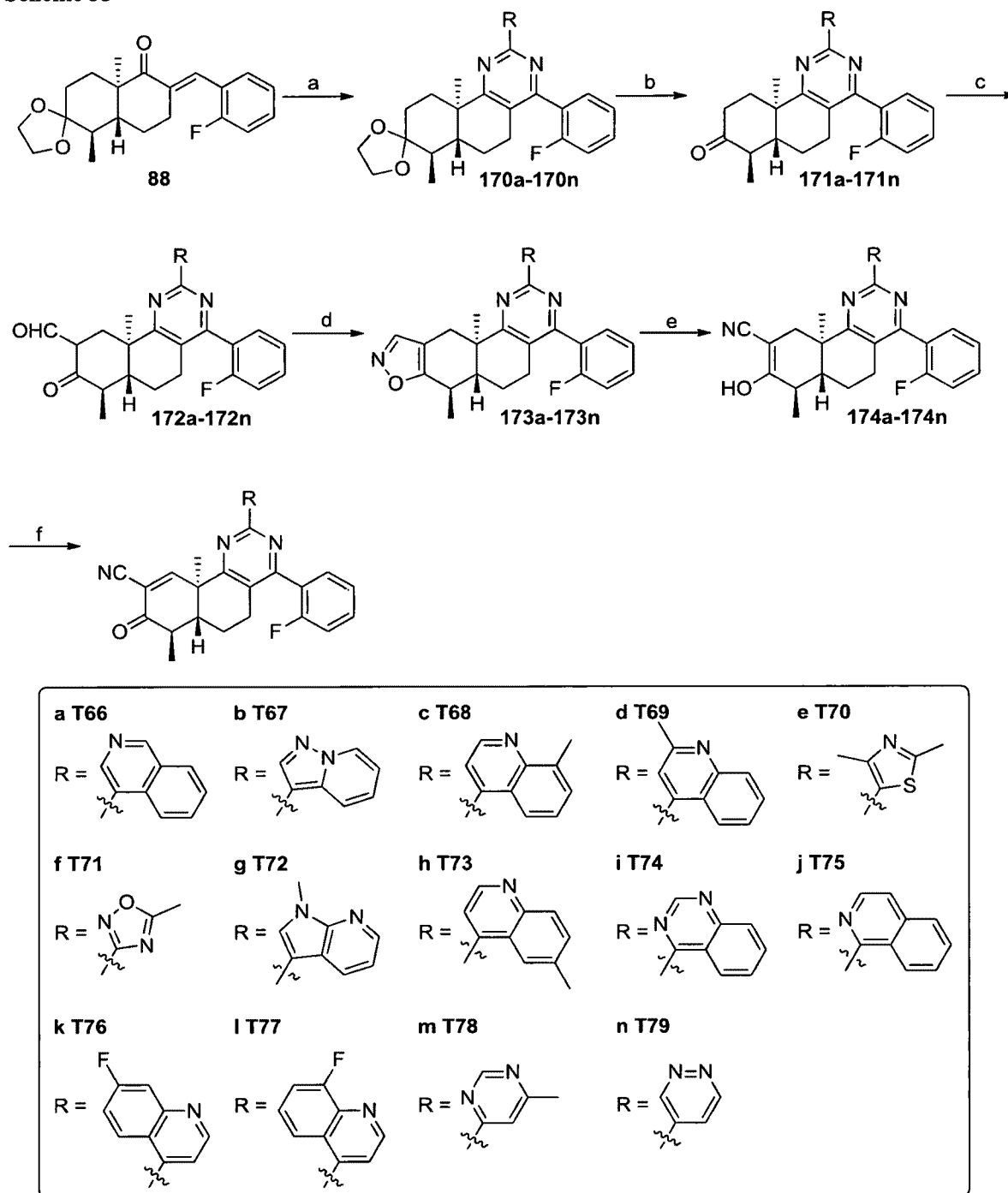
Scheme 35
