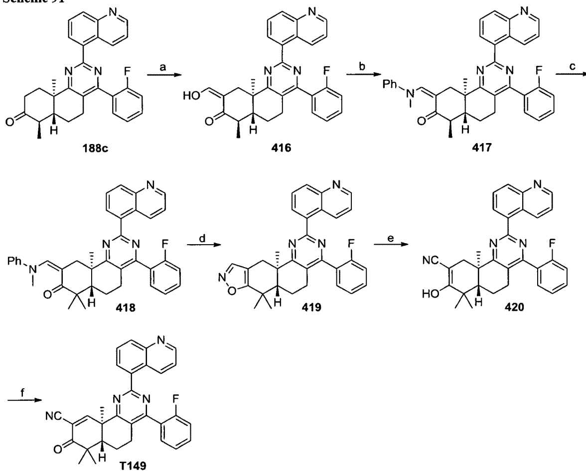
Scheme 91
