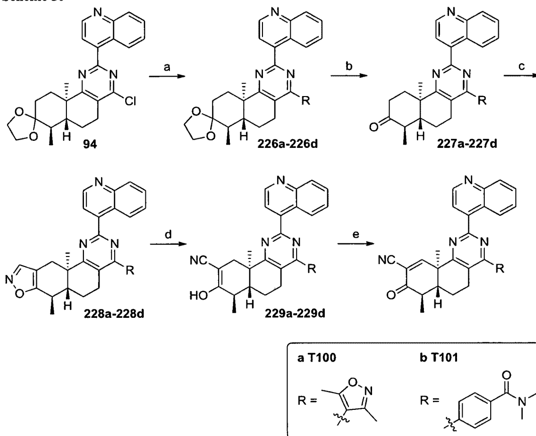
Scheme 50
