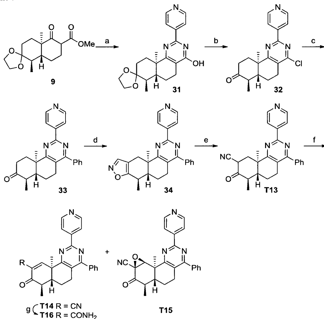
Scheme 7
