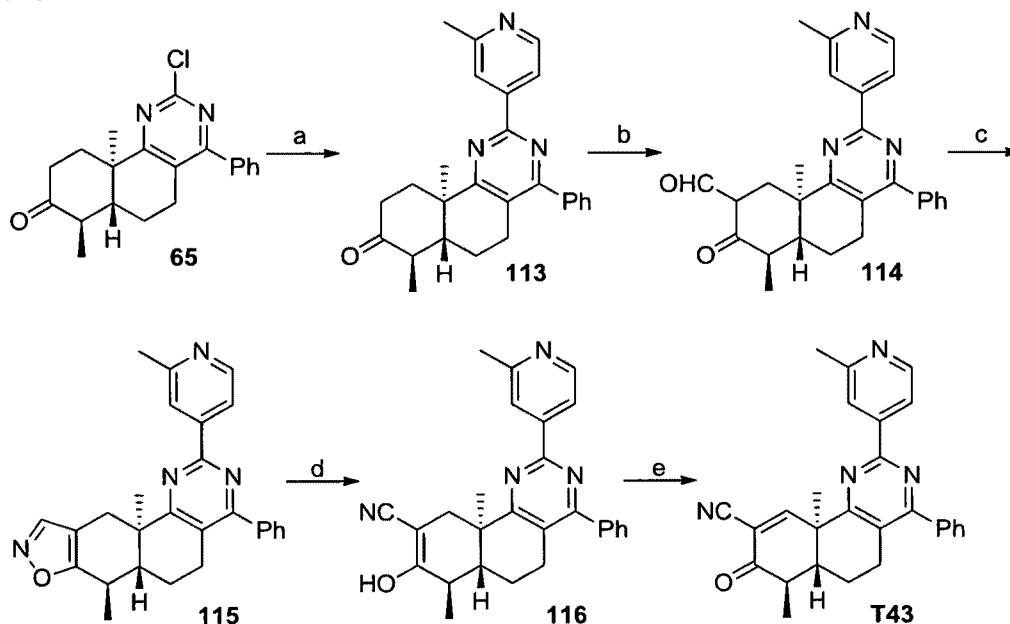
Scheme 23
