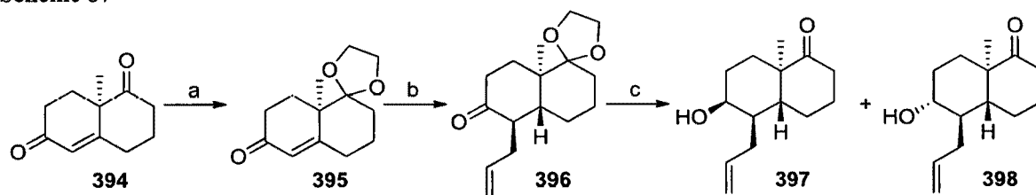
Scheme 87
