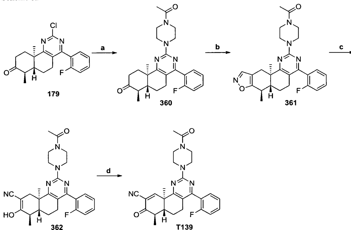
Scheme 81
