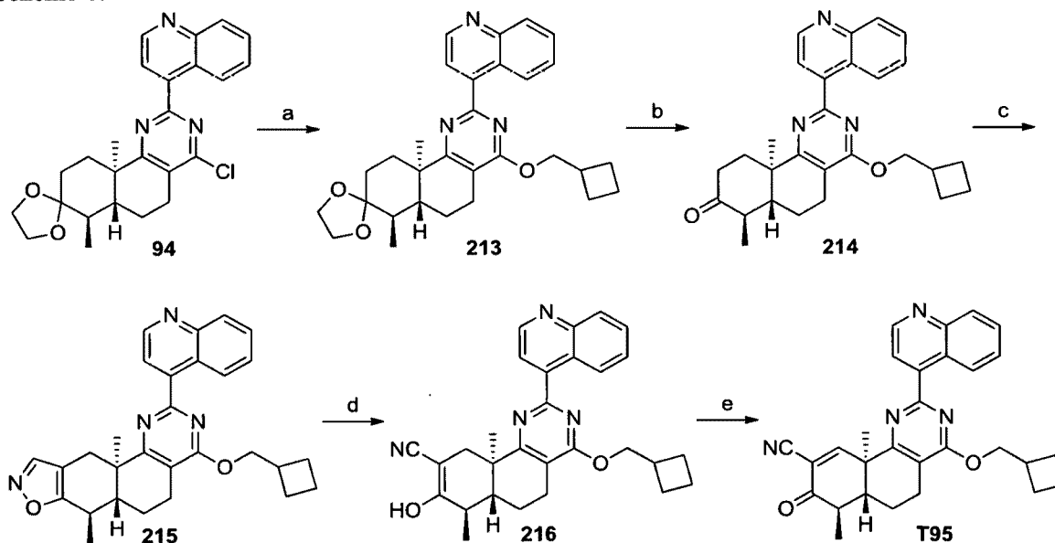
Scheme 47
