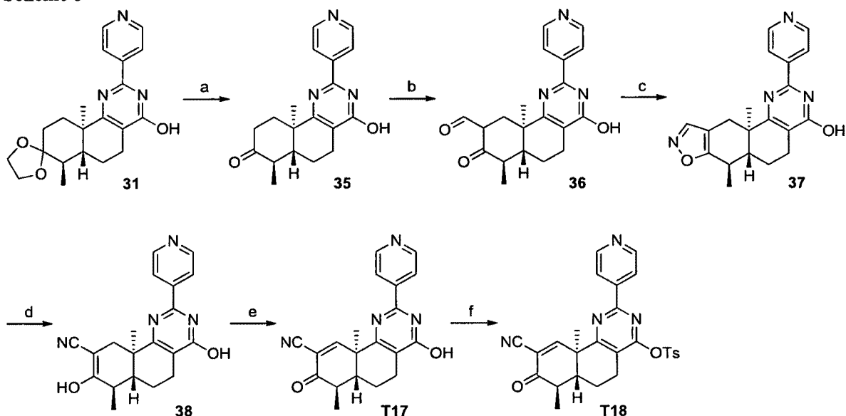
Scheme 8
