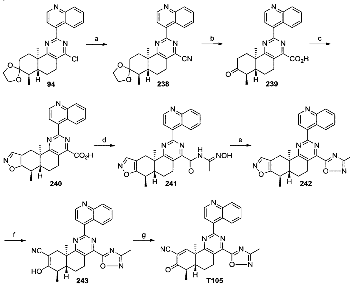
Scheme 53
