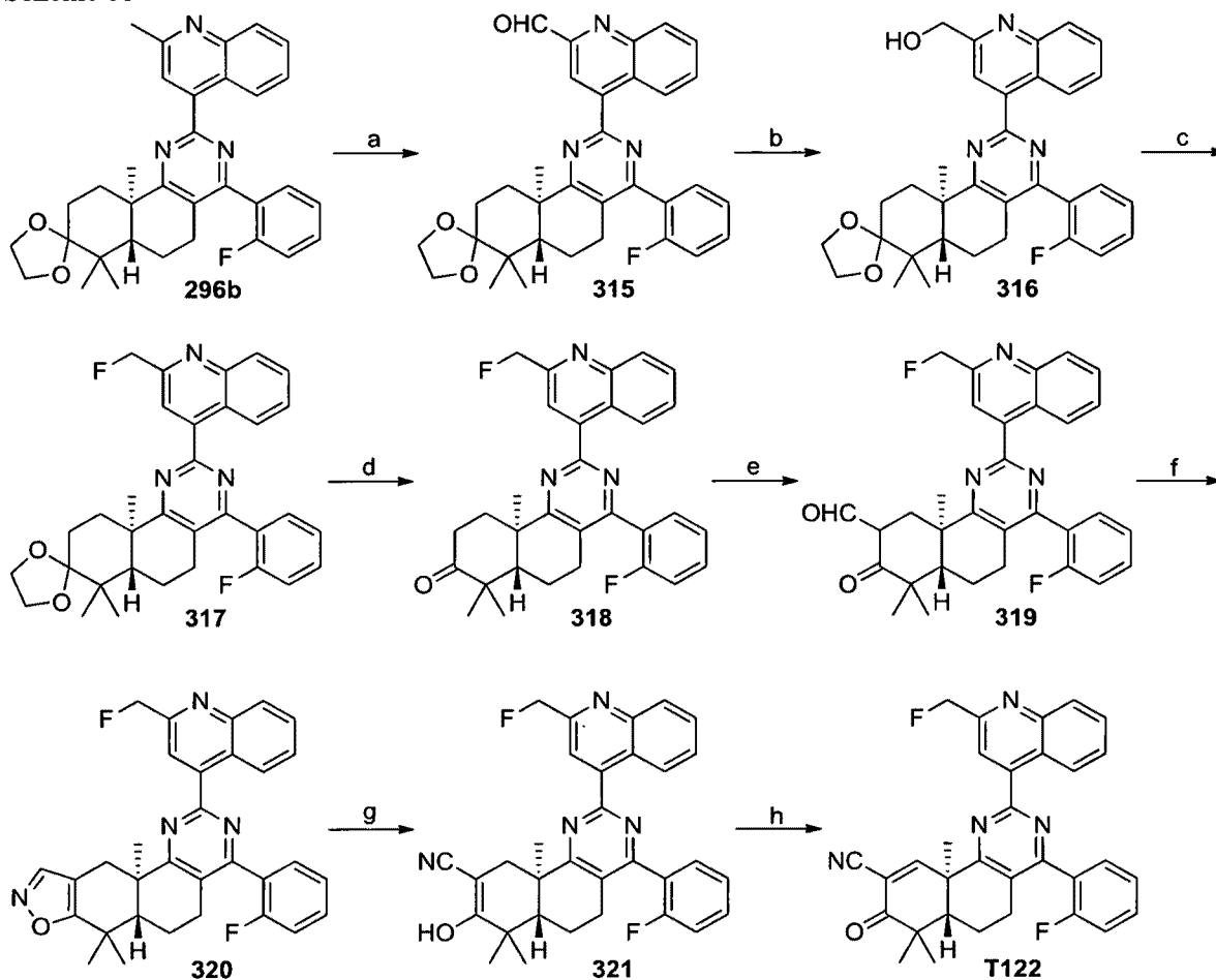
Scheme 66
