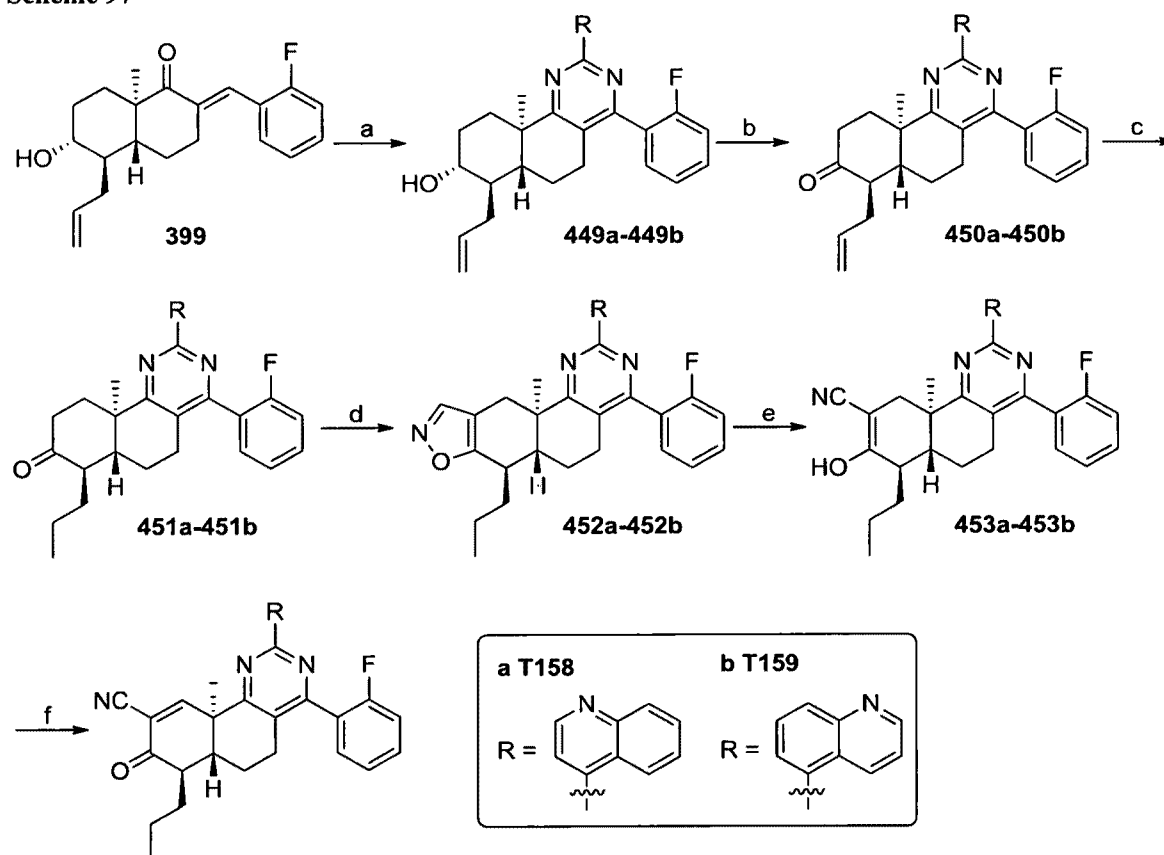
Scheme 97
