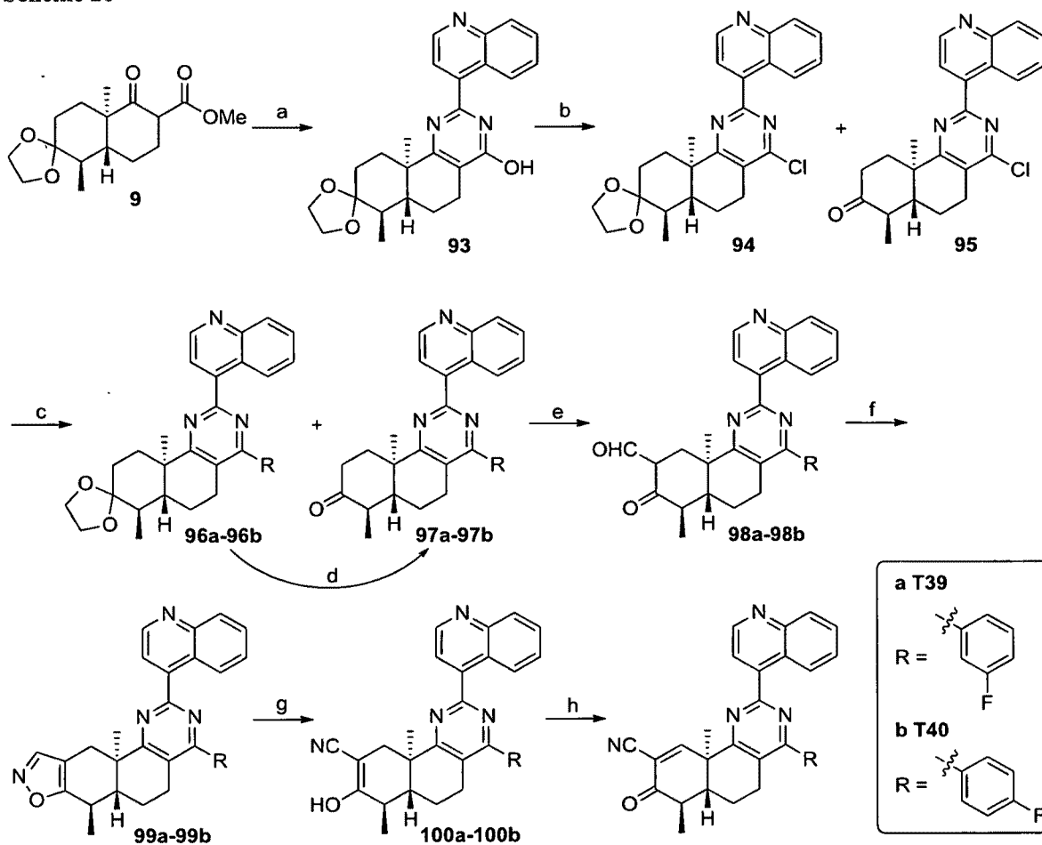
Scheme 20
