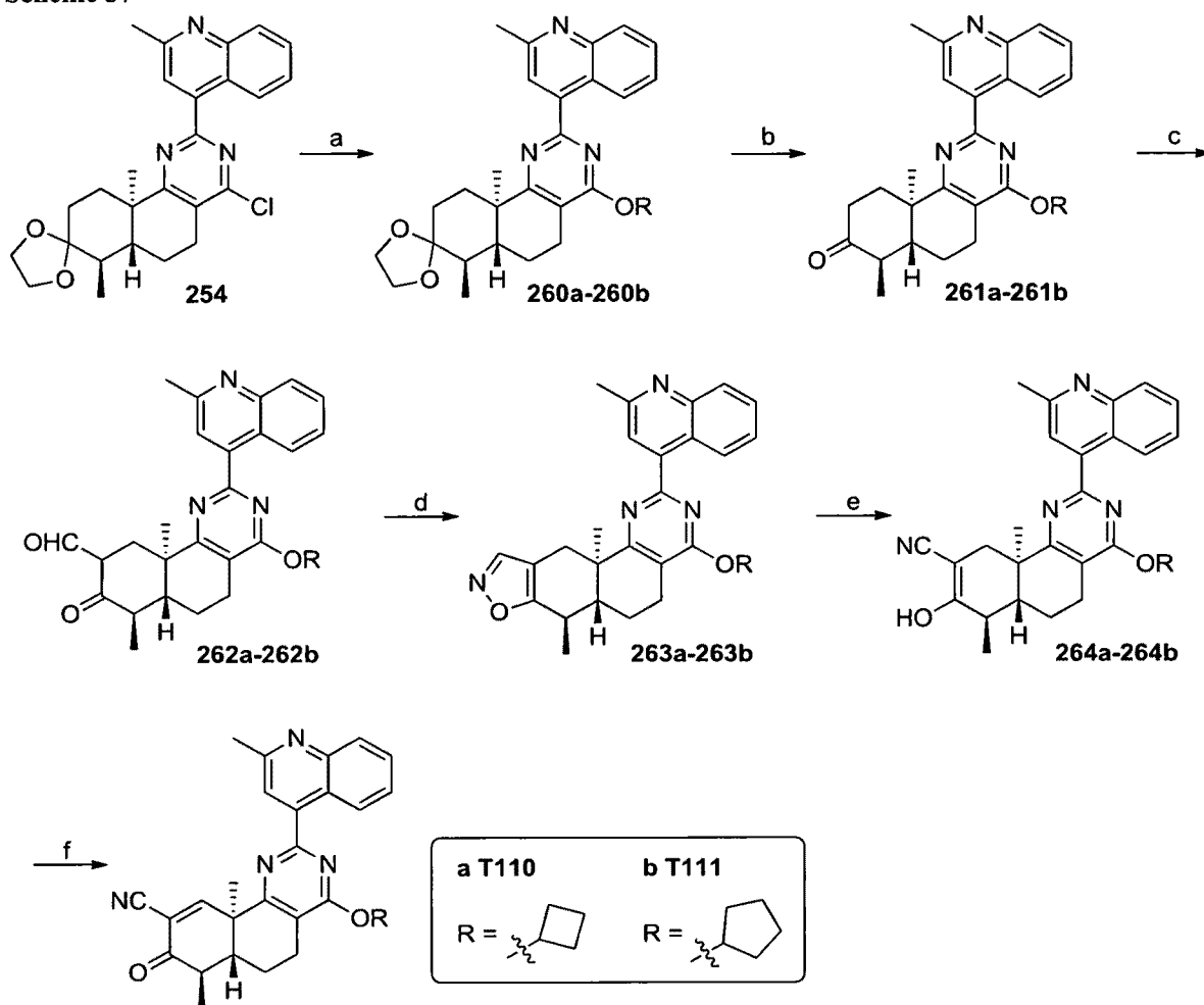
Scheme 57
