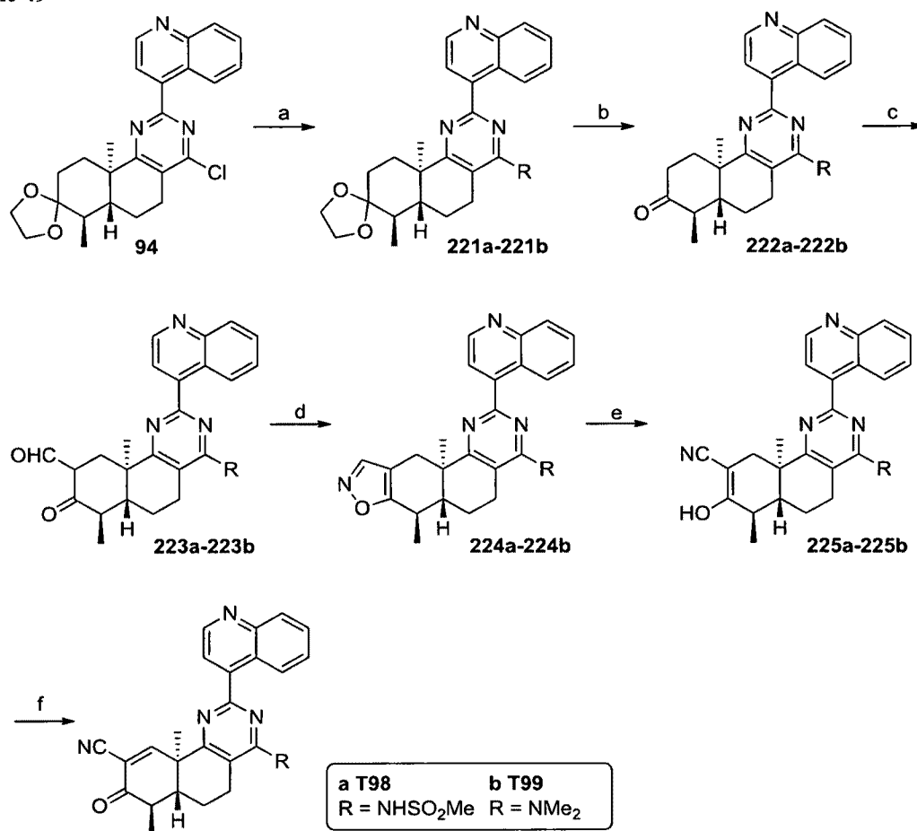
Scheme 49
