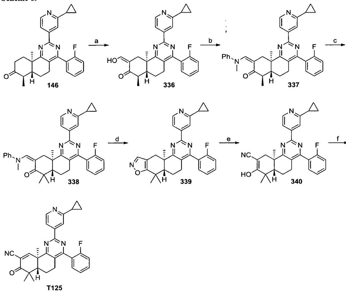
Scheme 69
