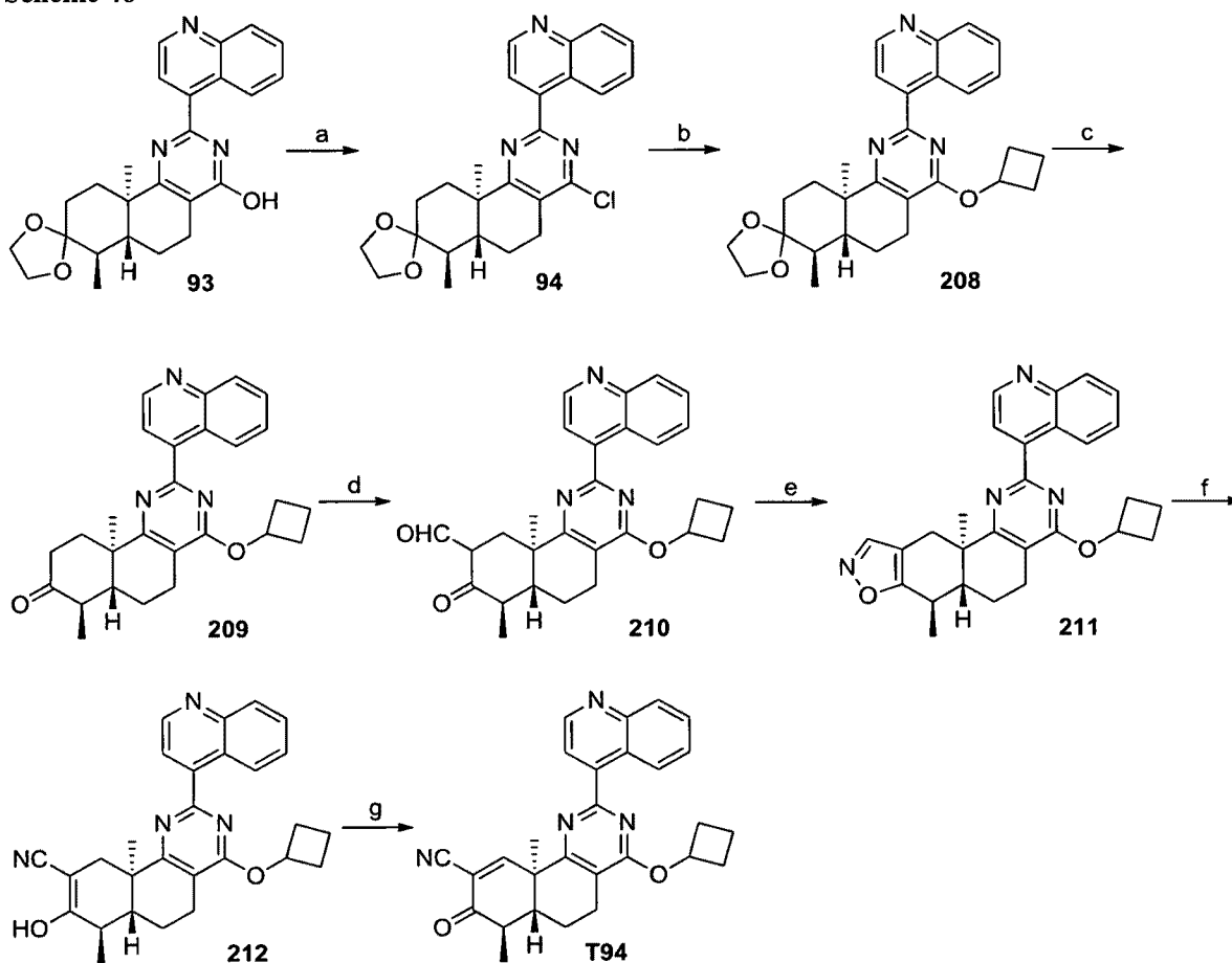
Scheme 46
