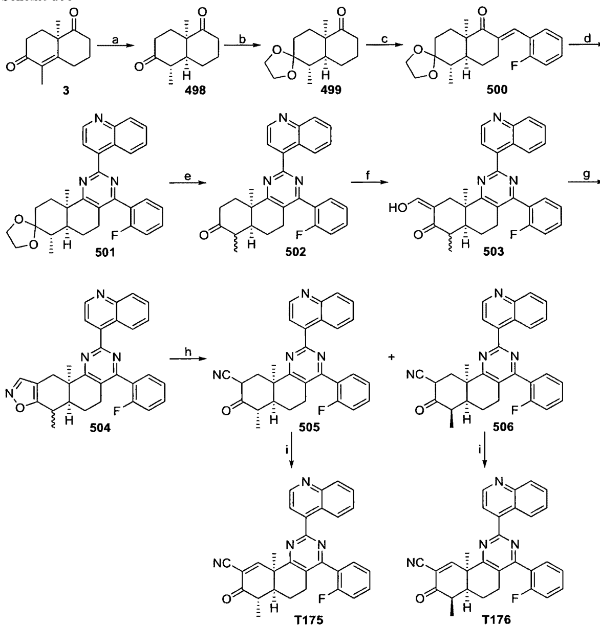
Scheme 106
