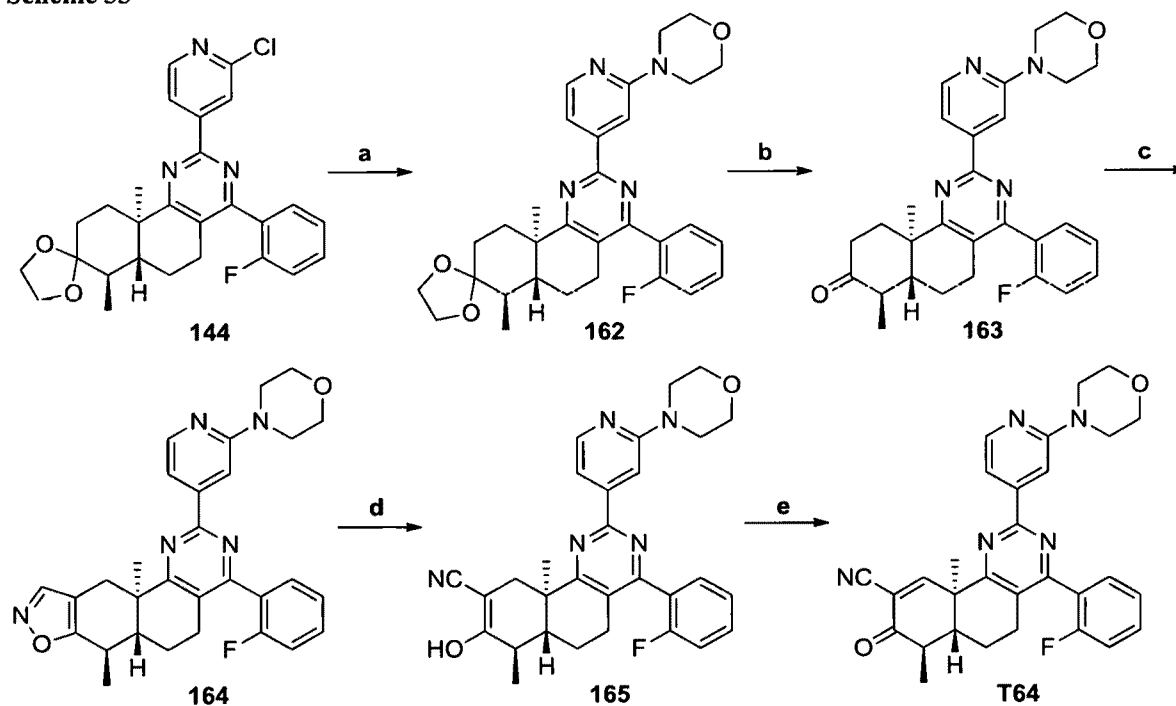
Scheme 33
