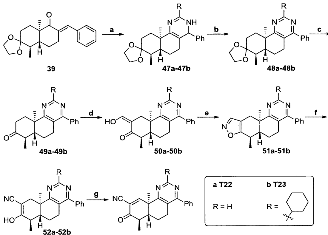
5 Scheme 11
