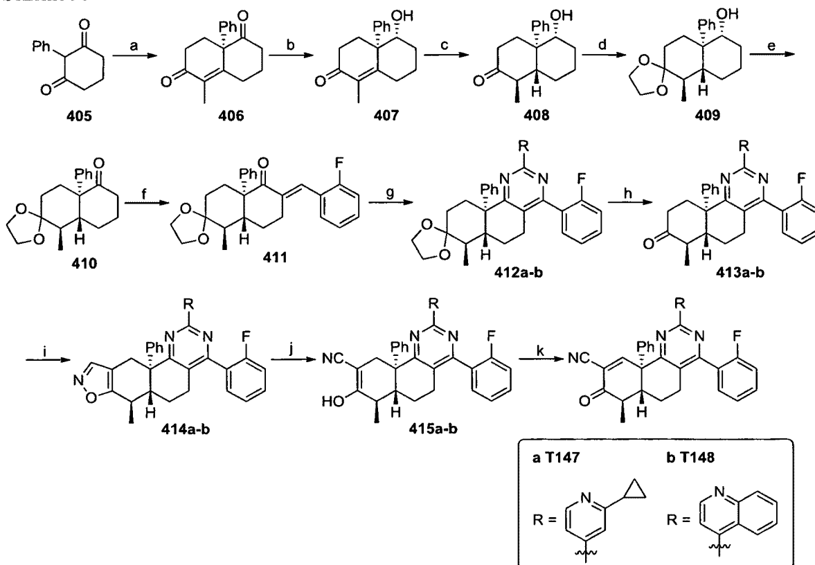
Scheme 90
