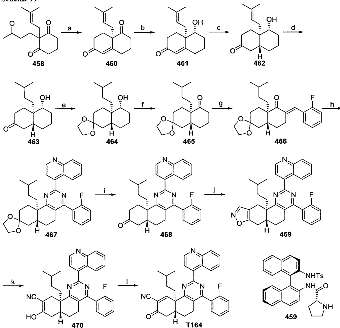
Scheme 99
