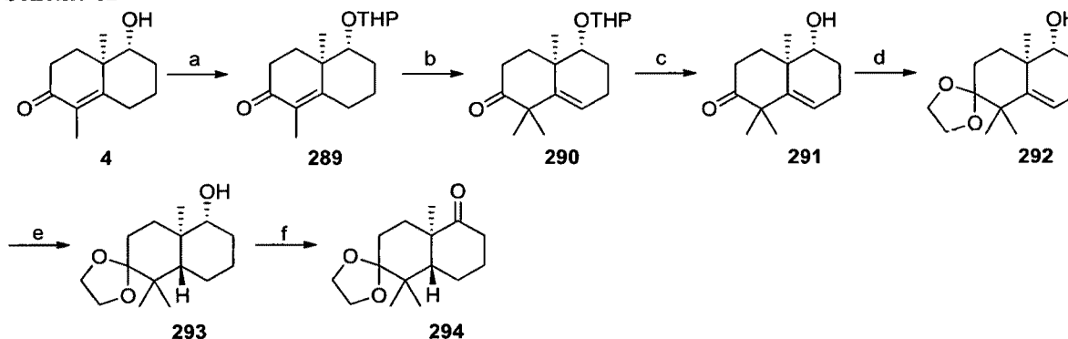
Scheme 62
