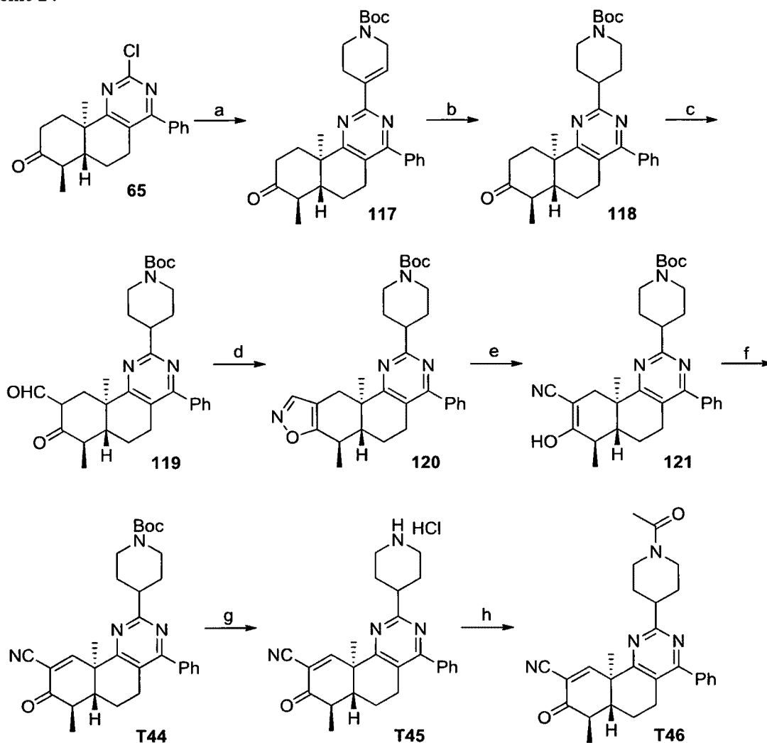
Scheme 24
