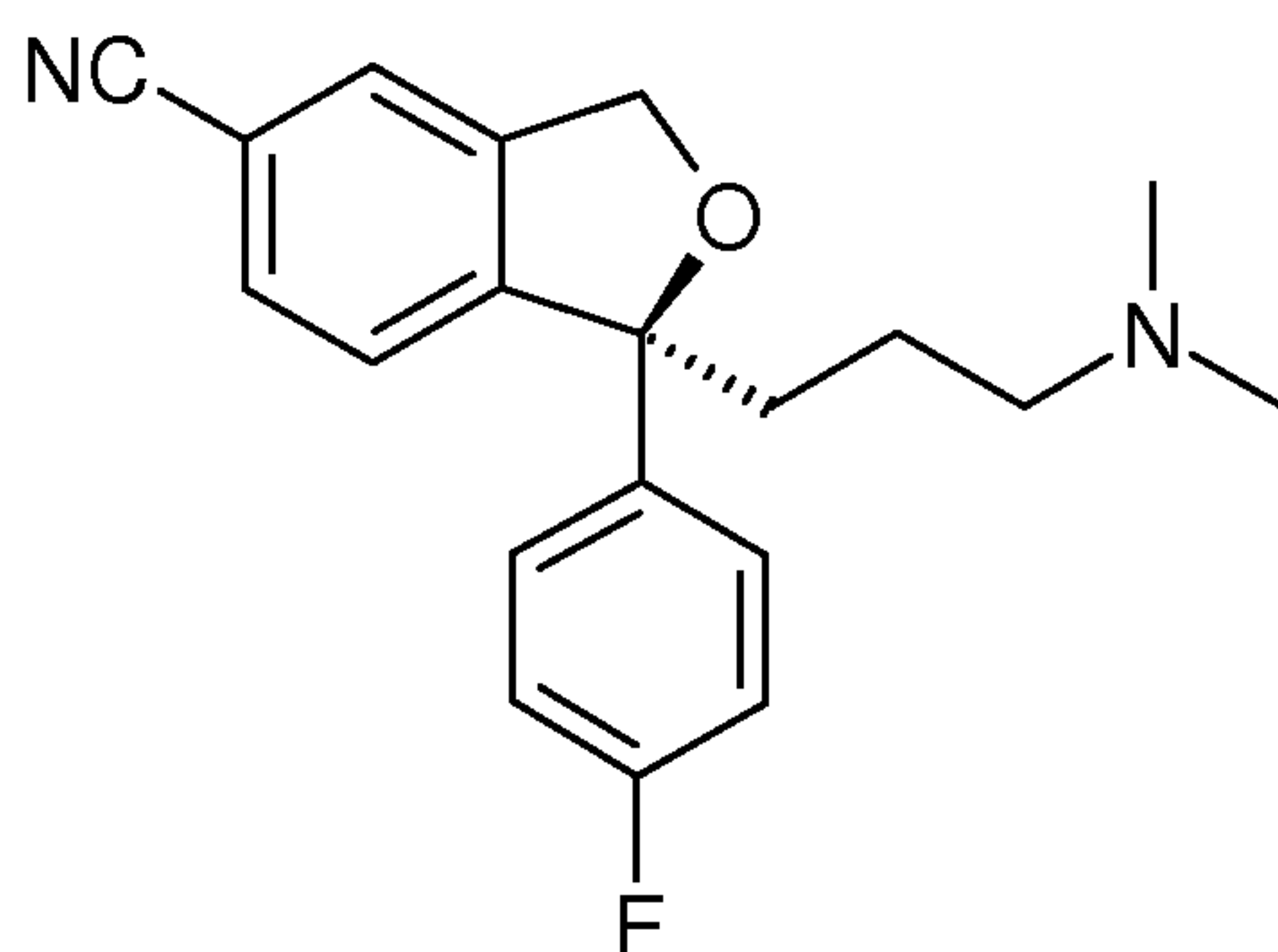
Formula I
