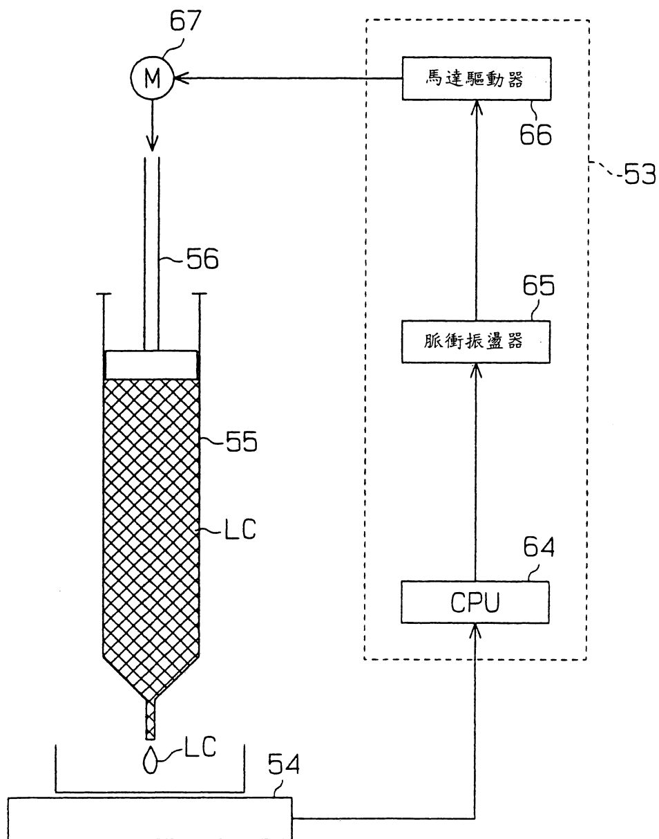
滴下計測部之概略說明圖
