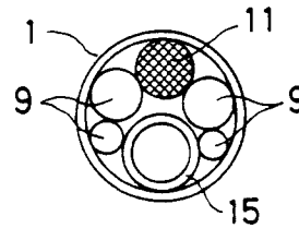
FIG. 3 PRIOR ART
