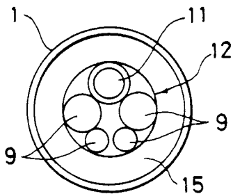
FIG. 4 PRIOR ART
