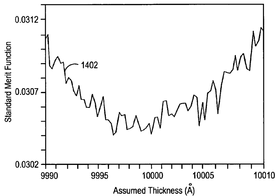
FIG. 14 (PRIOR ART)
