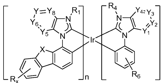
, Formula VIII.
