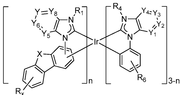
Formula VII,
