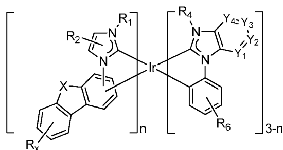
Formula V,
