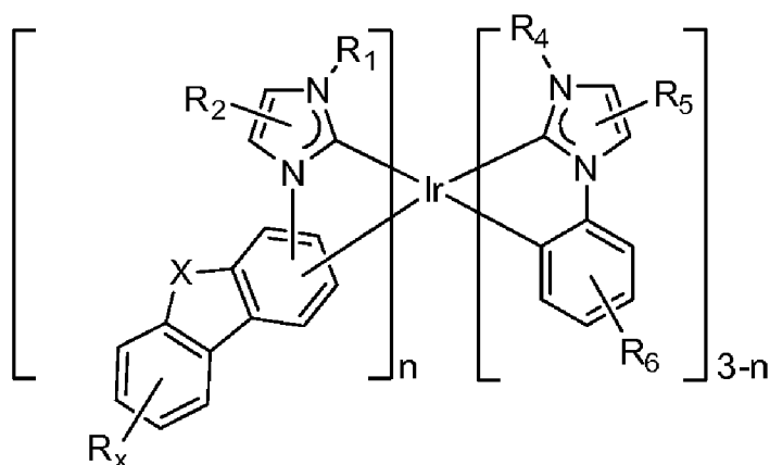
Formula I
