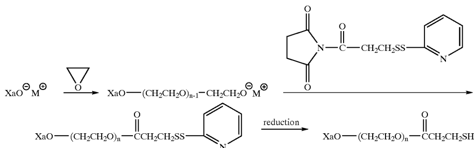
Reaction scheme 1:
