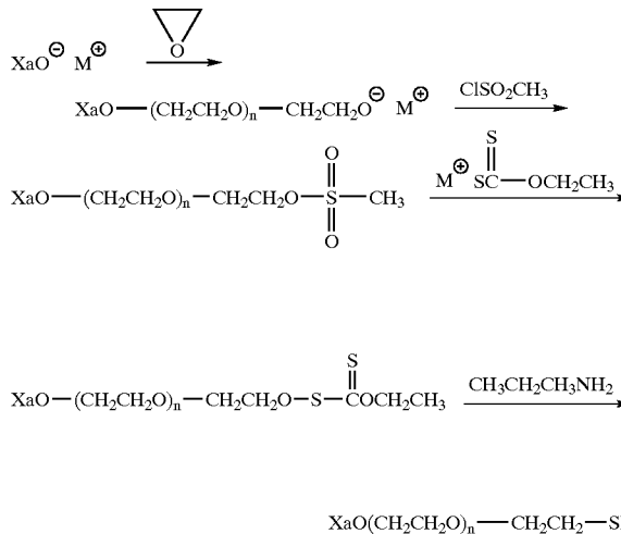
Reaction scheme 2:
