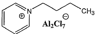
1-Butyl-pyridinium heptachloroaluminate
