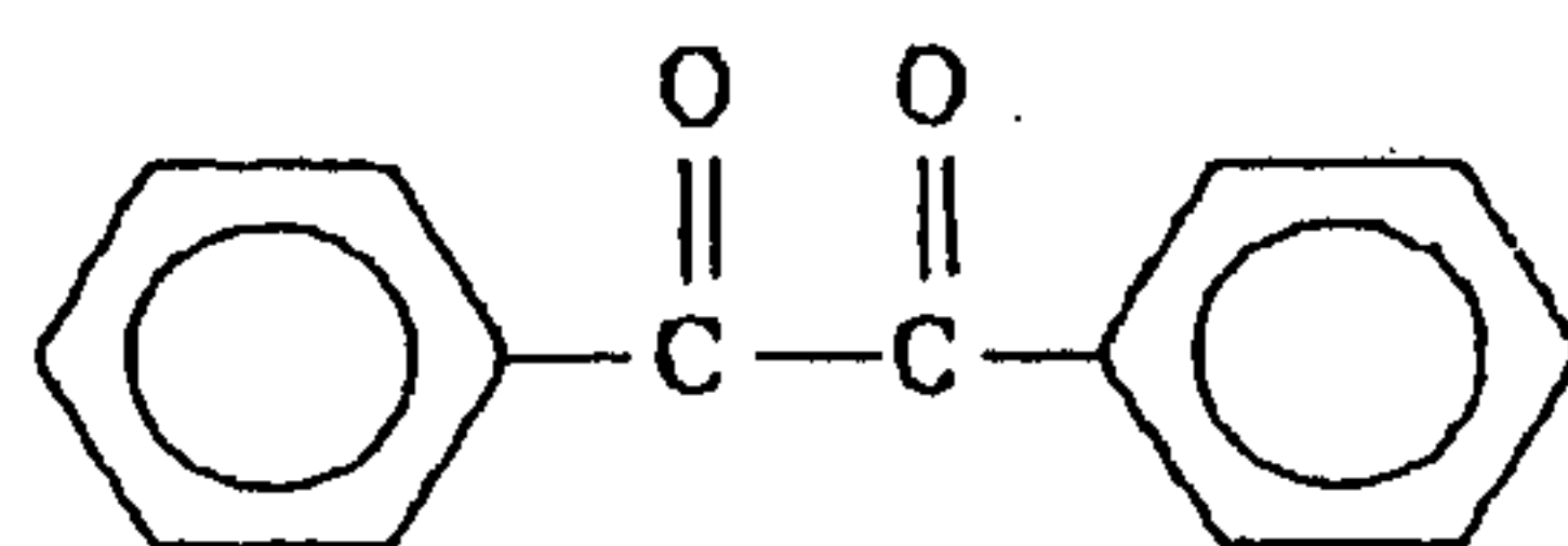
Benzyl
