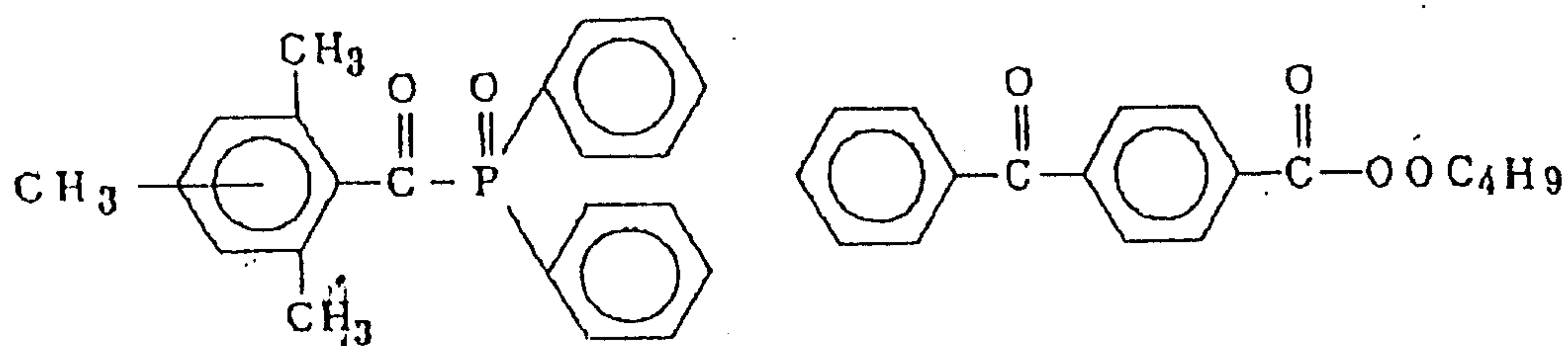
Acylphosphine oxide
