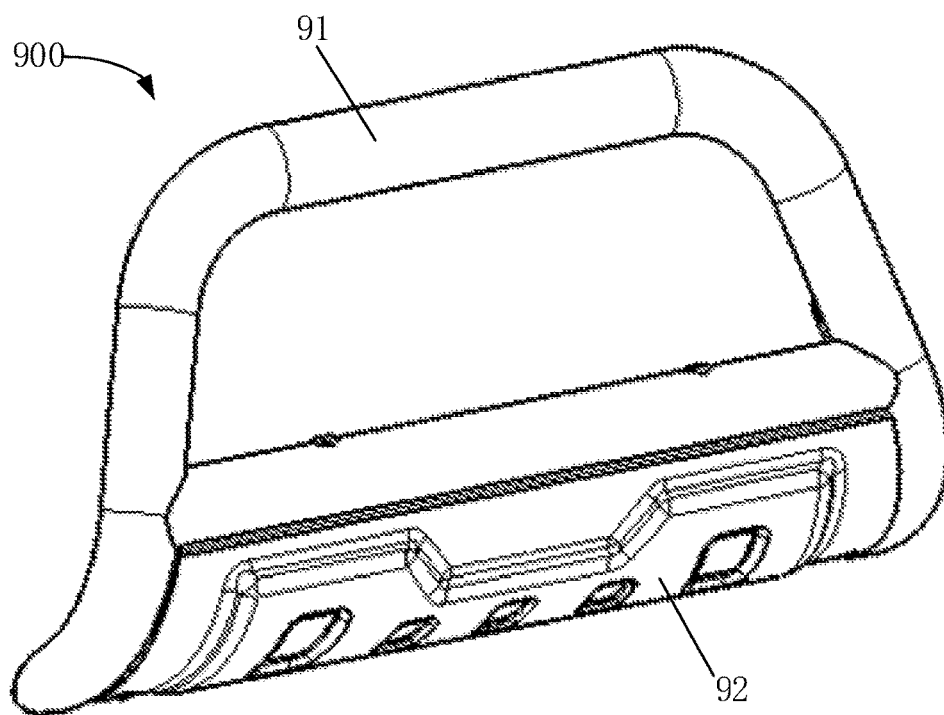
FIG. 1 (RELATED ART)
