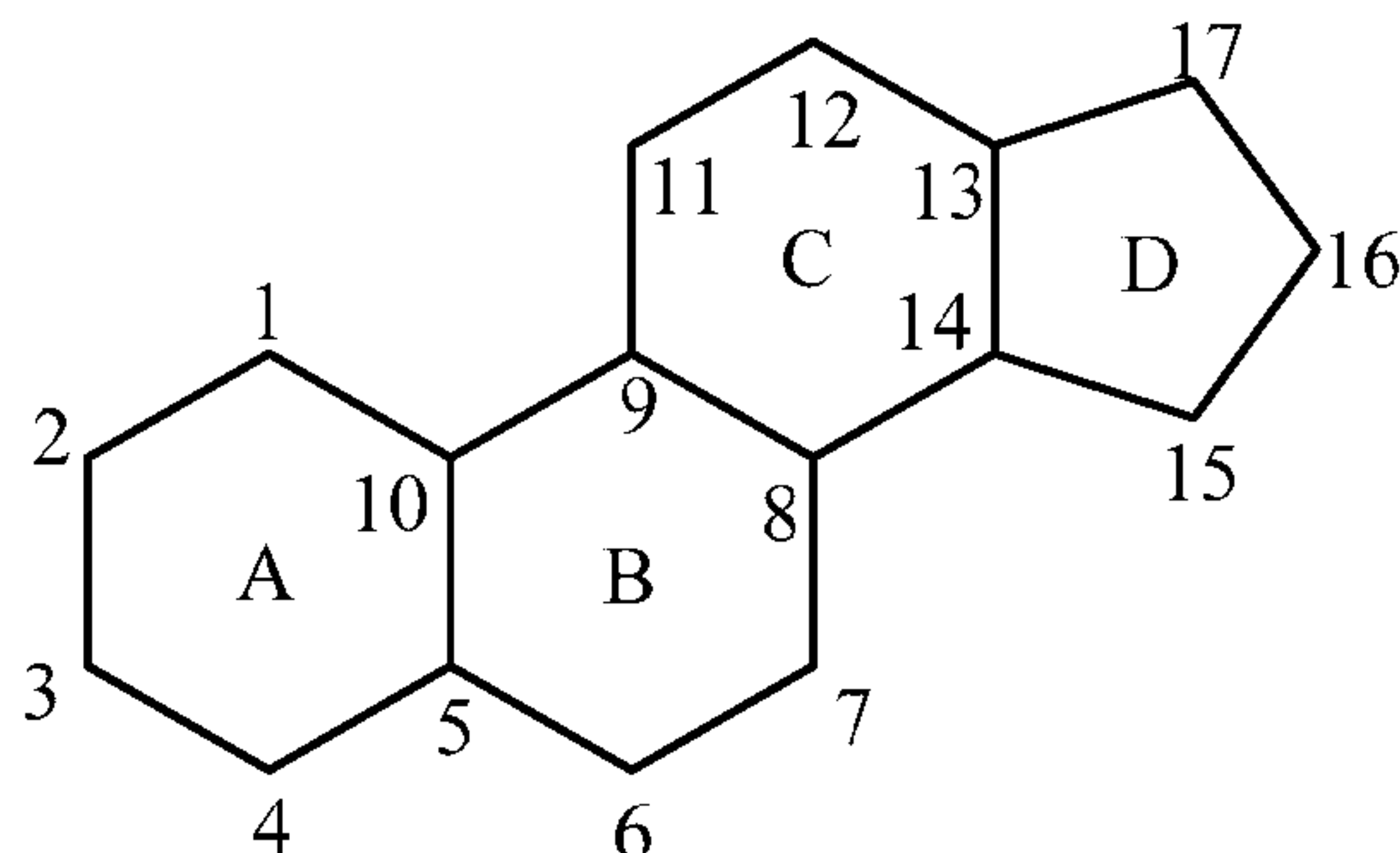
Formula I: Steroidal Backbone
