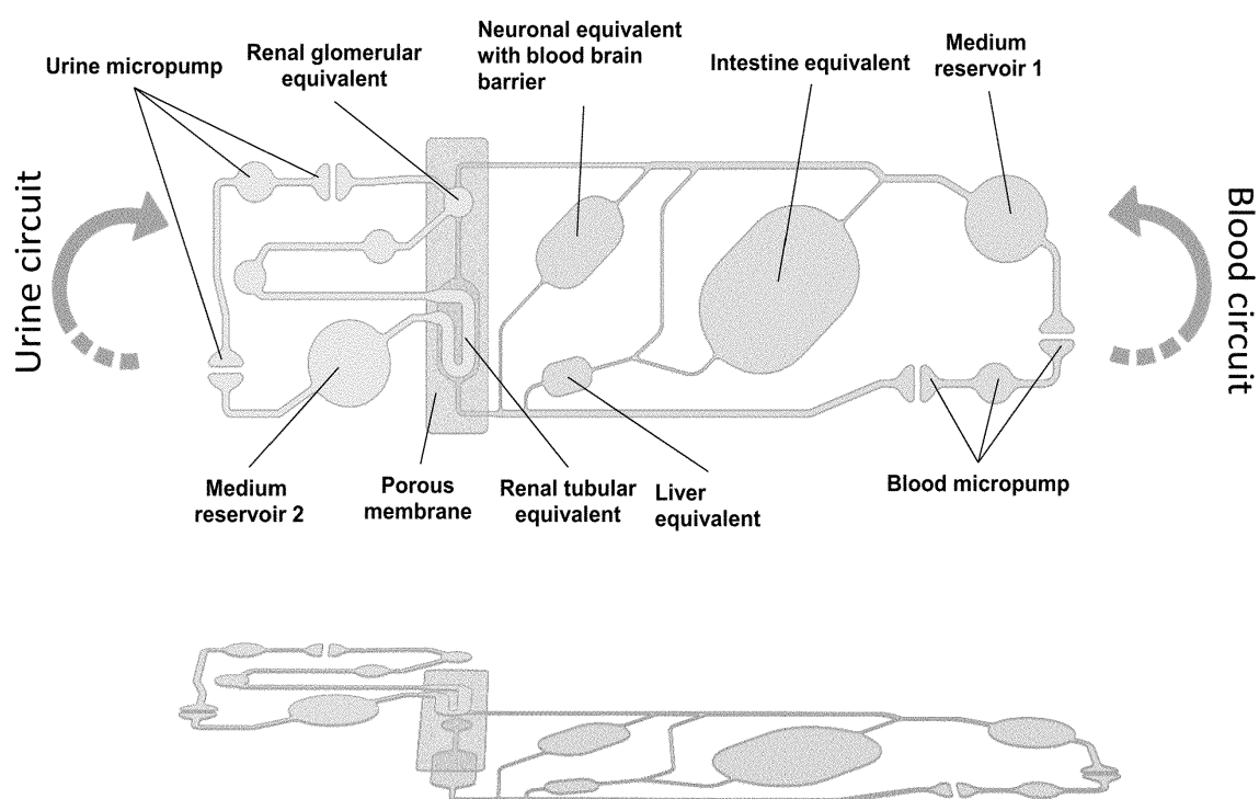
Fig. 1: Exemplary ADME-N chip footprint (top) and isometrical view on separate layers (bottom) exemplifying the positioning of a membrane between the two circuits.
