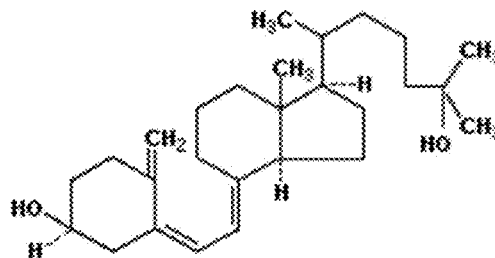
25 Hydroxyvitamin D-3
