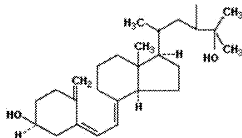
25 Hydroxyvitamin D-2
