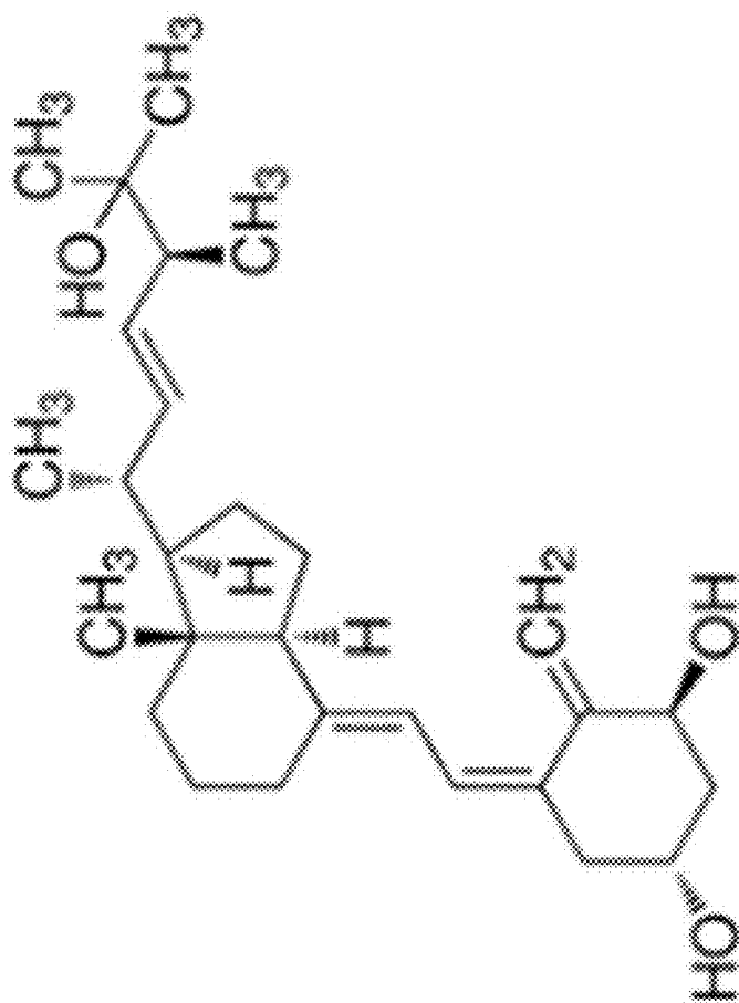
1,25-dihydroxyvitamin D2
