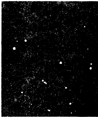
DIFFRACTION PATTERN
