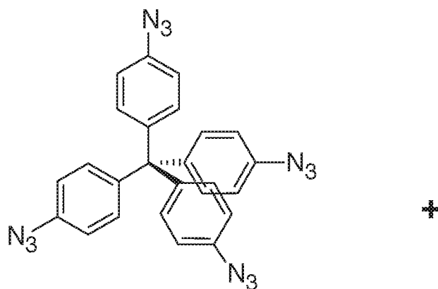
tetrakis(4-azidophenyl)methane (SM-AZ 4 ) MW = 484 g/mol
