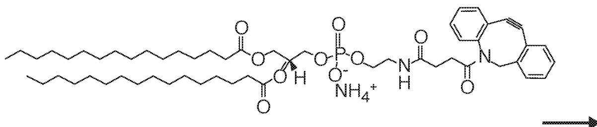
1,2-dipalmitoyl-sn-glycero-3-phosphoethanolamine-N-dibenzocyclooctyl (DBCO PL) MW = 996 g/mol
