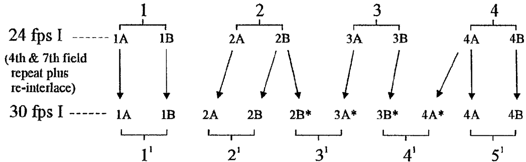
Figure 7e 4th & 7th Field Repeat plus Re-Interlace (24 fps I to 30 fps I)
