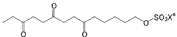
[Chem. 18]
