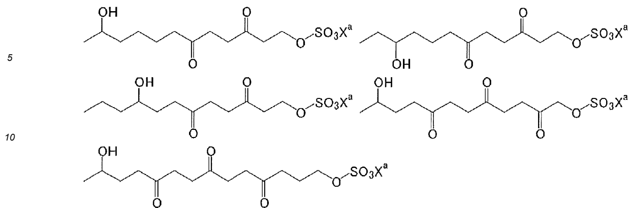
[Chem. 19]
