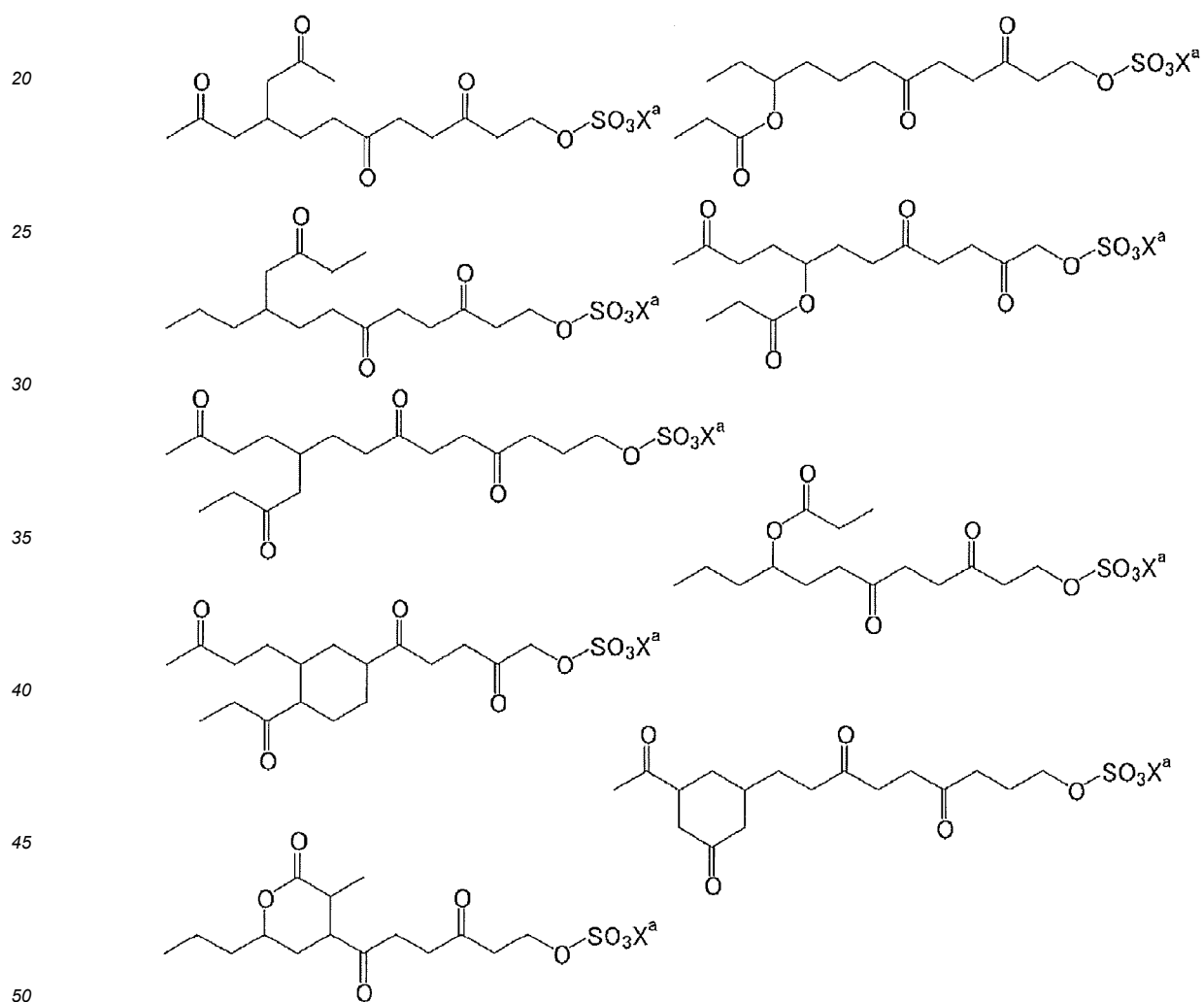
[Chem. 19]
