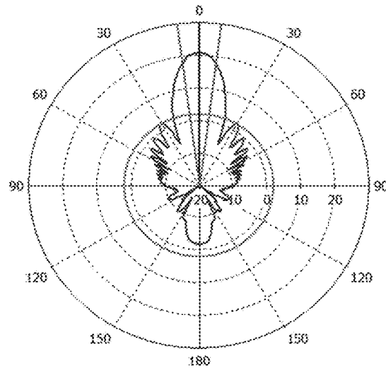
Antenna Gain Pattern
