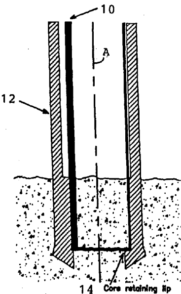
Break-off Configuration (Break-off Tube rotated 180 degrees)
