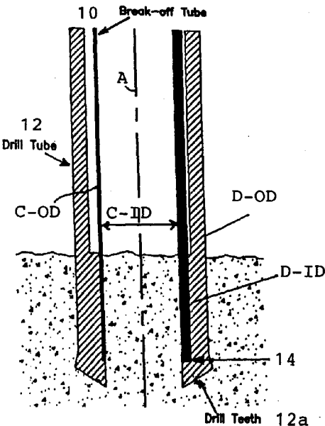
Core Drilling Configuration
