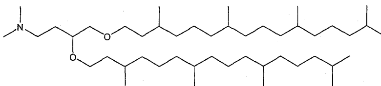
C2-DPanDMA
