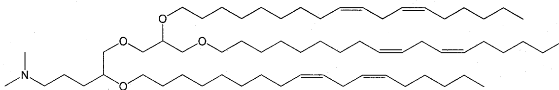
C3-TLinDMA
