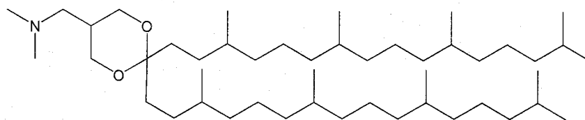
DPan-C1K6-DMA
