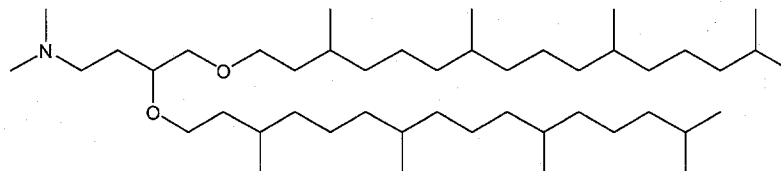
C2-DPanDMA
