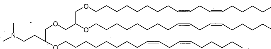
C2-TLinDMA
