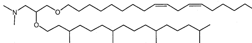
Linoleyl/Phytanyl DMA
