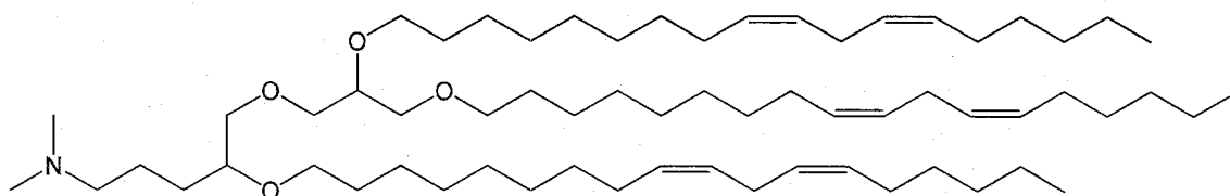
C3-TLinDMA
