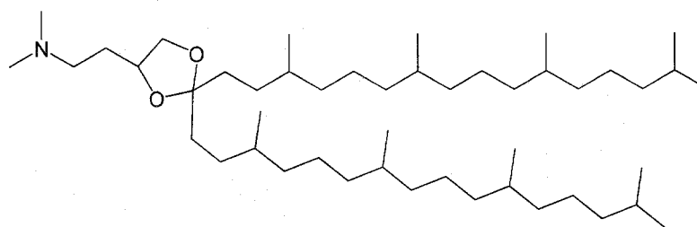
DPan-C2K-DMA
