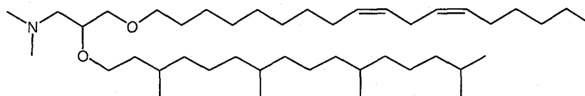
Linoleyl/Linolenyl DMA
