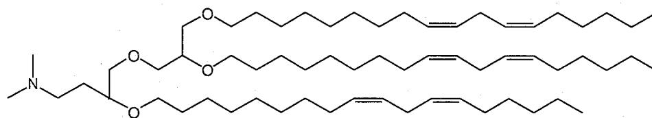
C2-TLinDMA
