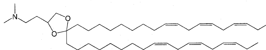
DLen-C2K-DMA
