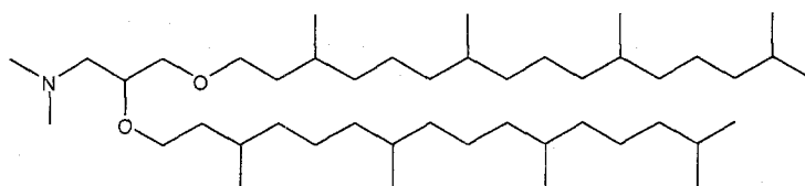
DPanDMA
