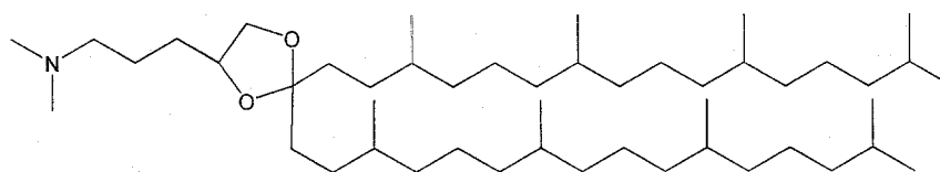
DPan-C3K-DMA
