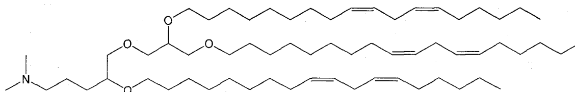
C3-TLinDMA
