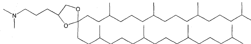
DPan-C3K-DMA
