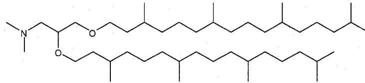
DPanDMA
