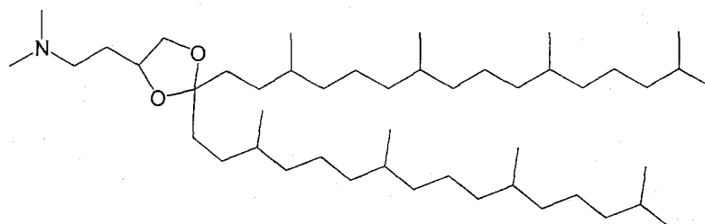
DPan-C2K-DMA
