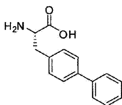
2-1-biphenyl-L-alanine (Bin)
