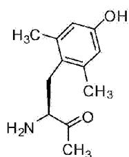
2,6-dimethyl-L-tyrosine (Dmt)
