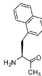
2-(1-naphthyl)-L-alanine (Nal(1))
