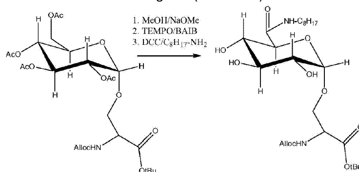
Scheme 7. Alternative example of nonionic surfactant reagent.
