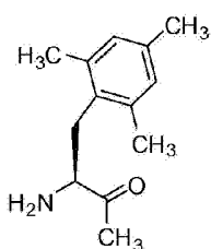
2,4,6-trimethyl-L-phenylalanine (Tmp)
