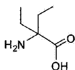
2,2-diethylglycine (Deg)
