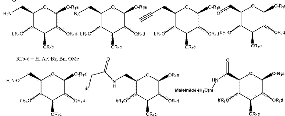
Scheme 6. Additional reagent examples.
