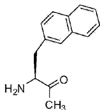
2-(2-naphthyl)-L-alanine (Nal(2))
