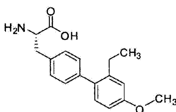
2-1-(2-ethyl-4-methoxyphenyl)-L-alanine
