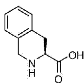
1,2,3,4-tetrahydroisoquinoline- 3-carboxylic acid (Tic)
