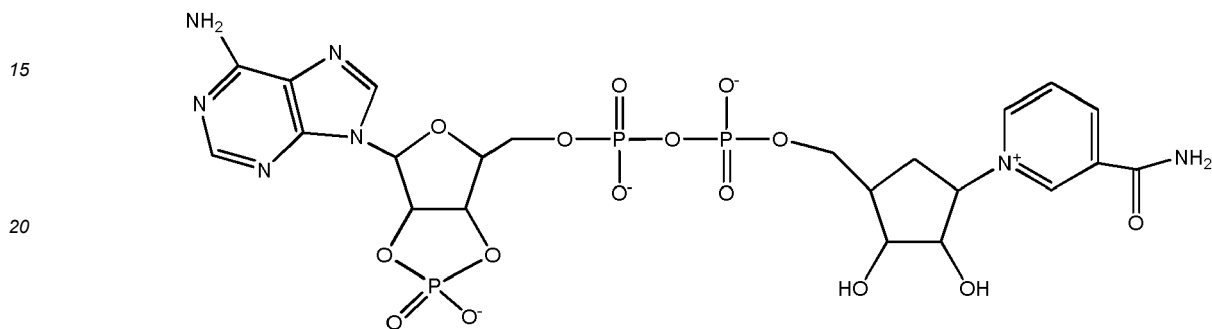
carbaNAD cyclophosphate
