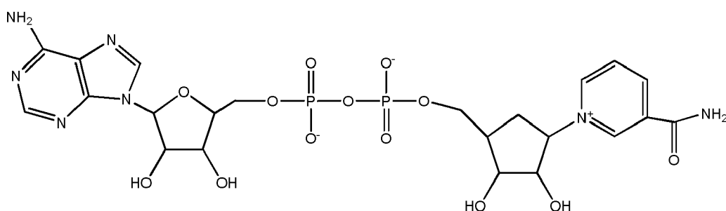
carbaNAD
