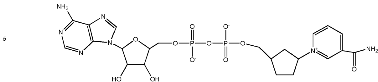
cyclopentyl NAD
