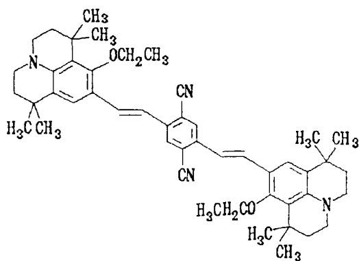
Structural Formula (1) - 2:
