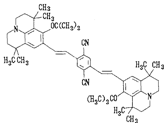
Structural Formula (1) - 3:
