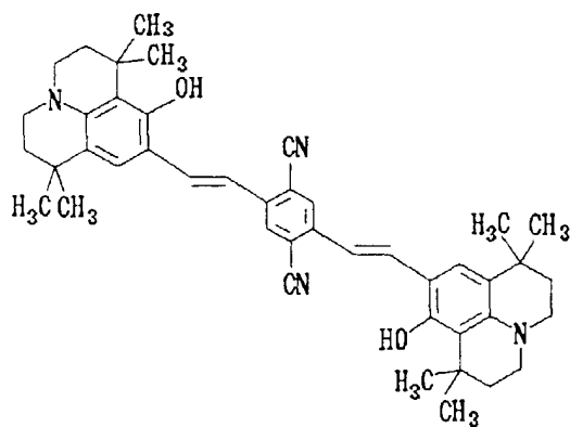
Structural Formula (1) - 6:
