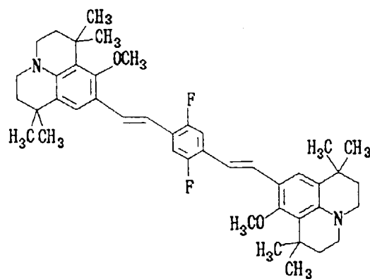
Structural Formula (1) - 7:
