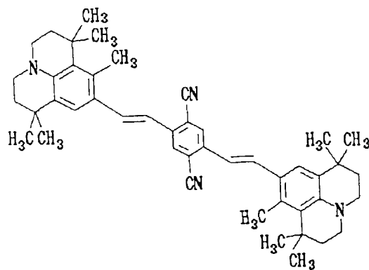
Structural Formula (1) - 4:
