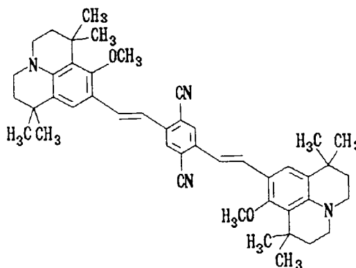
Structural Formula (1) - 1:
