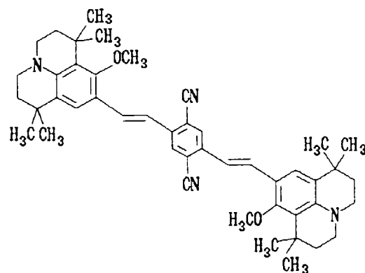
Structural Formula (1) - 1:
