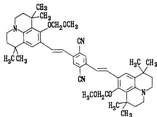
Structural Formula (1) - 8:
