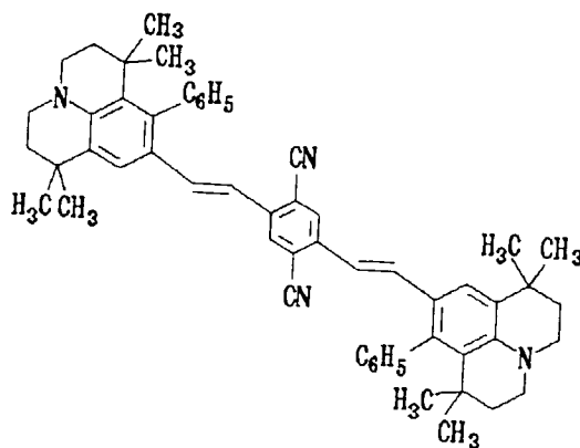
Structural Formula (1)-5:
