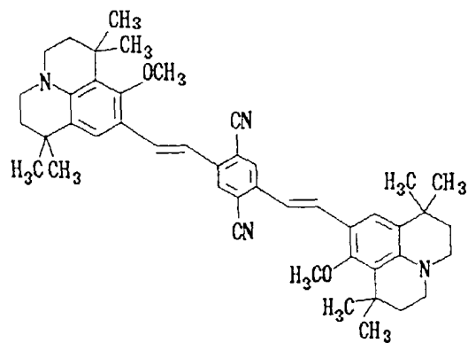
Structural Formula (1) - 1:
