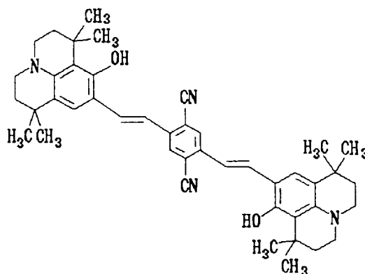
Structural Formula (1) - 6:
