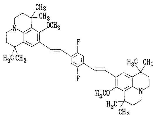
Structural Formula (1) - 7:
