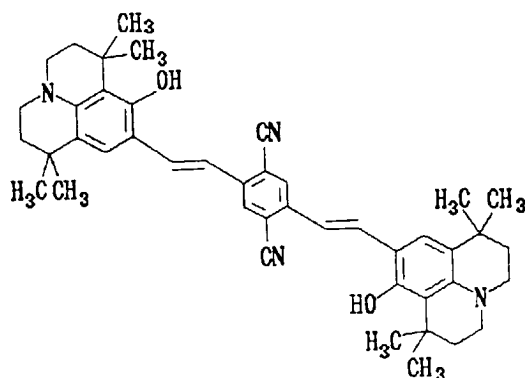
Structural Formula (1) - 6:
