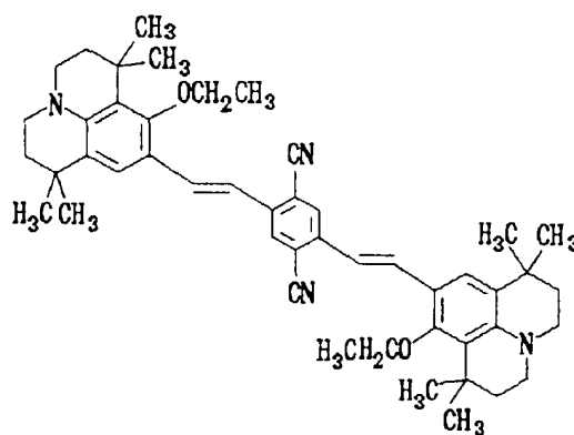
Structural Formula (1) - 2:
