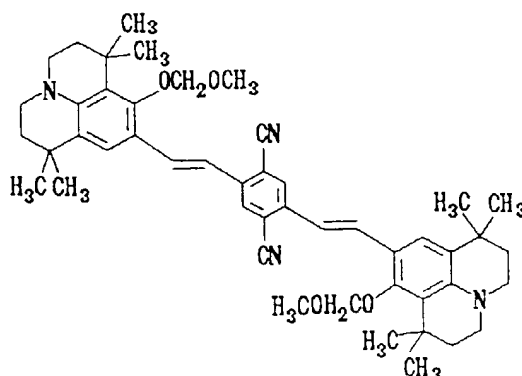
Structural Formula (1) - 8:
