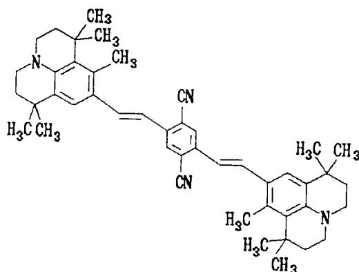
Structural Formula (1)-4:
