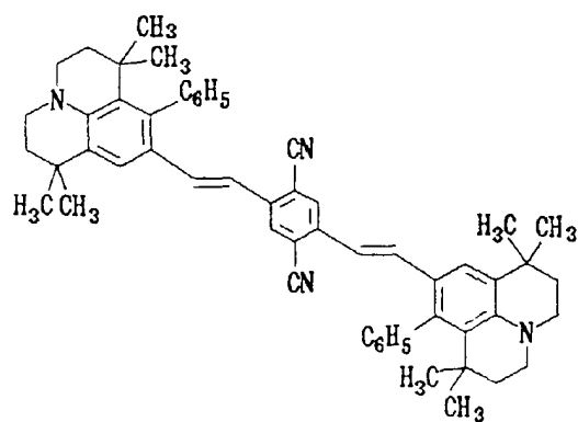
Structural Formula (1) - 5:
