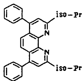
Compound No. 3
