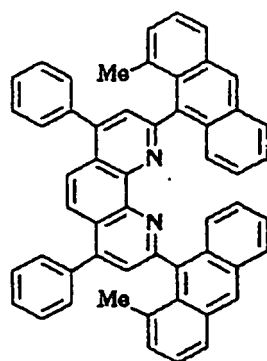
Compound No. 125
