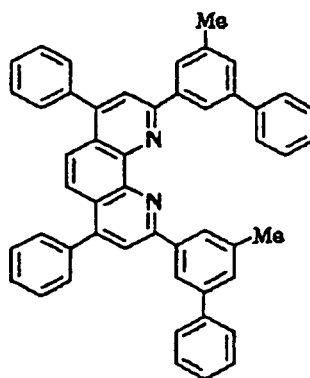
Compound No. 108
