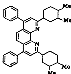
Compound No. 24
