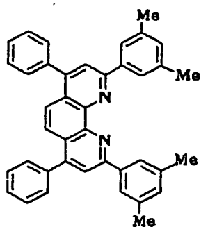
Compound No. 34
