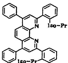
Compound No. 57
