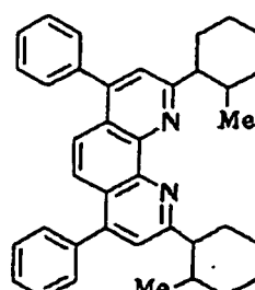
Compound No. 15
