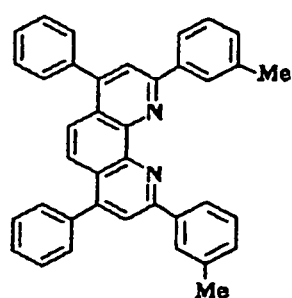
Compound No. 30
