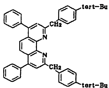
Compound No. 148
