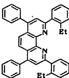
Compound No. 41
