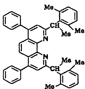
Compound No. 151
