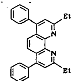
Compound No. 1
