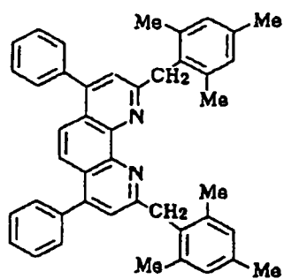
Compound No. 145
