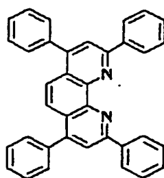
Compound No. 28
