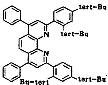
Compound No. 59
