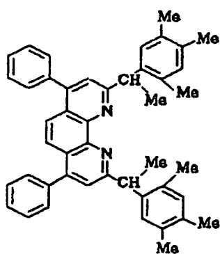
Compound No.155
