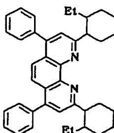
Compound No. 20
