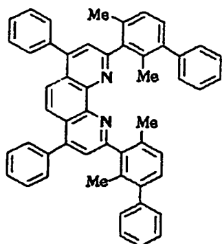
Compound No. 109
