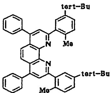
Compound No. 72
