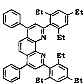
Compound No. 51
