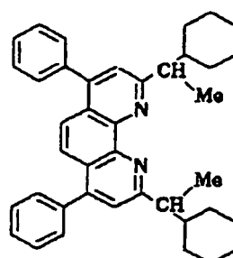
Compound No. 172
