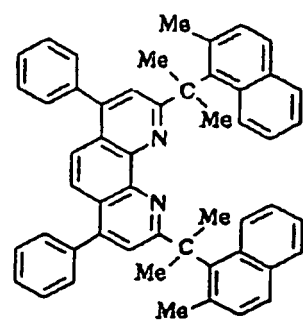
Compound No. 169
