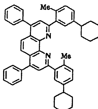
Compound No. 86
