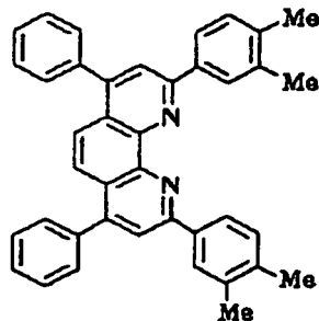
Compound No. 35
