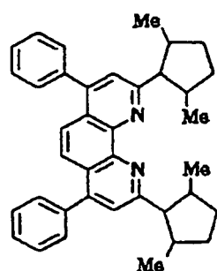
Compound No. 10
