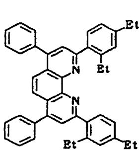
Compound No. 46
