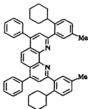
Compound No. 80
