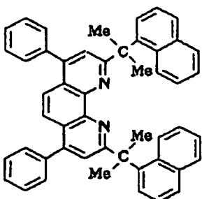
Compound No. 167
