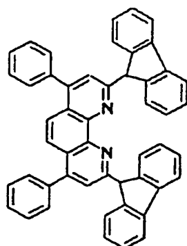
Compound No. 133
