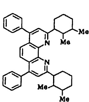
Compound No. 22
