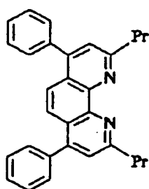
Compound No. 2
