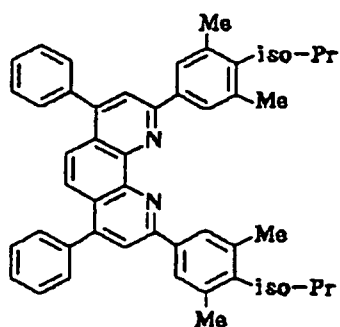
Compound No. 77
