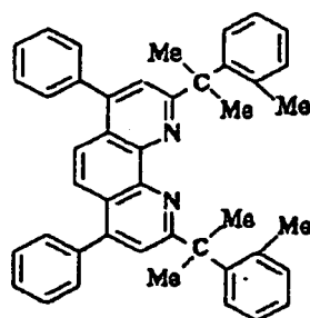
Compound No.156
