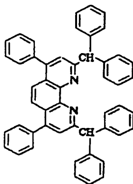
Compound No. 159
