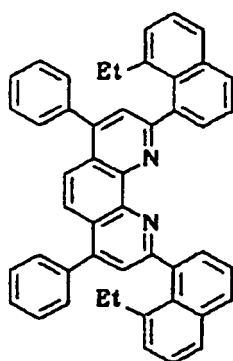
Compound No. 121
