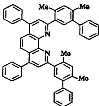
Compound No. 111
