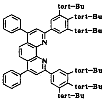
Compound No. 63
