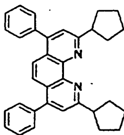
Compound No. 8
