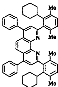
Compound No. 83
