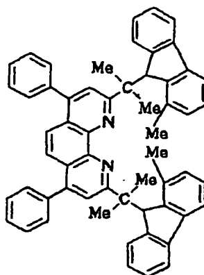
Compound No. 178
