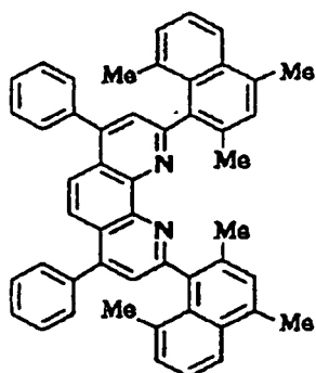
Compound No. 119
