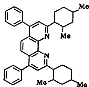
Compound No. 21
