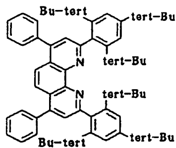
Compound No. 62
