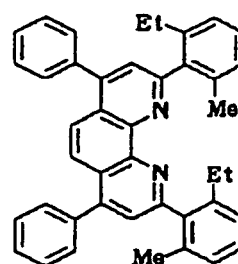
Compound No. 66
