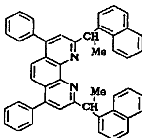
Compound No. 163
