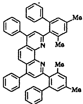
Compound No. 103
