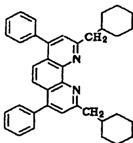
Compound No. 171
