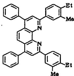
Compound No. 70
