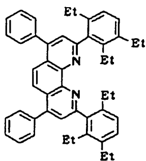
Compound No. 49
