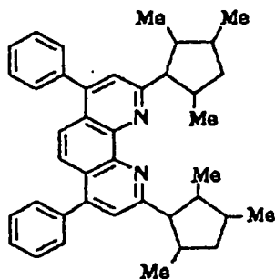
Compound No. 11
