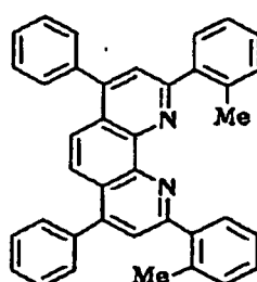
Compound No. 29
