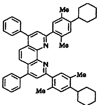
Compound No. 93
