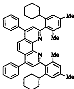
Compound No. 84
