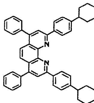
Compound No. 90
