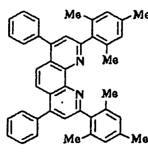
Compound No. 39
