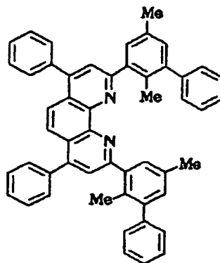
Compound No. 112
