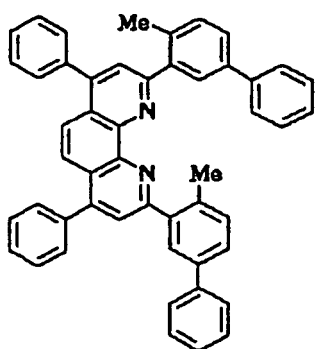
Compound No. 107
