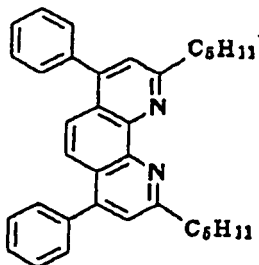
Compound No. 13
