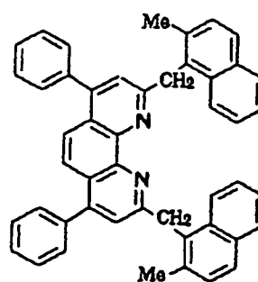
Compound No. 162
