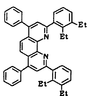
Compound No. 45
