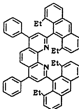
Compound No. 130
