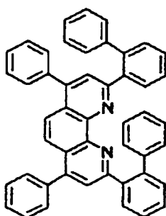
Compound No. 95
