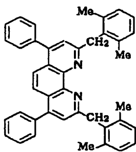
Compound No. 143
