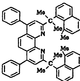
Compound No. 168
