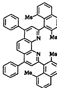
Compound No. 118
