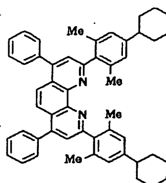
Compound No. 92
