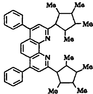
Compound No. 12
