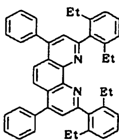
Compound No. 44
