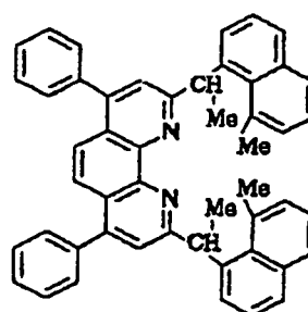
Compound No. 164
