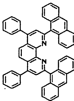
Compound No. 124
