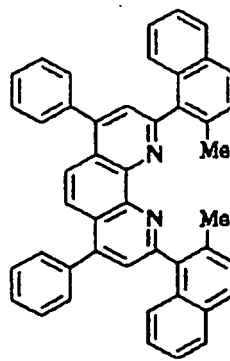
Compound No. 126
