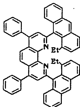
Compound No. 129
