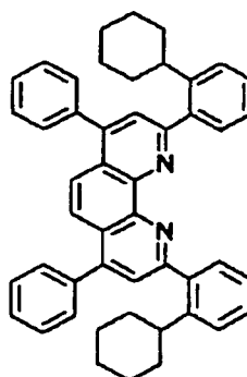
Compound No. 78
