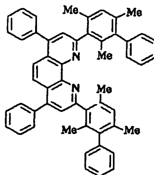
Compound No. 114
