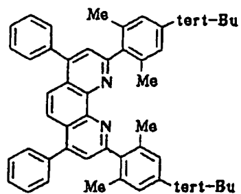
Compound No. 74
