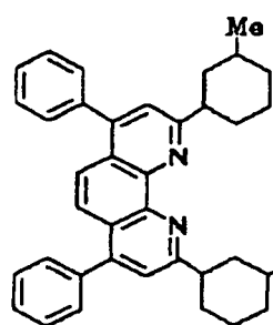
Compound No. 16
