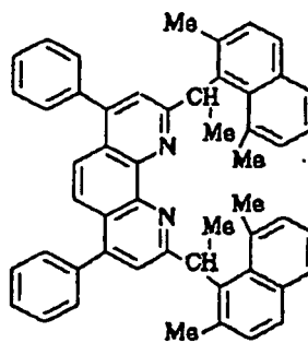
Compound No. 166
