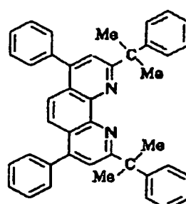
Compound No. 140
