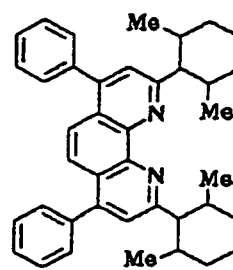
Compound No. 18
