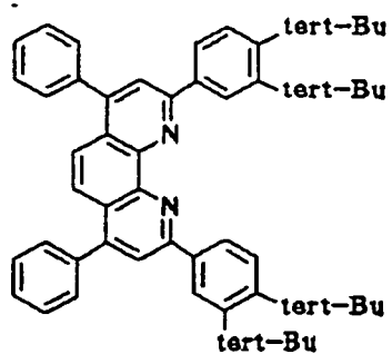
Compound No. 61
