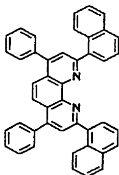
Compound No. 115
