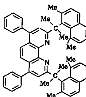
Compound No. 170
