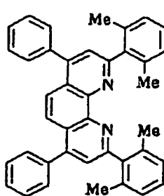
Compound No. 32
