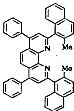
Compound No. 117
