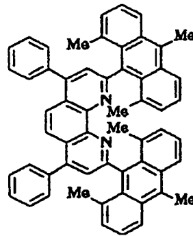
Compound No. 128
