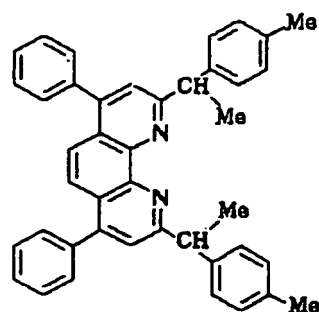
Compound No. 150
