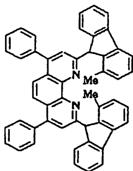
Compound No. 135
