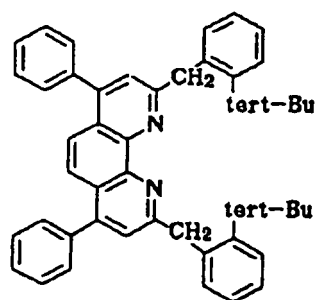
Compound No. 146
