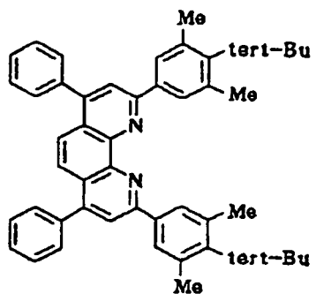
Compound No. 75
