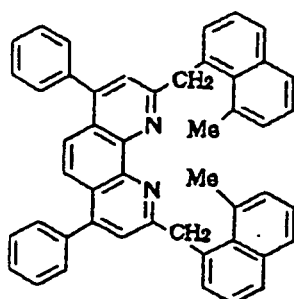
Compound No. 161
