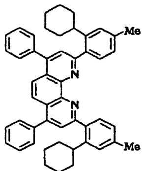
Compound No. 81
