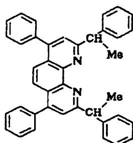
Compound No. 139
