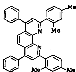
Compound No. 33
