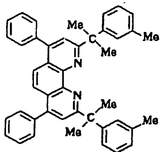
Compound No.157
