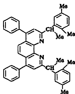
Compound No. 152
