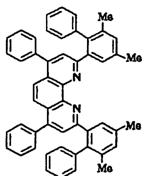
Compound No. 102
