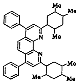
Compound No. 27
