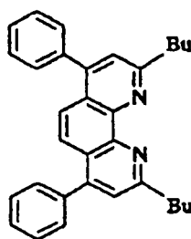
Compound No. 4
