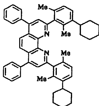
Compound No. 89
