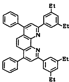
Compound No. 47
