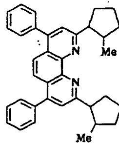
Compound No. 9
