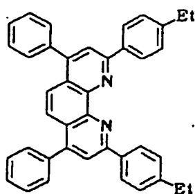
Compound No. 43
