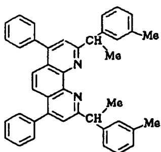
Compound No. 149
