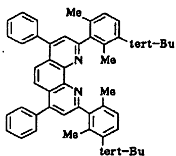
Compound No. 76
