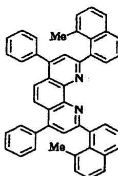
Compound No. 116
