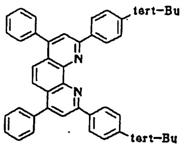
Compound No. 55
