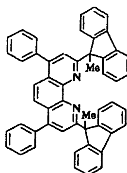
Compound No. 134
