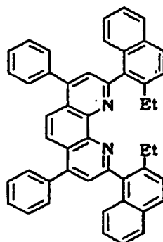
Compound No. 120
