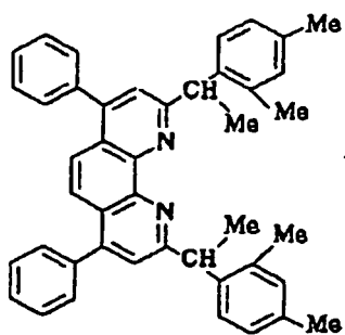
Compound No.153
