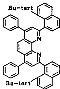
Compound No. 123
