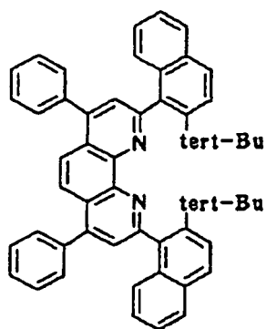
Compound No. 122
