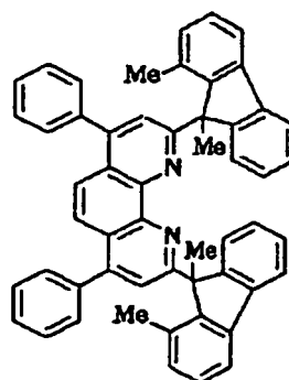
Compound No. 136
