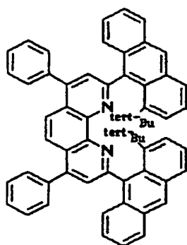
Compound No. 131
