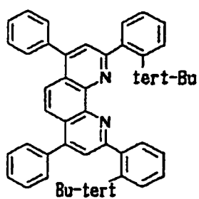
Compound No. 53
