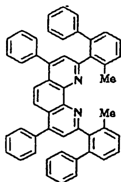
Compound No. 97
