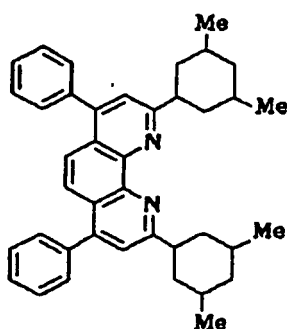
Compound No. 23
