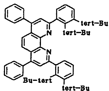
Compound No. 58
