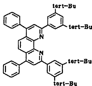
Compound No. 60
