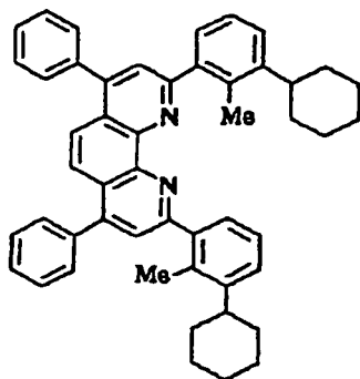
Compound No. 87
