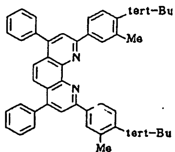
Compound No. 73
