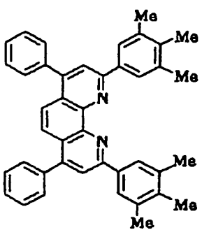
Compound No. 40
