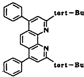
Compound No. 6
