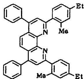
Compound No. 68
