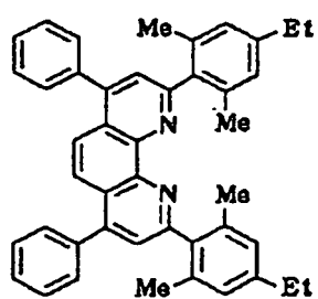
Compound No. 71
