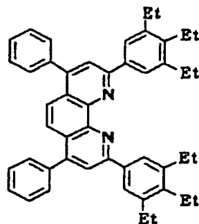
Compound No. 52
