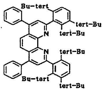
Compound No. 64
