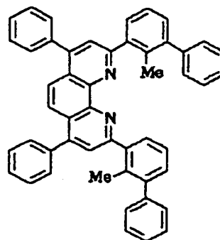
Compound No. 106
