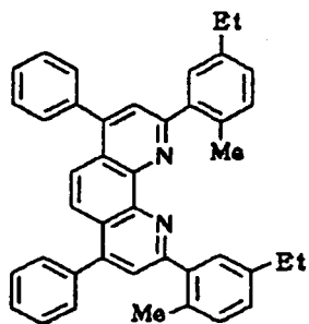
Compound No. 69
