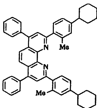
Compound No. 91
