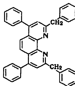
Compound No. 138
