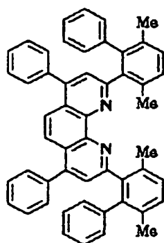
Compound No. 101
