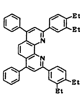
Compound No. 48
