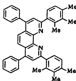
Compound No. 38
