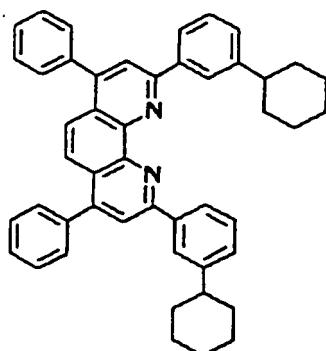
Compound No. 85
