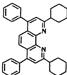
Compound No. 14
