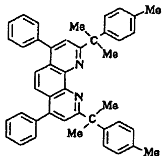
Compound No.158
