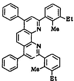
Compound No. 67
