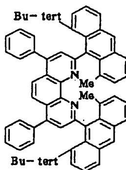
Compound No. 132
