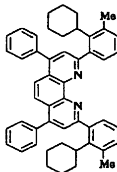
Compound No. 82
