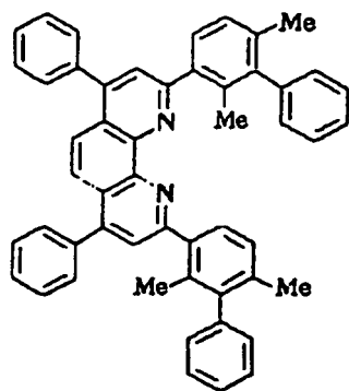
Compound No. 113
