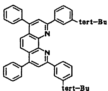
Compound No. 54
