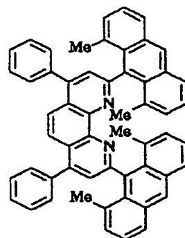
Compound No. 127
