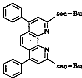
Compound No. 5
