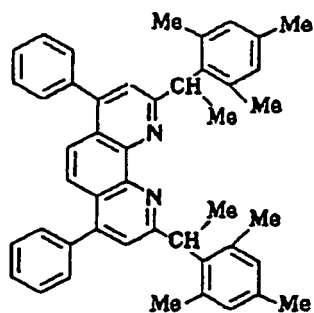
Compound No.154
