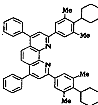
Compound No. 94
