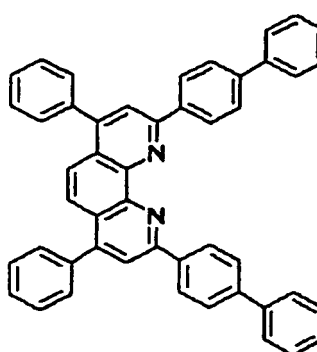
Compound No. 96
