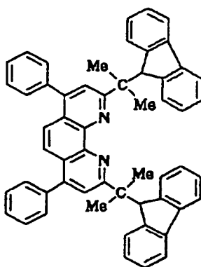
Compound No. 175
