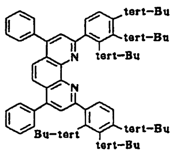
Compound No. 65
