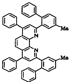
Compound No. 99
