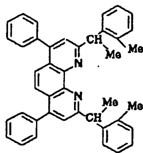
Compound No. 142
