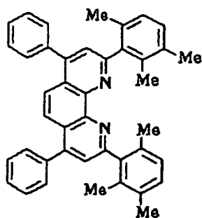
Compound No. 37
