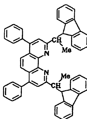
Compound No. 174
