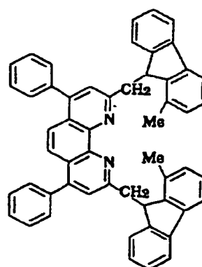
Compound No. 176
