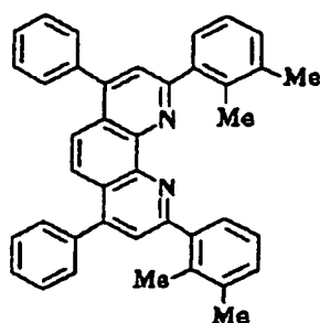
Compound No. 36
