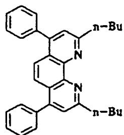
Compound No. 7
