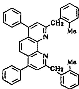
Compound No. 141
