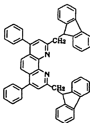
Compound No. 173
