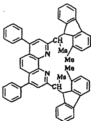
Compound No. 177
