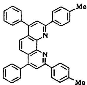
Compound No. 31
