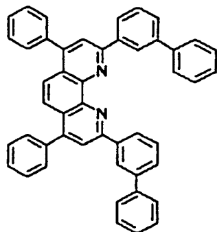
Compound No. 105
