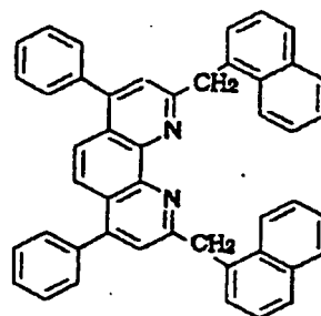
Compound No. 160
