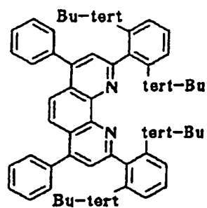
Compound No. 56
