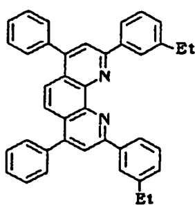
Compound No. 42
