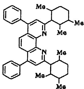
Compound No. 25
