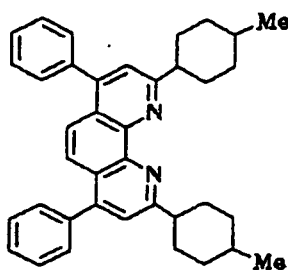
Compound No. 17
