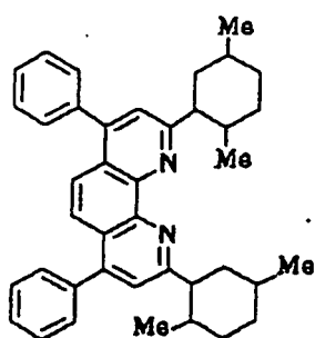
Compound No. 19
