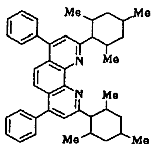
Compound No. 26
