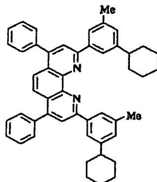
Compound No. 88
