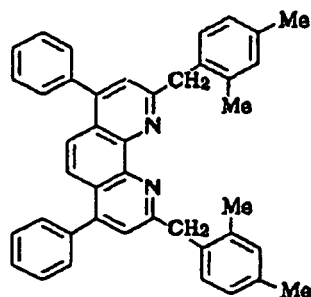
Compound No. 144
