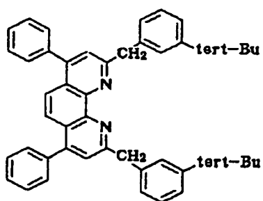
Compound No. 147
