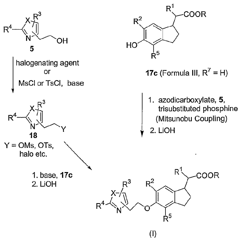
Reaction Scheme 3
