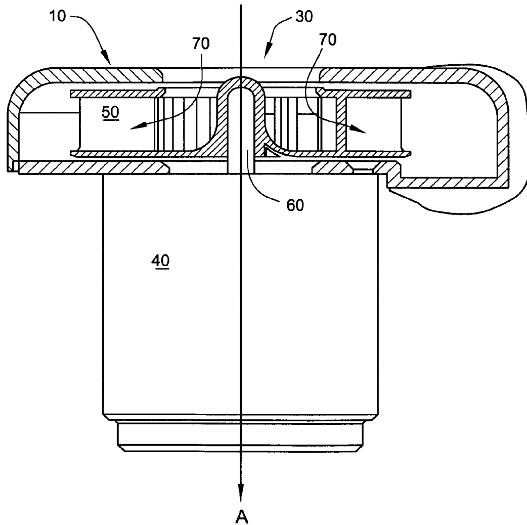
FIG. 2 (PRIOR ART)
