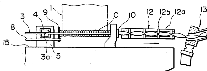
FIG. 2 PRIOR ART
