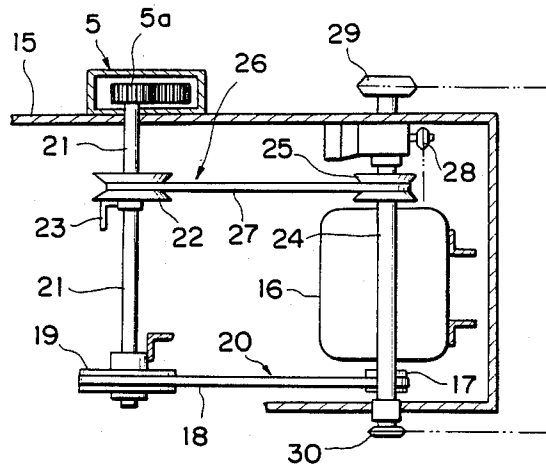
FIG. 4 PRIOR ART
