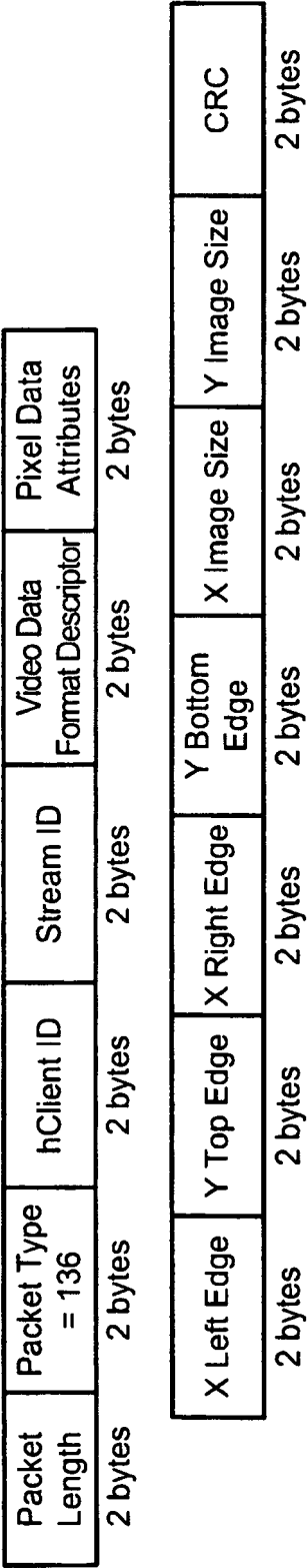
Scaled Video Stream Setup Packet
